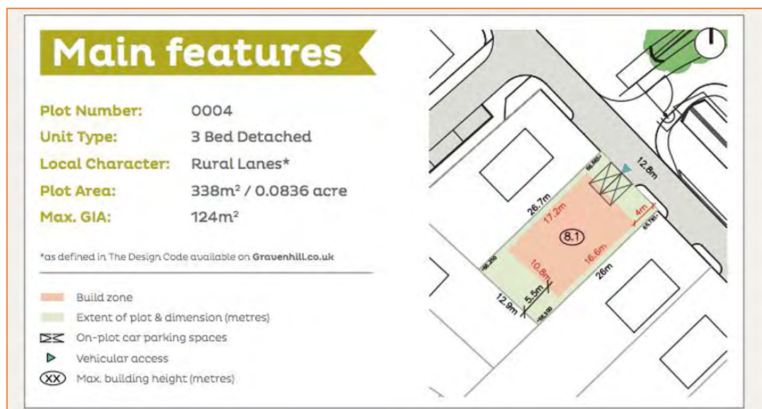
Figure 9: Example extract from a site regulating plan and associated plot passport 21
