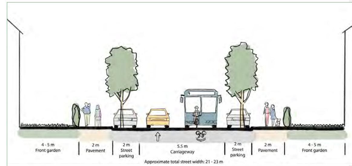
Figure 59: Cross section of 'central street' typology
