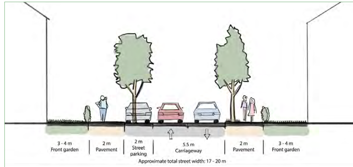
Figure 60: Cross section of 'residential street' typology
