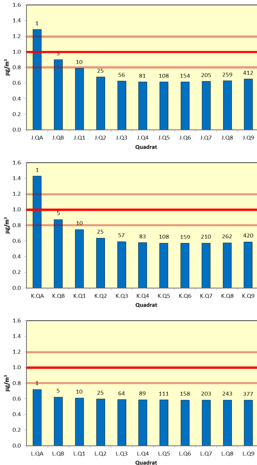
Figure 9.14: Annual Mean \text{NH}_3 Concentrations Along Transects J, K, and L. Approximate distance from the nearest main road to each quadrat to shown numerically above each column. Lines show the 1 \mu\text{g}/\text{m}^3 critical level and the \pm 20\% critical level range suggested by CEH.
