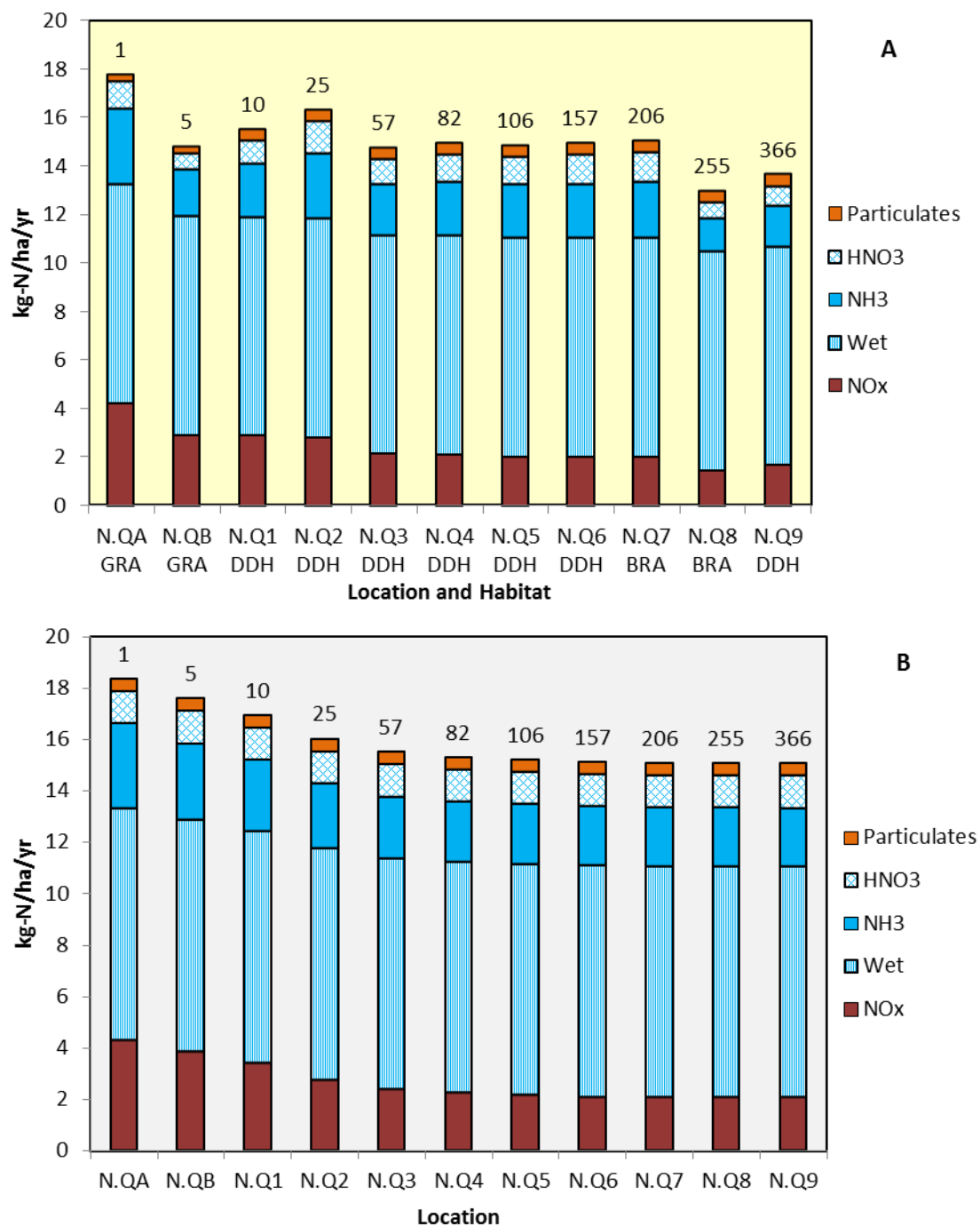
Figure 9.29: Deposition to Ecological Transect N – EA Method – A Using Current Habitat Types and B If all Habitat were Heath (approximate distance from the nearest main road to each quadrant to shown numerically above each column) 36
