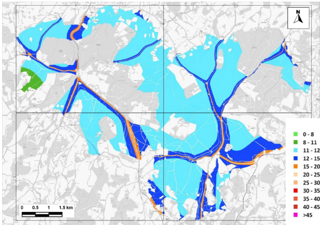
Figure 9.46: Predicted Annual Mean NOx Concentrations across the SAC – Existing Baseline ( \mu\text{g}/\text{m}^3 )
