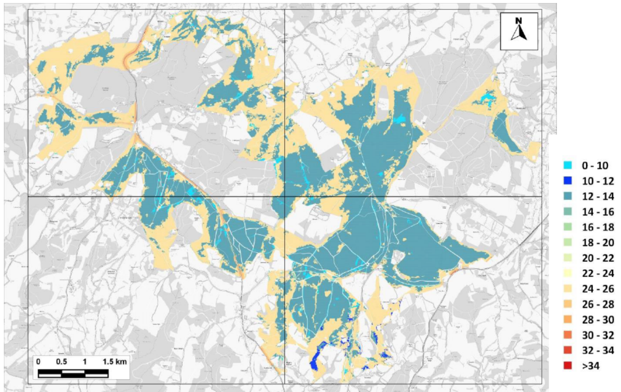
Figure 11.13: Nitrogen Deposition to SAC – 2028 No WDC-Growth - C (AQC Method) (kg-N/ha/yr)
