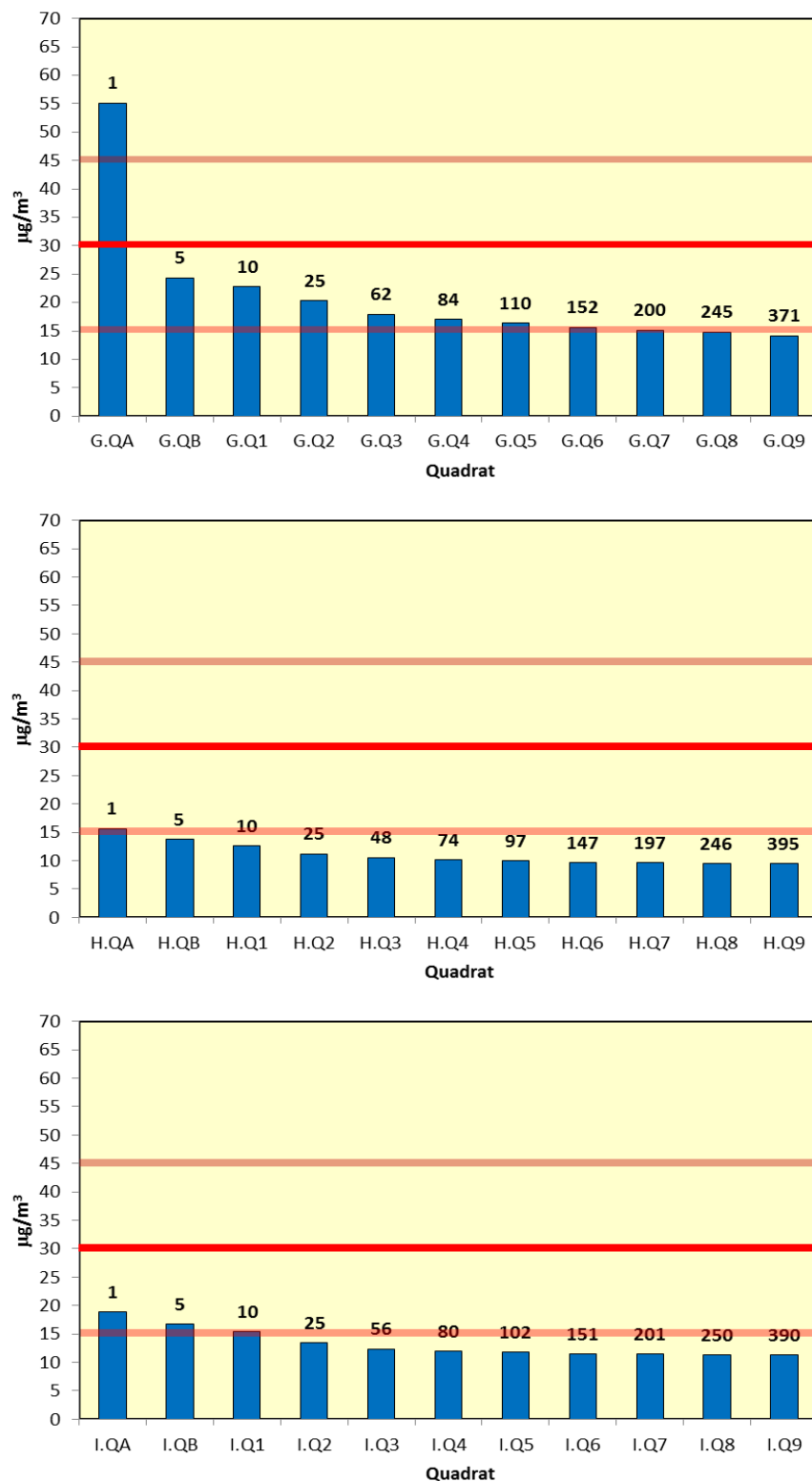
Figure 9.3: Annual Mean NO x Concentrations Along Transects G, H, and I. Approximate distance from the nearest main road to each quadrant to shown numerically above each column. Lines show the 30 µg/m 3 critical level and the 15 µg/m 3 and 45 µg/m 3 critical level range suggested by CEH.
