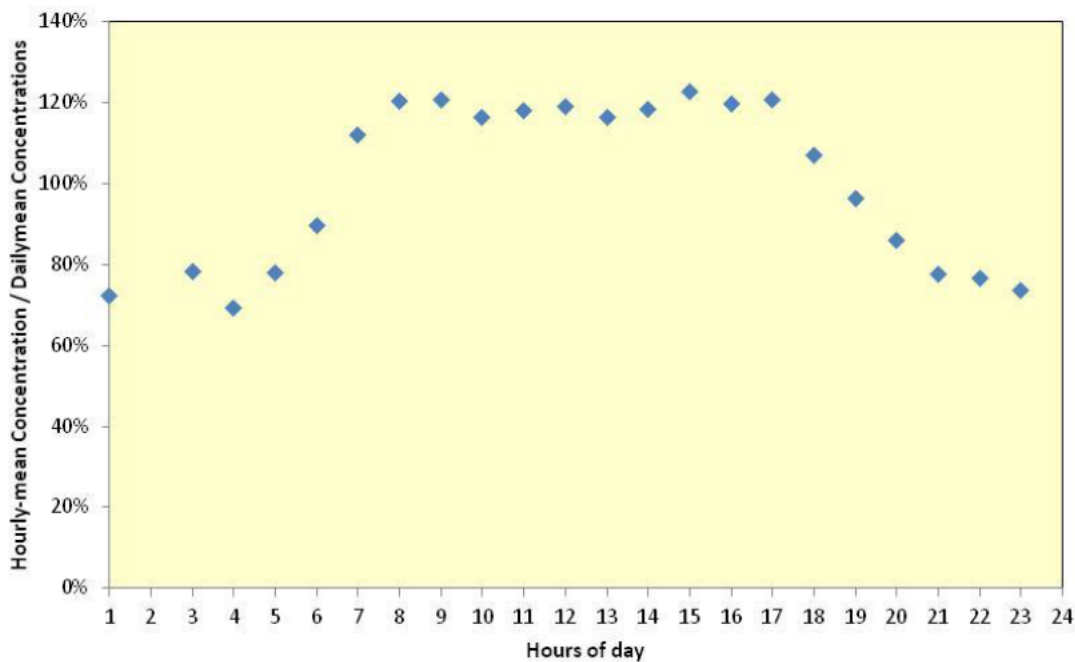
Figure 8.6: Ammonia Hourly-mean NH 3 / Average Daily-mean NH 3 between October 2014 and August 2016 (GMT) 31
