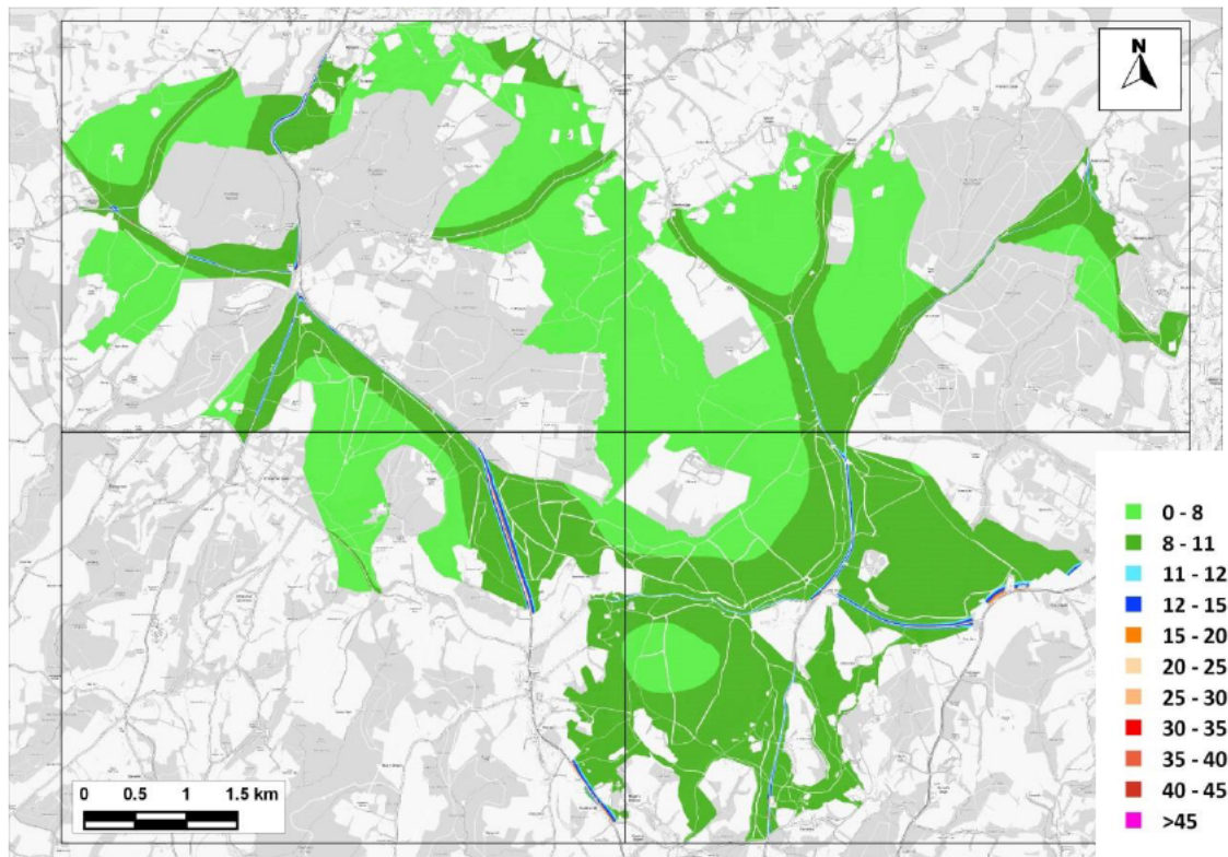
Figure 10.1: Predicted Annual Mean NO x Concentrations across the SAC– 2028 No-Growth - B ( \mu\text{g}/\text{m}^3 )
