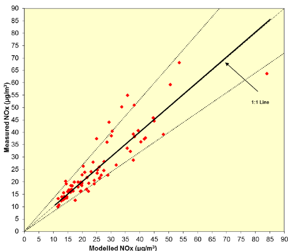
Figure 5.23: Modelled vs Measured Total Annual Mean NO x Concentrations following All Adjustments
