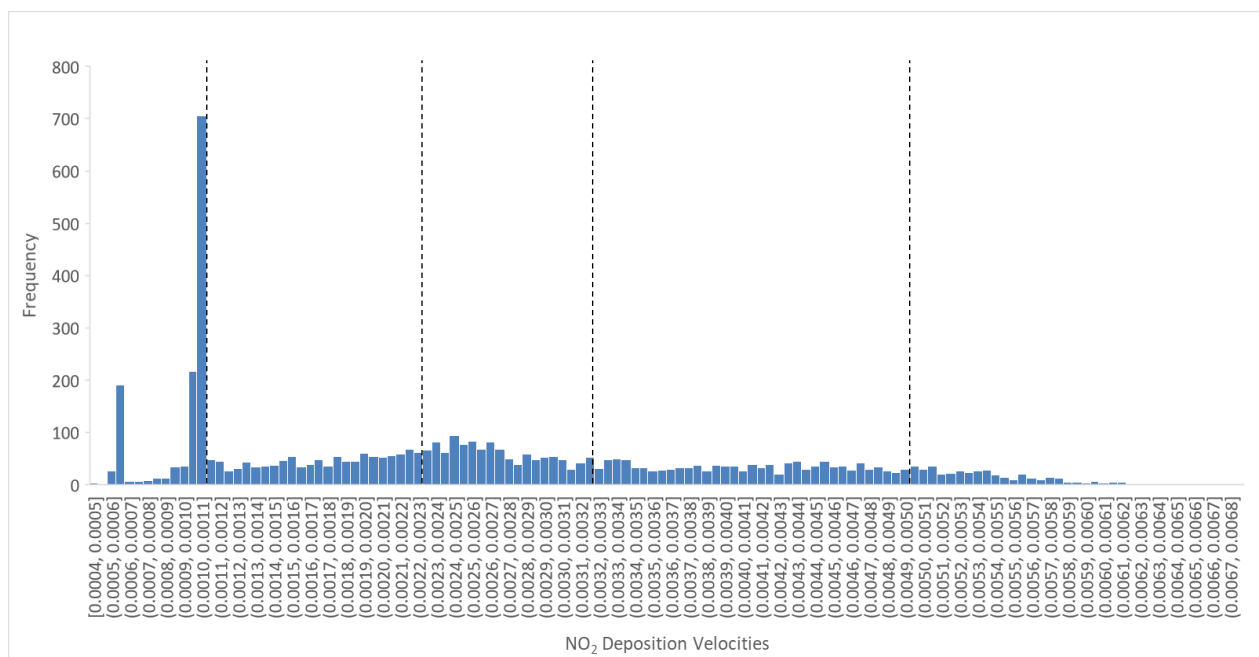
Figure 5.41: Frequency of Summer Daytime Hourly Values of V_d \text{NO}_2 to Heath
