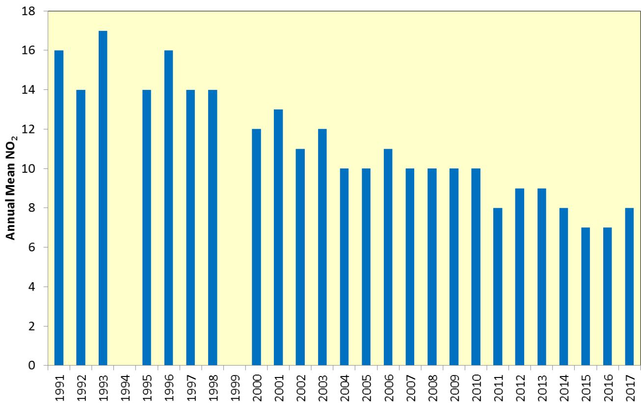
Figure 3.1: Measured Annual Mean NO 2 Concentrations at Lullington Heath over 27 Years (µg/m 3 )
