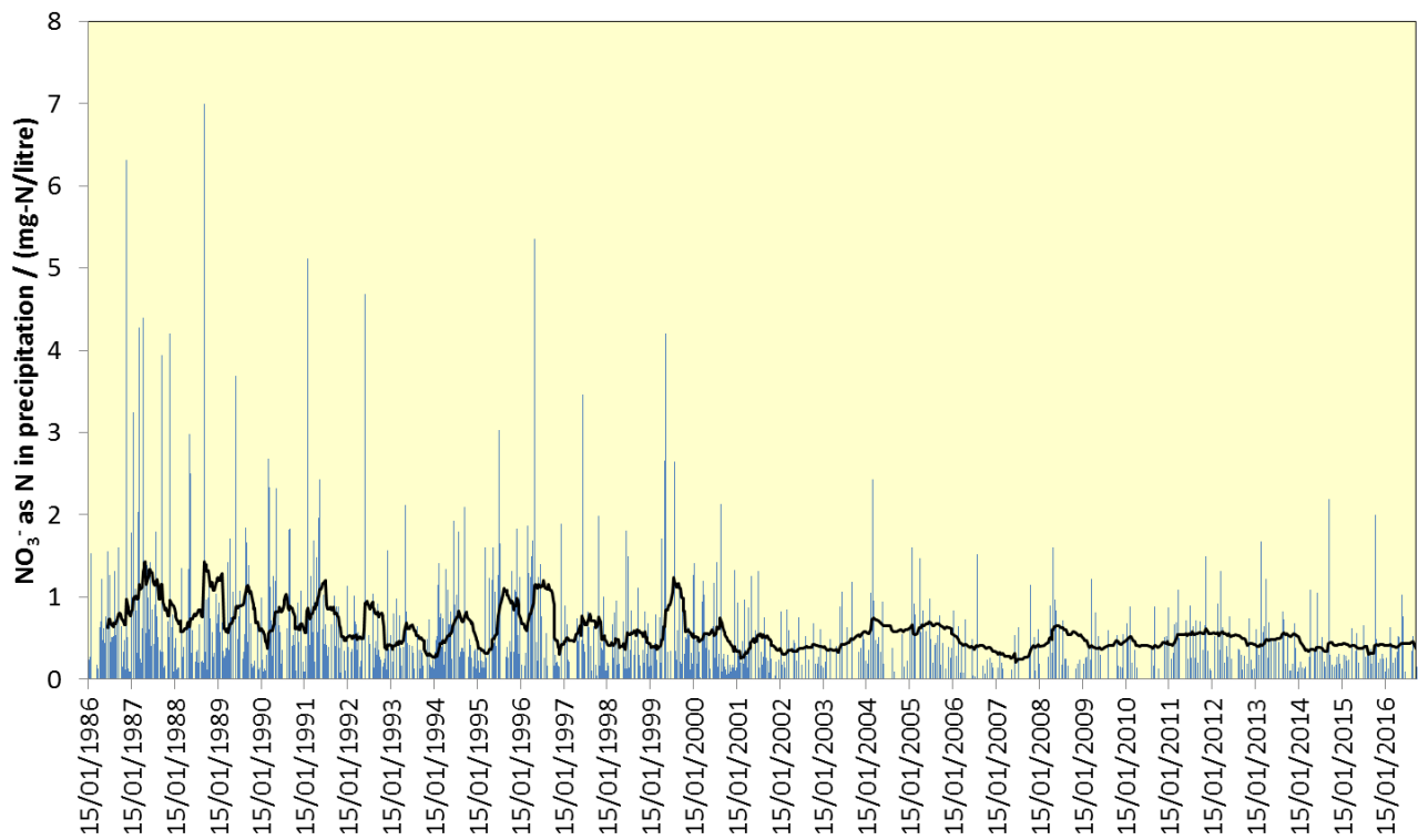
Figure 3.4: \text{NO}_3^- in Precipitation Measured at Barcombe Mills from 1986-2016 (blue line) and 24-month rolling average (black line) (mg-N/litre)
