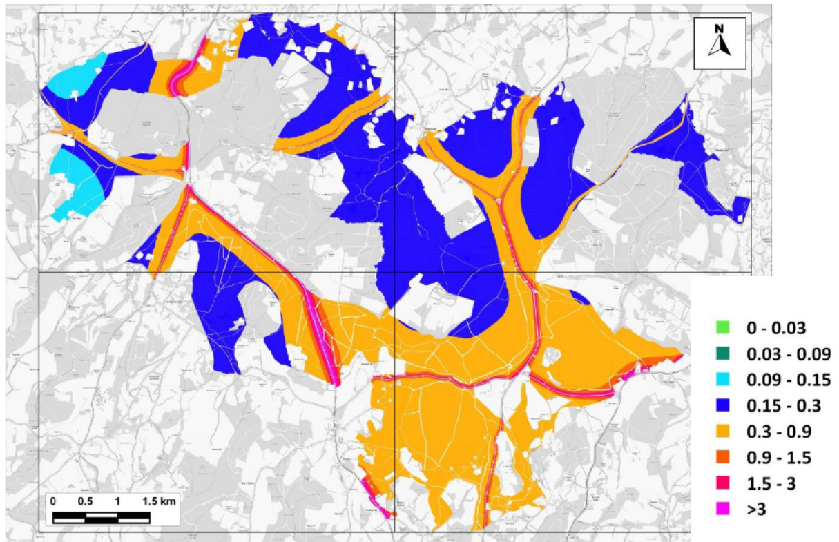
Figure 14.1: Change in Predicted Annual Mean NO x Comparing 'With Plan' to 'No Growth' Under Emissions Scenario A ( \mu\text{g}/\text{m}^3 )
