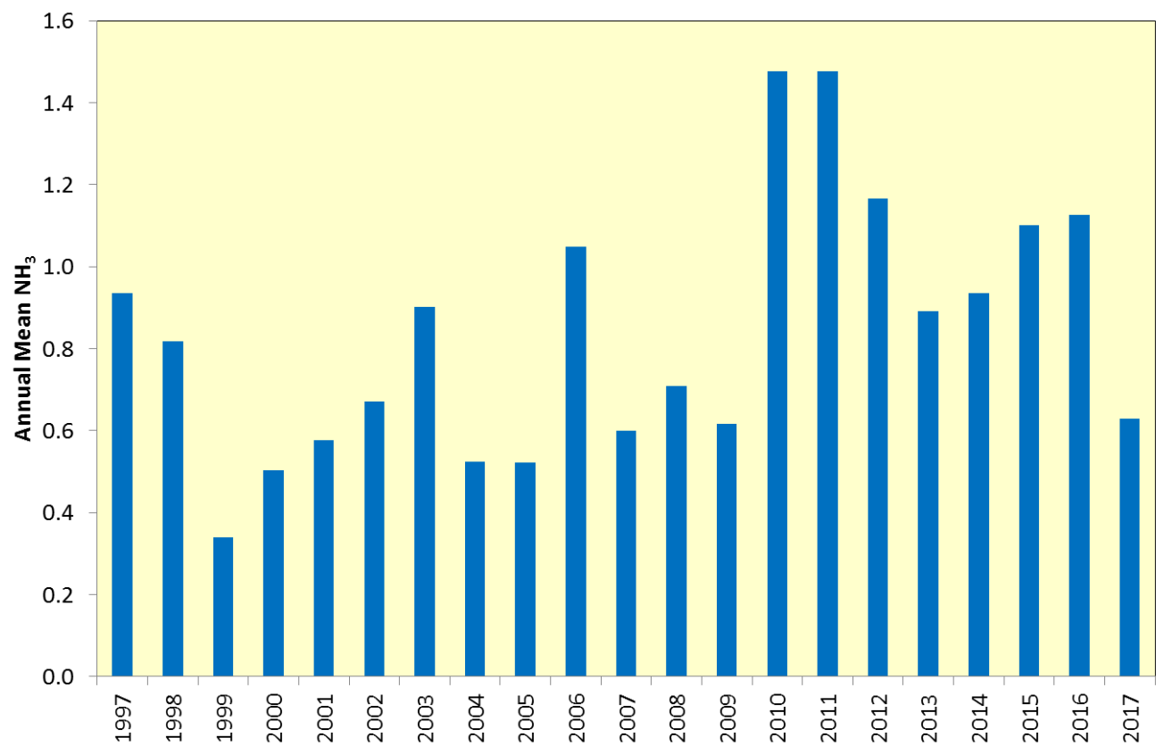
Figure 3.2: Measured Annual Mean NH 3 Concentrations at Lullington Heath over 21 Years (µg/m 3 )
