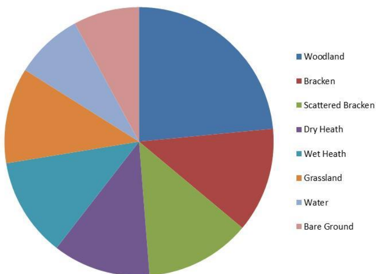
Figure 9.50: Average Nitrogen Deposition to Different Ashdown Forest SAC Land Surfaces (EA Method) – Relative Flux per Ha
