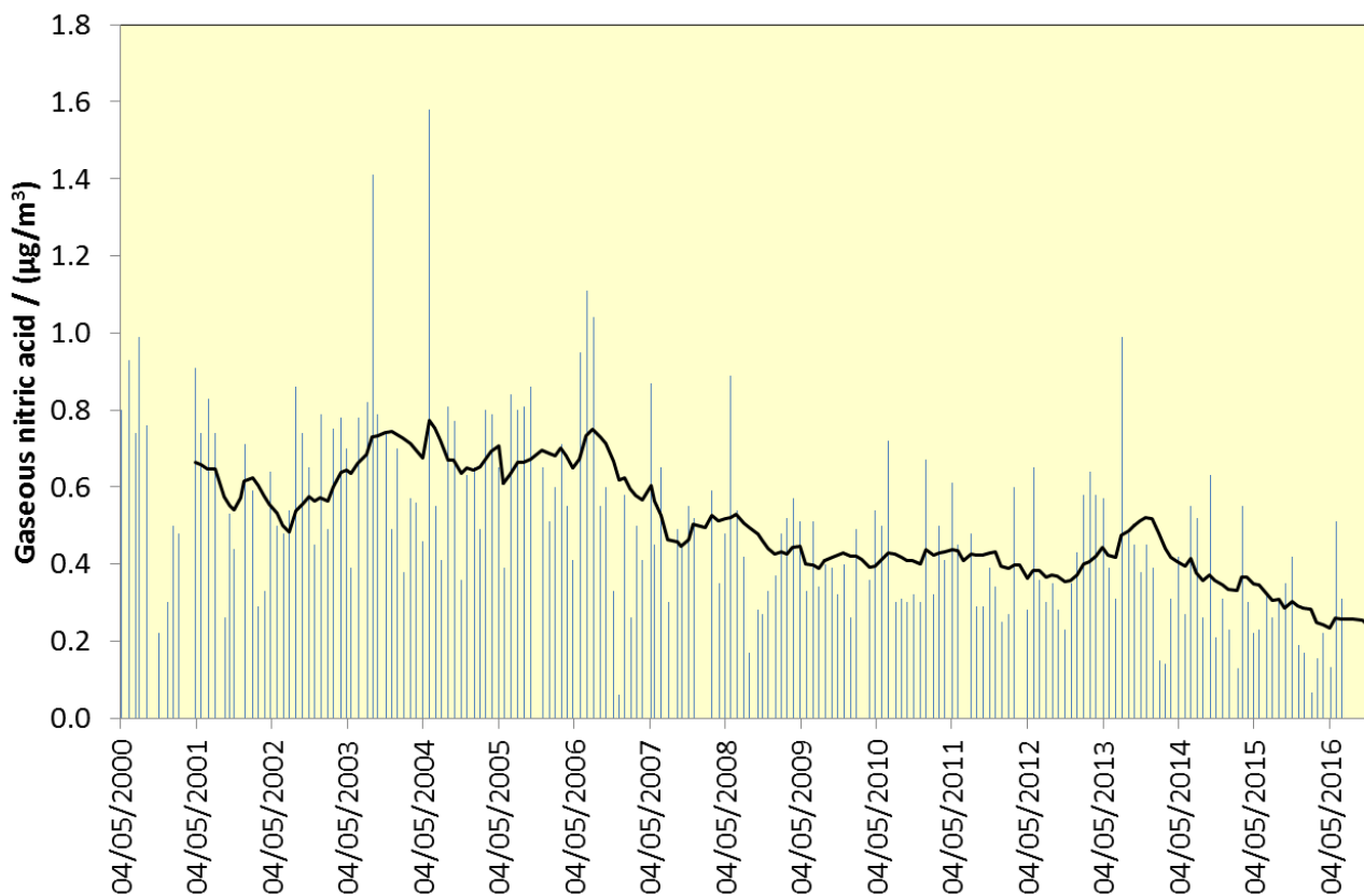
Figure 3.5: Gaseous Nitric Acid Measured at Barcombe Mills from 2000-2016 (blue line) and 24-month rolling average (black line) ( \mu\text{g}/\text{m}^3 )
