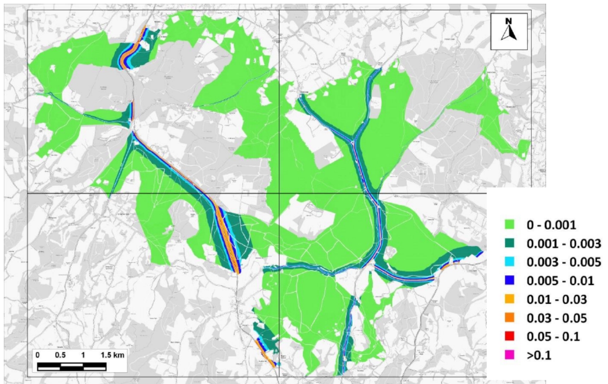
Figure 13.5: Change in Predicted Annual Mean \text{NH}_3 Comparing 'With Plan' to 'No WDC-Growth' ( \mu\text{g}/\text{m}^3 )
