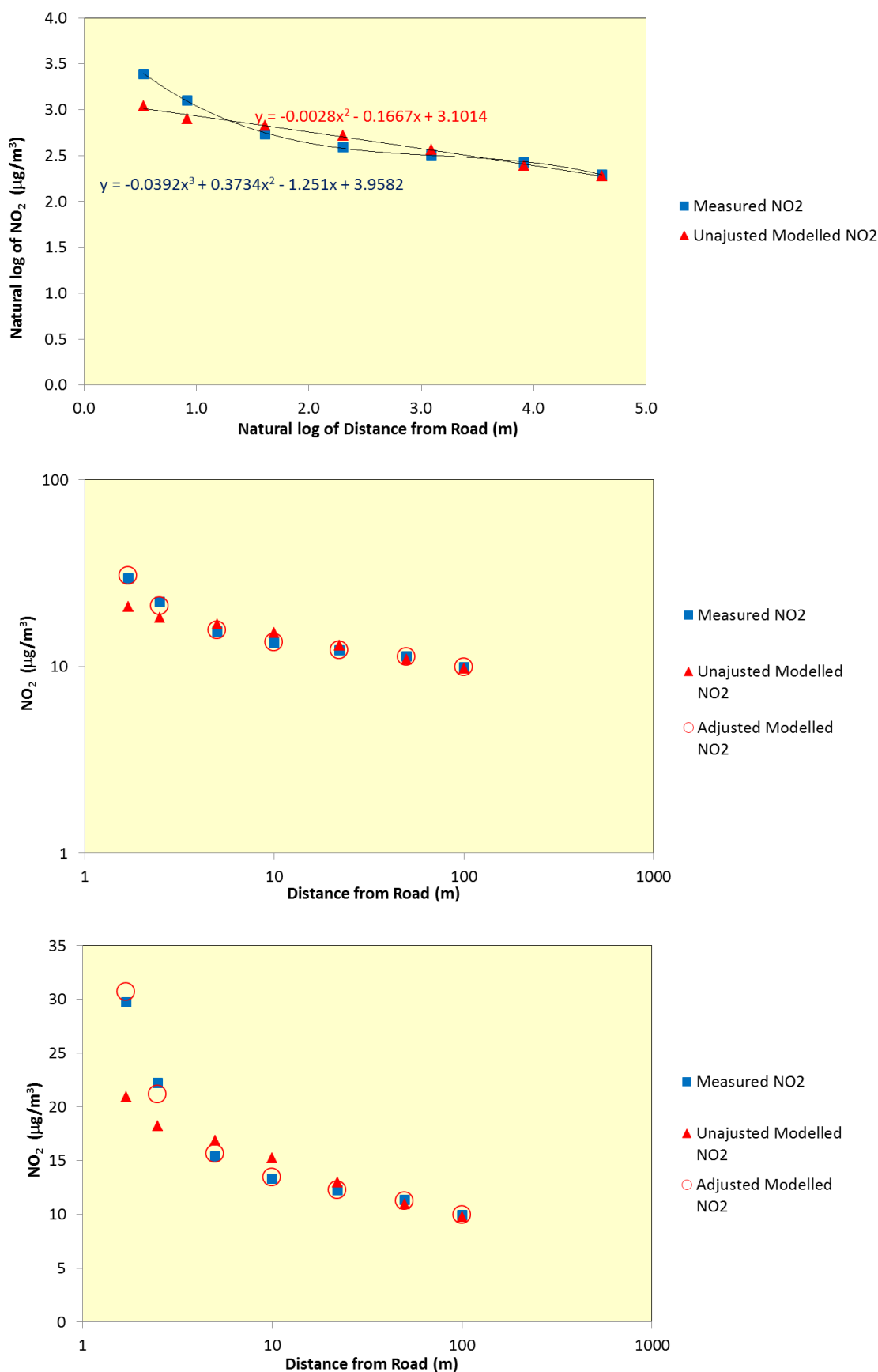
Figure 5.30: Measured vs Predicted 2-Year Average NO 2 Concentrations along Transect 1: top = unadjusted model on log scales, middle = unadjusted and adjusted models on log 'y' scale; bottom = unadjusted and adjusted models.
