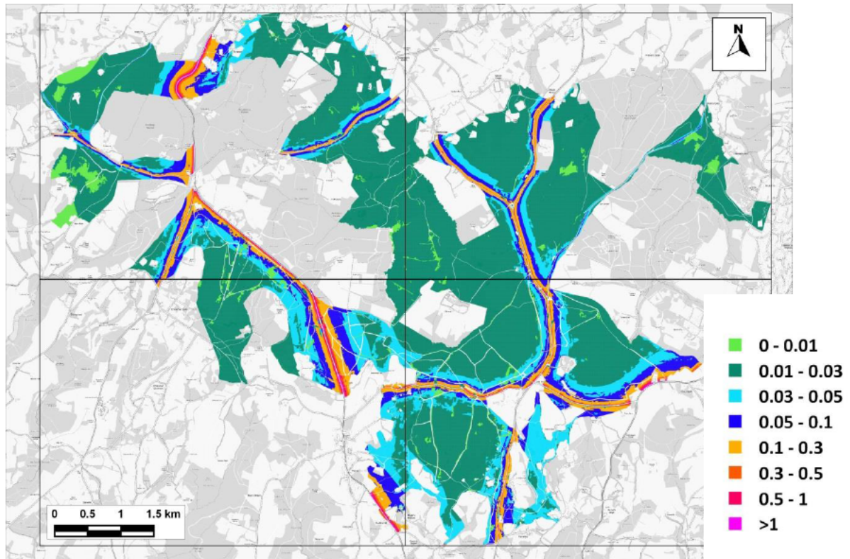
Figure 14.23: Change in Predicted Nitrogen Deposition to SAC Comparing 'With Plan' to 'No Growth' Scenarios Under Emission Scenario C (EA Method) (kg-N/ha/yr)
