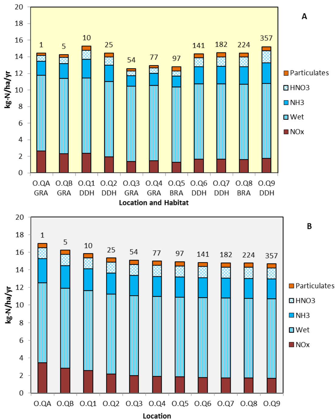
Figure 9.30: Deposition to Ecological Transect O – EA Method – A Using Current Habitat Types and B If all Habitat were Heath (approximate distance from the nearest main road to each quadrant to shown numerically above each column) 36
