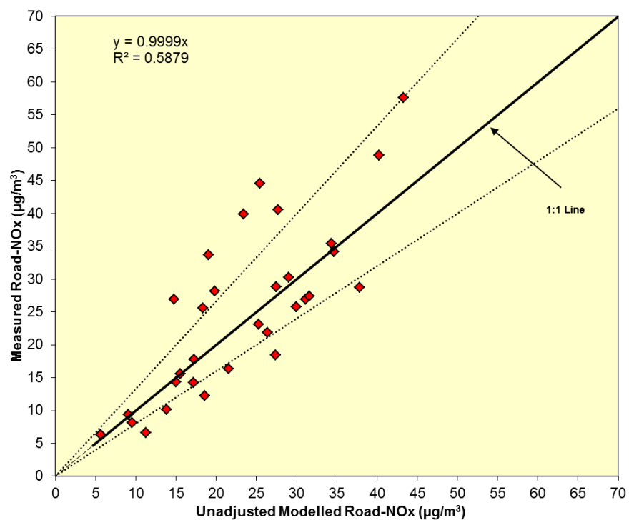
Figure 5.17: Modelled vs Measured Annual Mean Road-NOx, Link Set 1, Iteration 5
