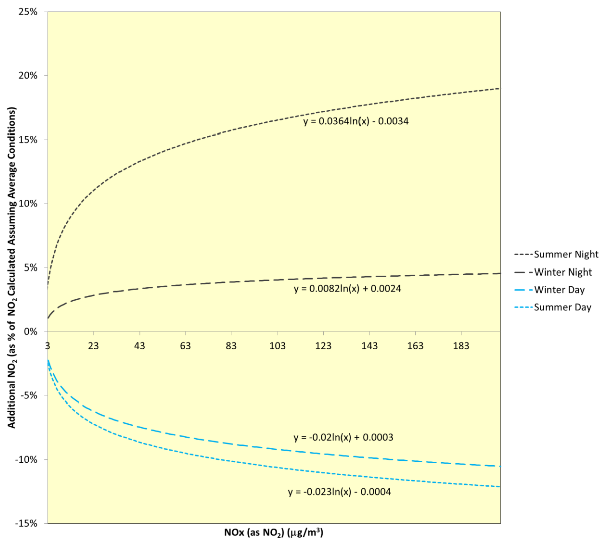
Figure 5.28: Period-specific Uplifts Applied to NO 2 Concentrations Calculated using Defra's NO x to NO 2 Calculator (four periods)
