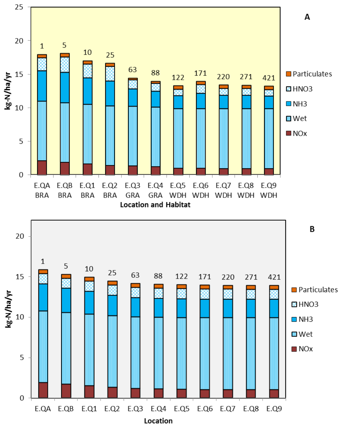
Figure 9.35: Deposition to Ecological Transect E – AQC Method – (A) Using Current Habitat Types and (B) If all Habitat were Heath (approximate distance from the nearest main road to each quadrant to shown numerically above each column) 36
