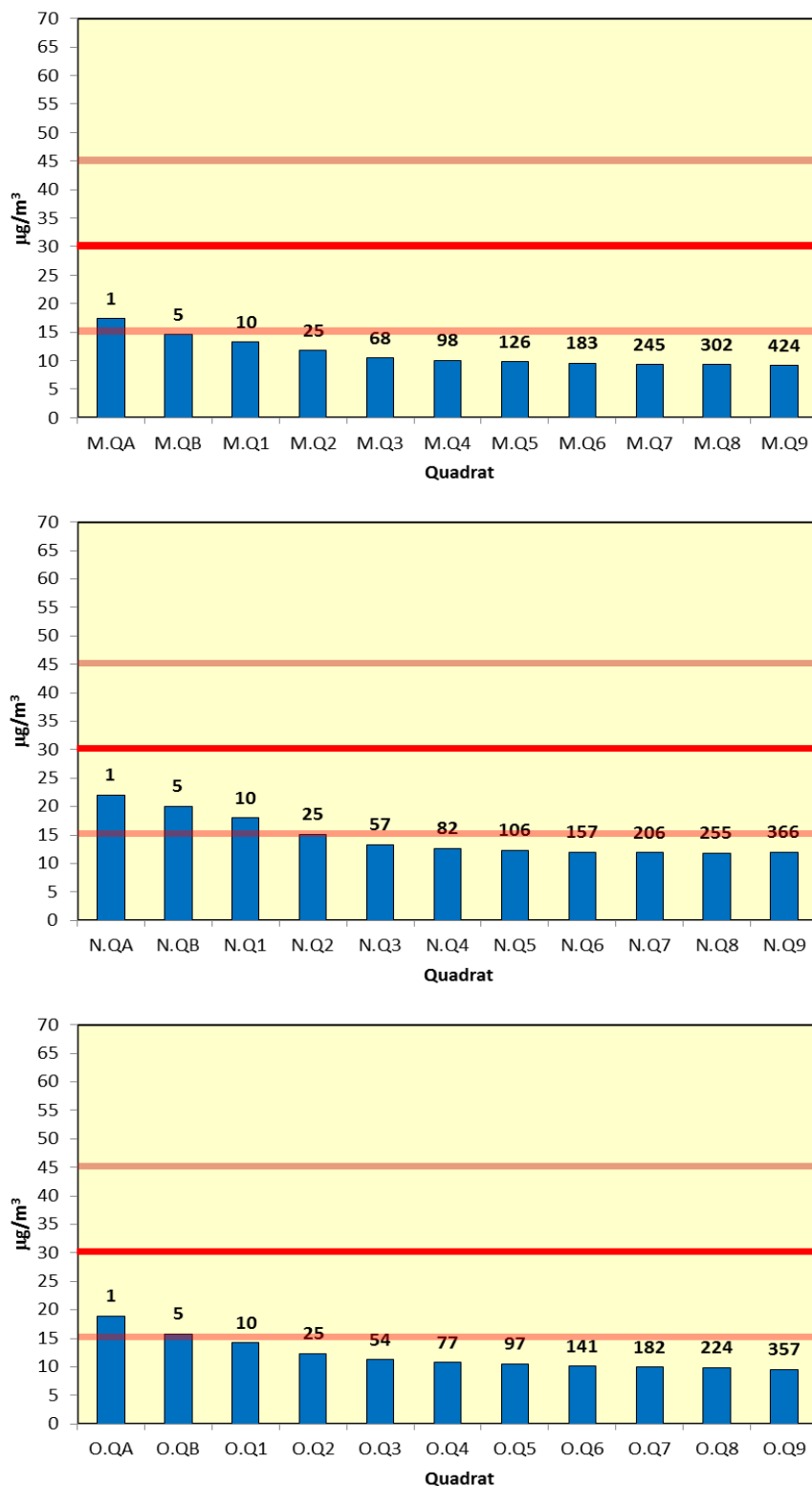
Figure 9.5: Annual Mean NO x Concentrations Along Transects M, N, and O. Approximate distance from the nearest main road to each quadrant to shown numerically above each column. Lines show the 30 µg/m 3 critical level and the 15 µg/m 3 and 45 µg/m 3 critical level range suggested by CEH.
