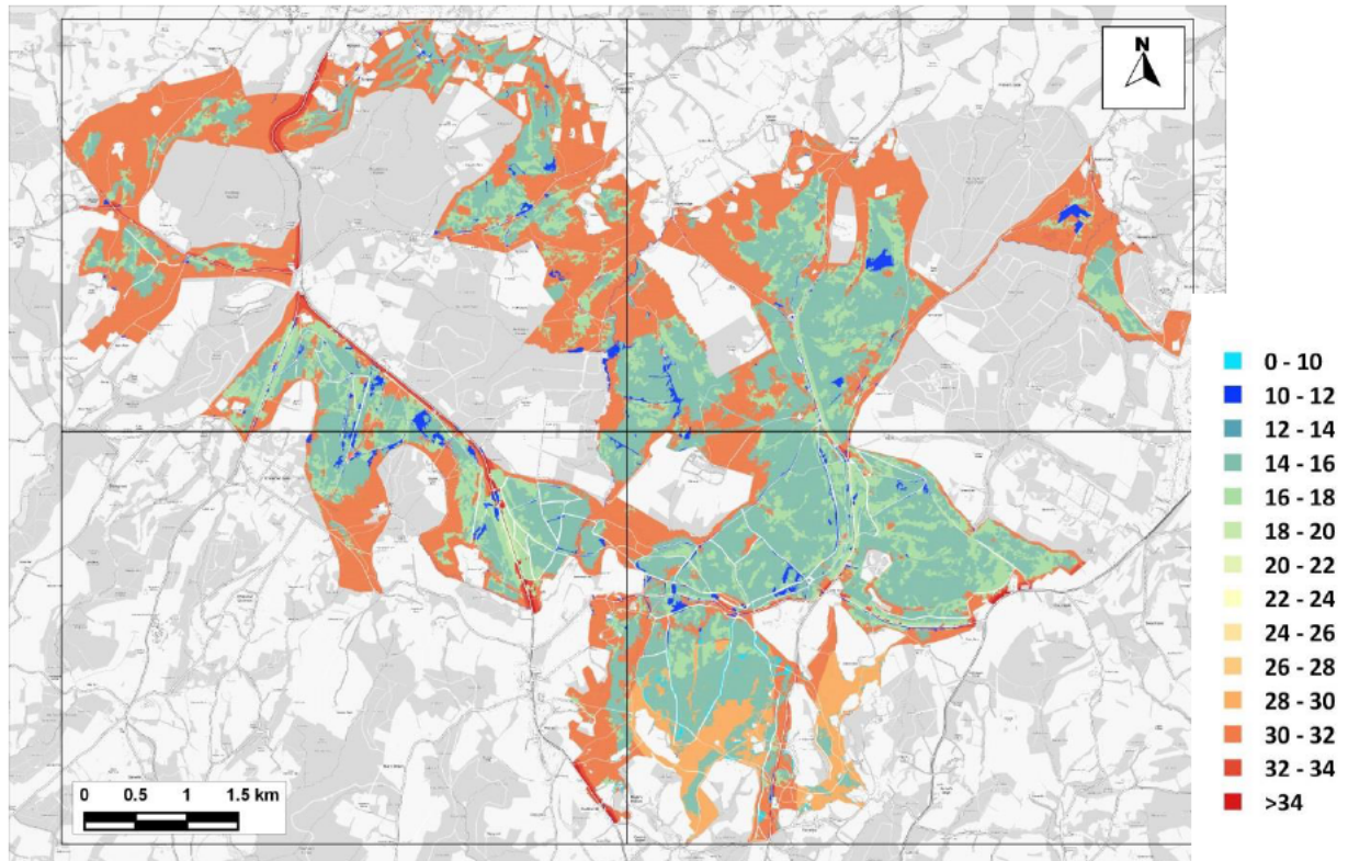
Figure 12.4: Nitrogen Deposition to SAC – 2028 With Plan - A (EA Method) (kg-N/ha/yr)
