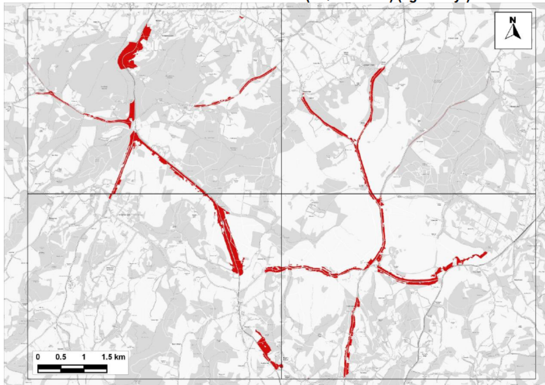
Figure 14.26: Areas in SAC Predicted to Experience an Increase in Nitrogen Deposition Greater than 1% of the 10 kg-N/ha/yr Critical Load where this Critical Load would also be Exceeded - Comparing 'With Plan' to 'No Growth' Scenarios under Emissions Scenario C (AQC Method)
