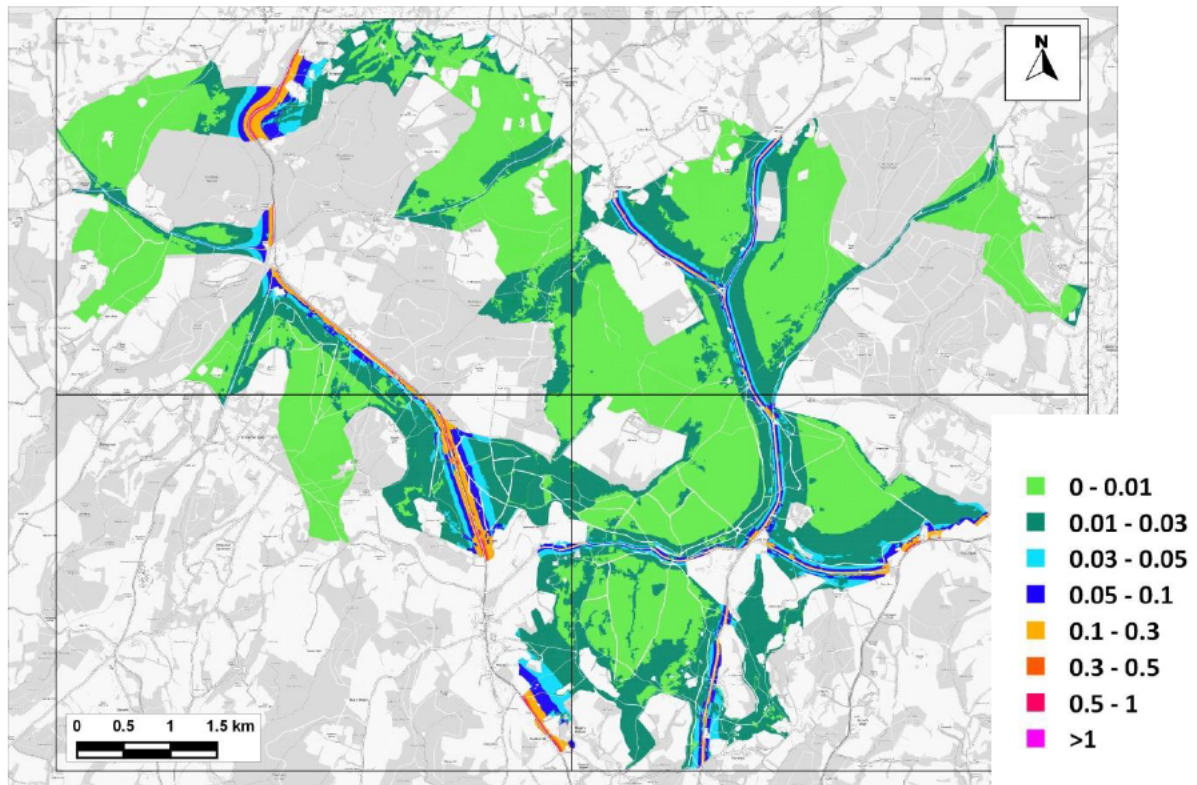
Figure 13.9: Change in Predicted Nitrogen Deposition to SAC Comparing 'With Plan' to 'No WDC-Growth' under Emissions Scenario A (AQC Method) (kg-N/ha/yr)
