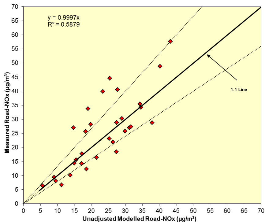
Figure 5.14: Modelled vs Measured Annual Mean Road-NOx, Link Set 1, Iteration 4
