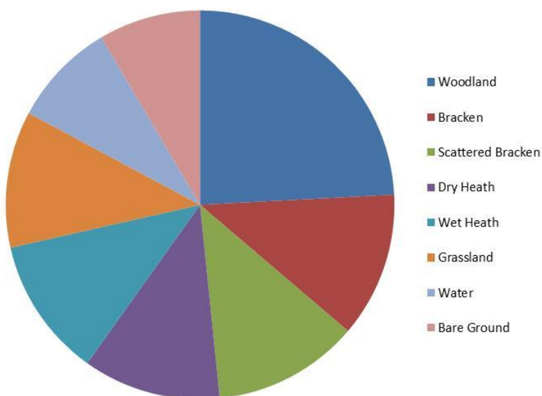
Figure 9.54: Average Nitrogen Deposition to Different Ashdown Forest SAC Land Surfaces (AQC Method) – Relative Flux per Ha
