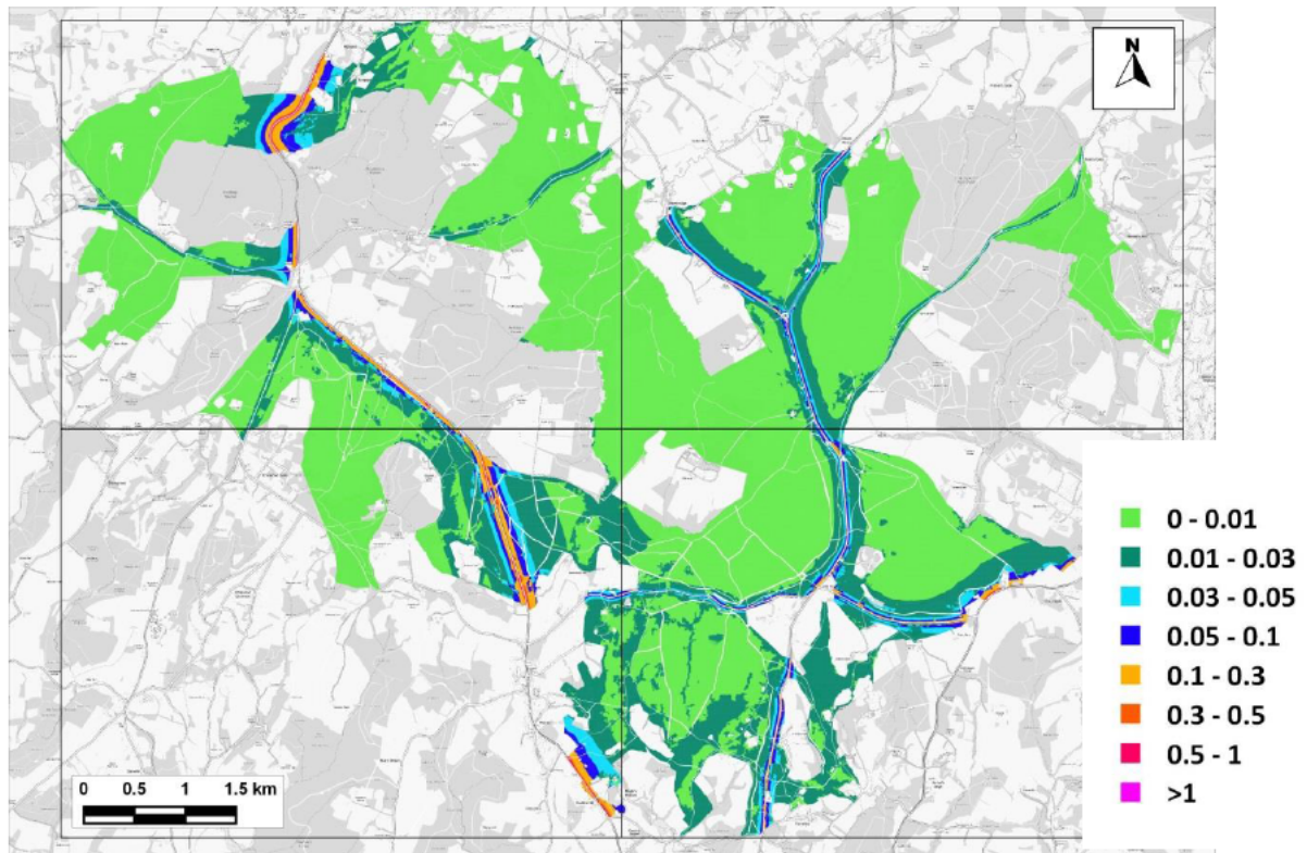
Figure 13.17: Change in Predicted Nitrogen Deposition to SAC Comparing 'With Plan' to 'No WDC-Growth' under Emissions Scenario B (AQC Method) (kg-N/ha/yr)
