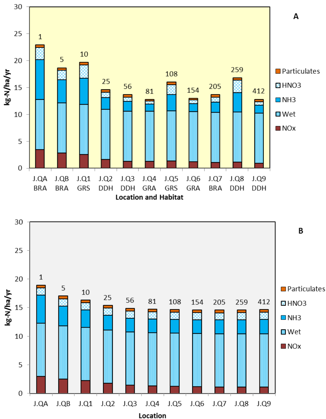
Figure 9.40: Deposition to Ecological Transect J – AQC Method – (A) Using Current Habitat Types and (B) If all Habitat were Heath (approximate distance from the nearest main road to each quadrant to shown numerically above each column) 36
