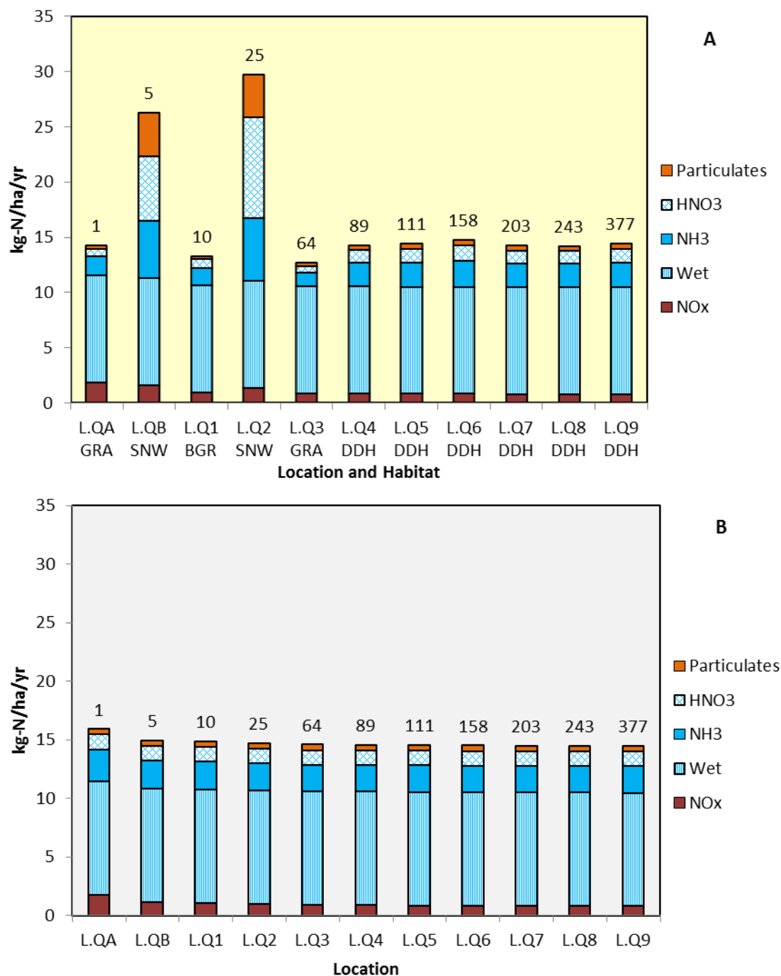
Figure 9.42: Deposition to Ecological Transect L – AQC Method – (A) Using Current Habitat Types and (B) If all Habitat were Heath (approximate distance from the nearest main road to each quadrant to shown numerically above each column) 36
