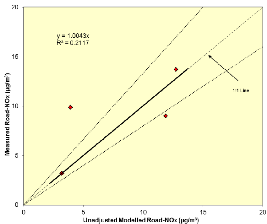
Figure 5.10: Modelled vs Measured Annual Mean Road-NOx, Link Set 3, Iteration 2
