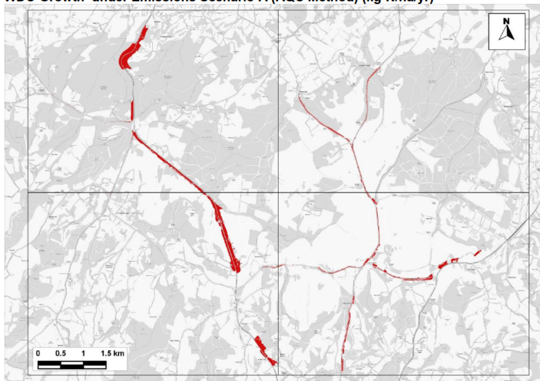
Figure 13.10: Areas in SAC Predicted to Experience an Increase in Nitrogen Deposition Greater than 1% of the 10 kg-N/ha/yr Critical Load where this Critical Load would also be Exceeded - Comparing 'With Plan' to 'No WDC-Growth' Scenarios under Emissions Scenario A (AQC Method)
