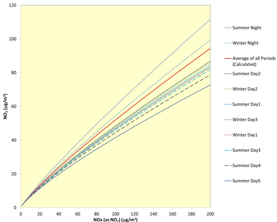
Figure 5.27: Lines of Best-fit for Period-specific NOx to NO 2 Relationships at Eight Automatic Monitoring Sites (ten periods) as a Function of the Total NOx Concentration
