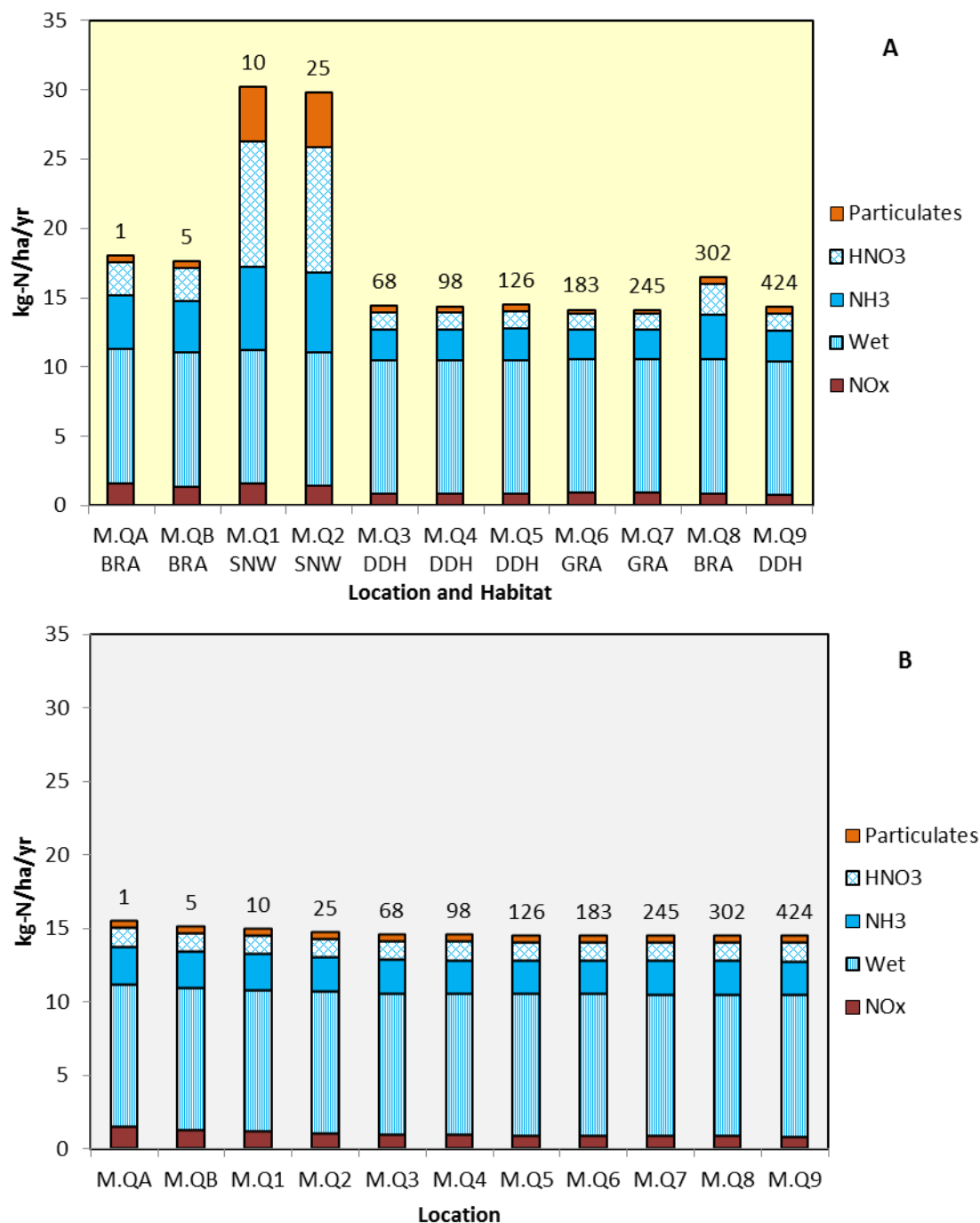
Figure 9.43: Deposition to Ecological Transect M – AQC Method – (A) Using Current Habitat Types and (B) If all Habitat were Heath (approximate distance from the nearest main road to each quadrant to shown numerically above each column) 36
