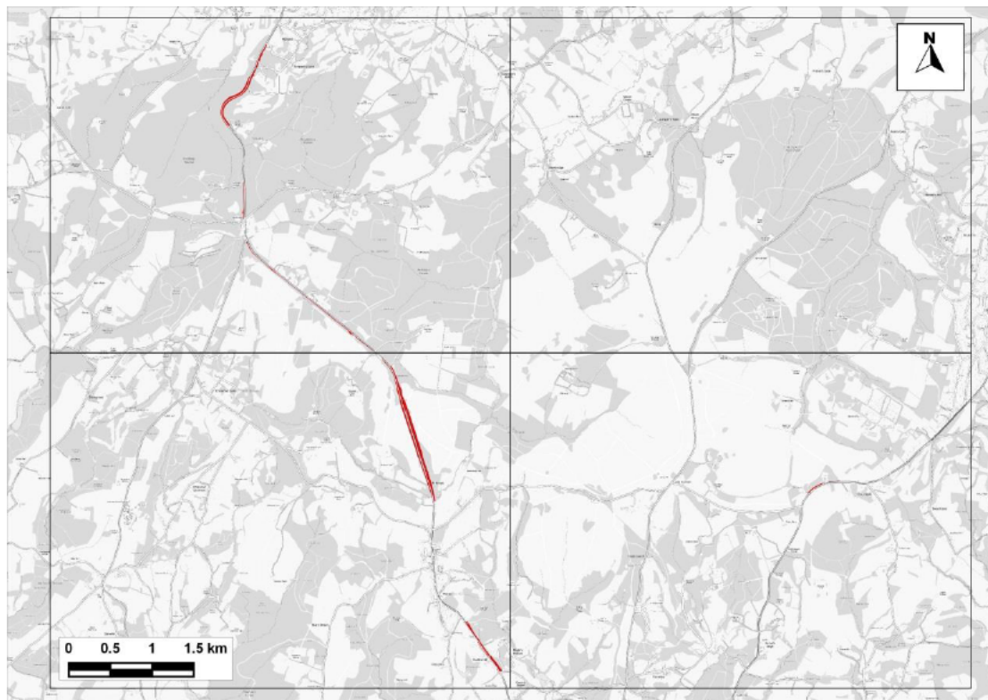
Figure 13.4: Areas in SAC Predicted to Experience an Increase in 24-hour Mean NO x Concentrations Greater than 10% of the 75 \mu\text{g}/\text{m}^3 Critical Level where the Critical Level would also be Exceeded - Comparing 'With Plan' to 'No WDC-Growth' Scenarios under Emissions Scenario A
