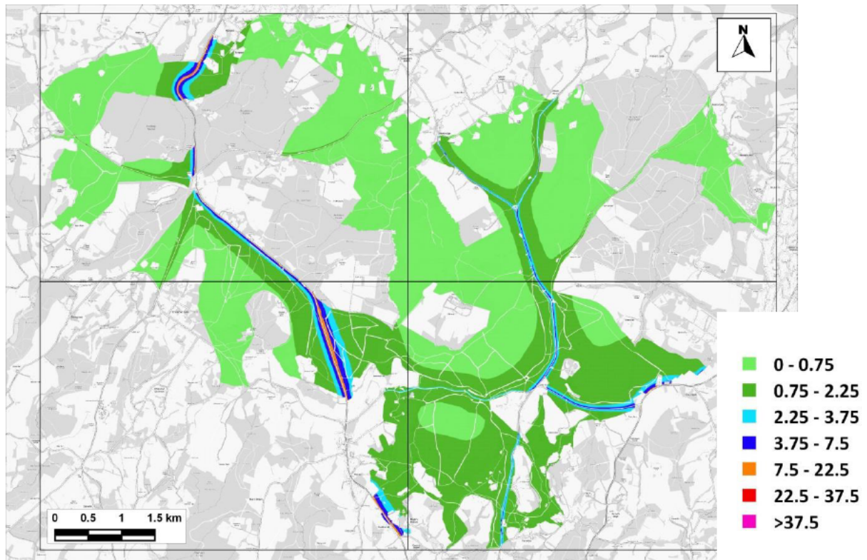
Figure 13.3: Change in Maximum Predicted 24-hour Mean NO x Comparing 'With Plan' to 'No WDC-Growth' under Emissions Scenario A ( \mu\text{g}/\text{m}^3 )
