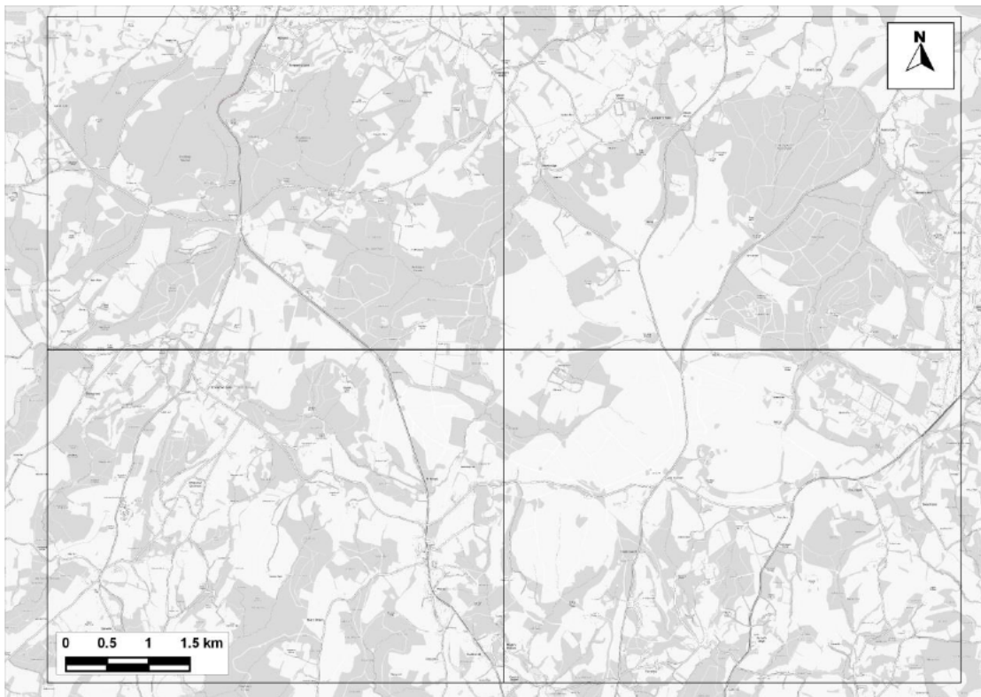
Figure 14.20: Areas in SAC Predicted to Experience an Increase in Annual Mean NO x Concentrations Greater than 1% of the 30 µg/m 3 Critical Level where the Critical Level would also be Exceeded - Comparing 'With Plan' to 'No Growth' Scenarios under Emissions Scenario C
