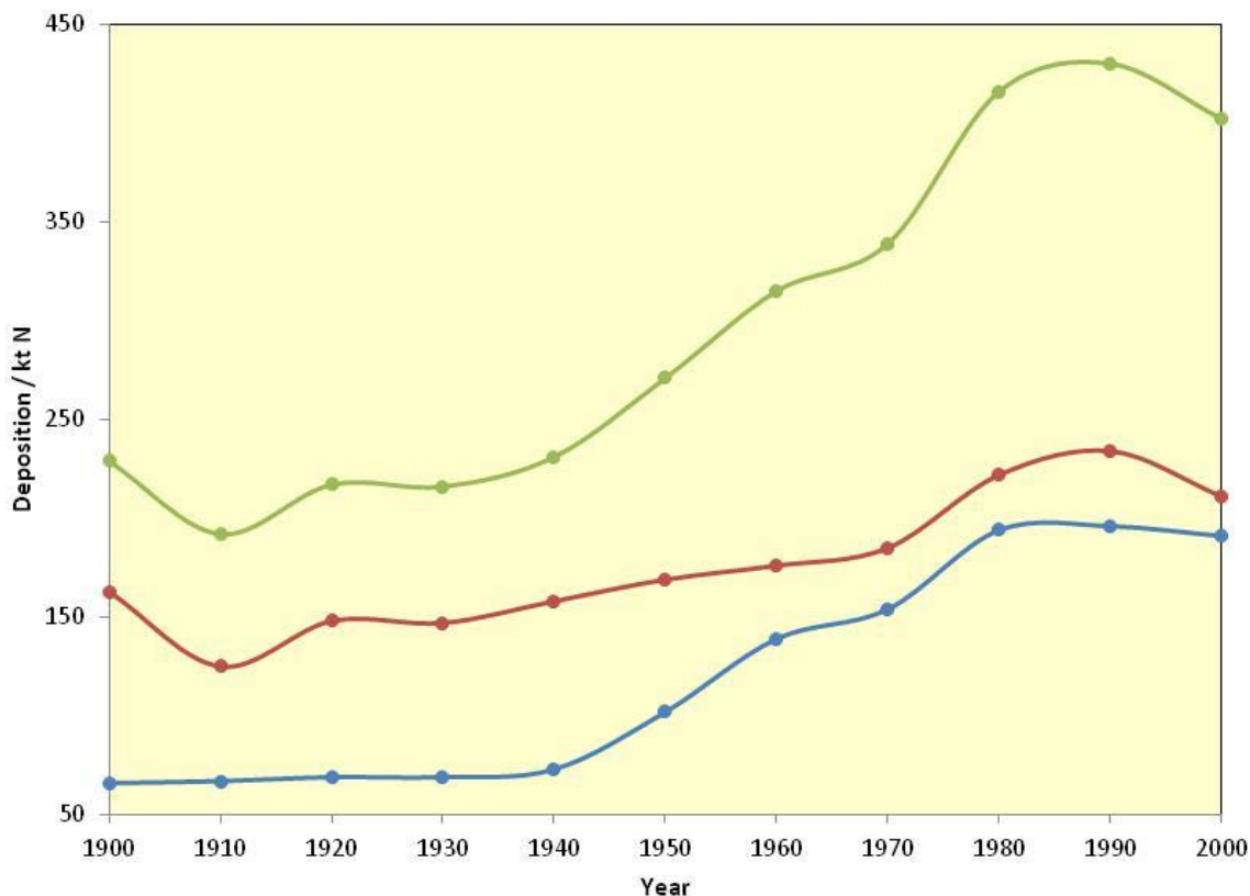
Figure 3.8: Predicted Historic Nitrogen Deposition to the UK during the 20 th Century (After Fowler et al. (2004)) Blue line shows oxidised nitrogen, red line shows reduced nitrogen, and green line shows total deposition
