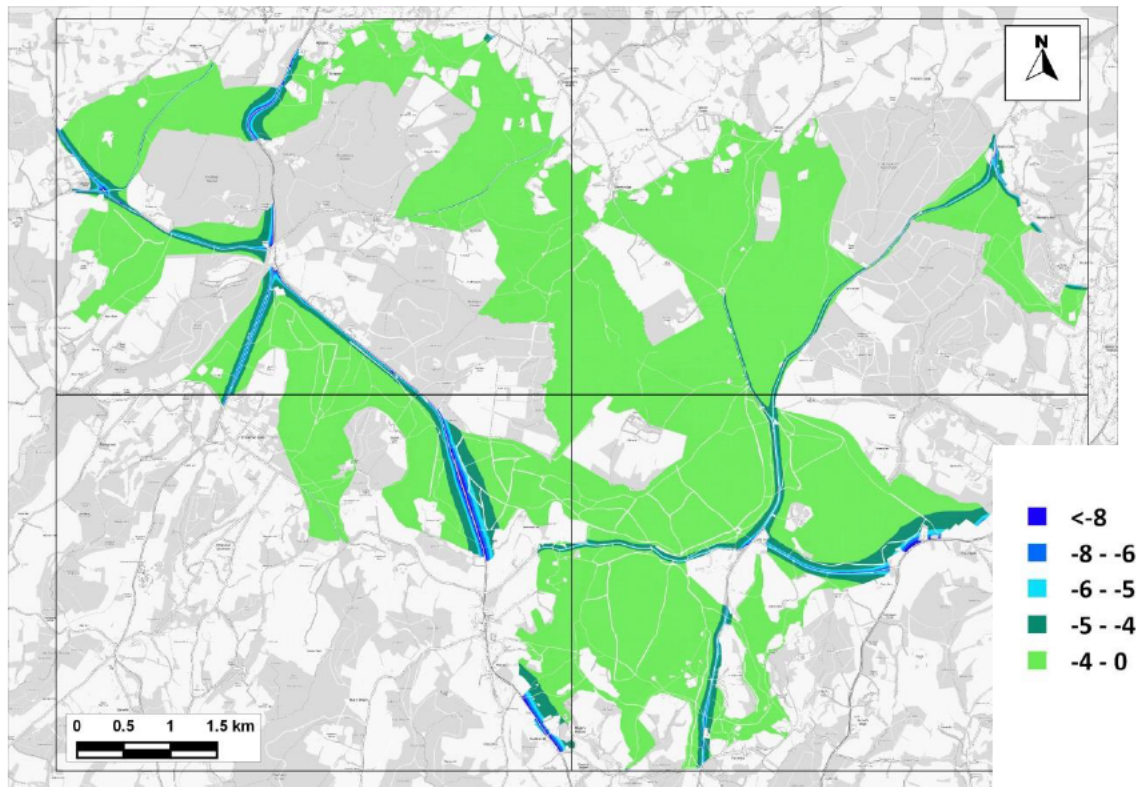
Figure 15.1: Change in Predicted Annual Mean NO x Comparing 'With Plan' Emissions Scenario B to 'No Growth' Emissions Scenario A (µg/m 3 )
