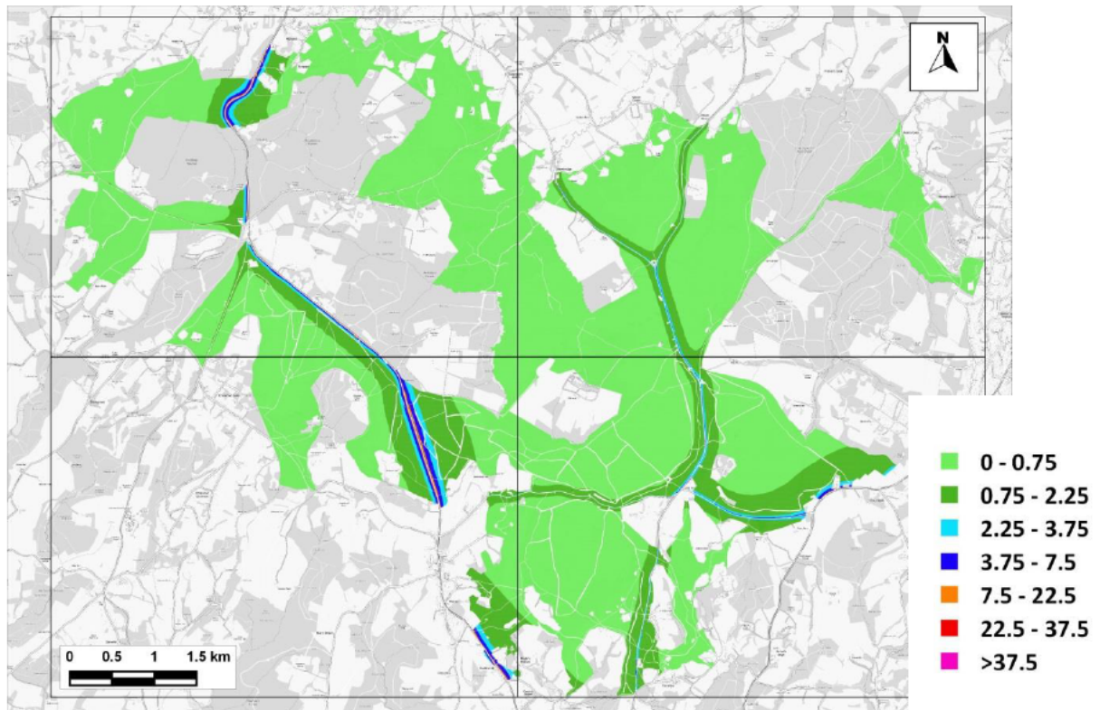
Figure 13.13: Change in Maximum Predicted 24-hour Mean NO x Comparing 'With Plan' to 'No WDC-Growth' under Emissions Scenario B ( \mu\text{g}/\text{m}^3 )
