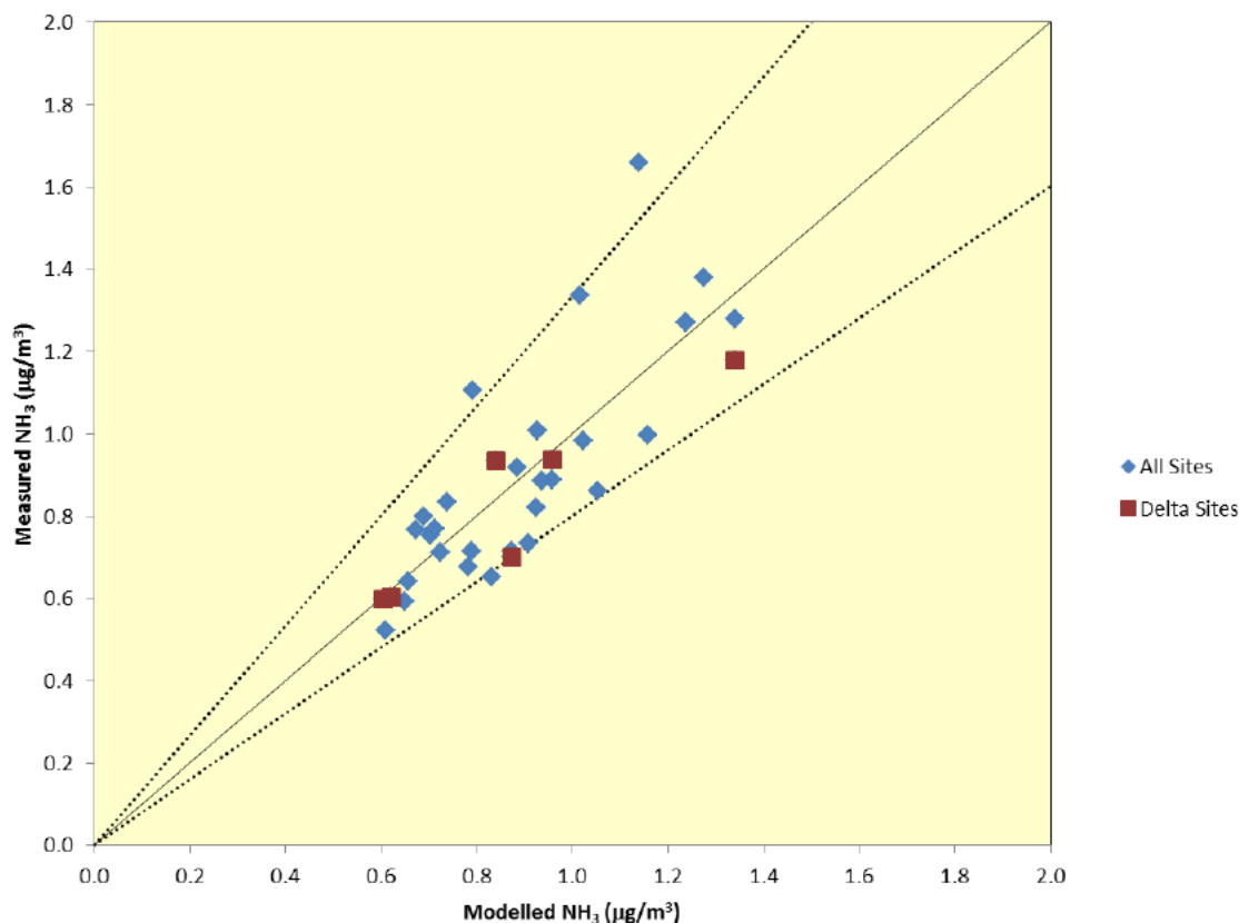
Figure 5.25: Measured vs Predicted Annual Mean \text{NH}_3
