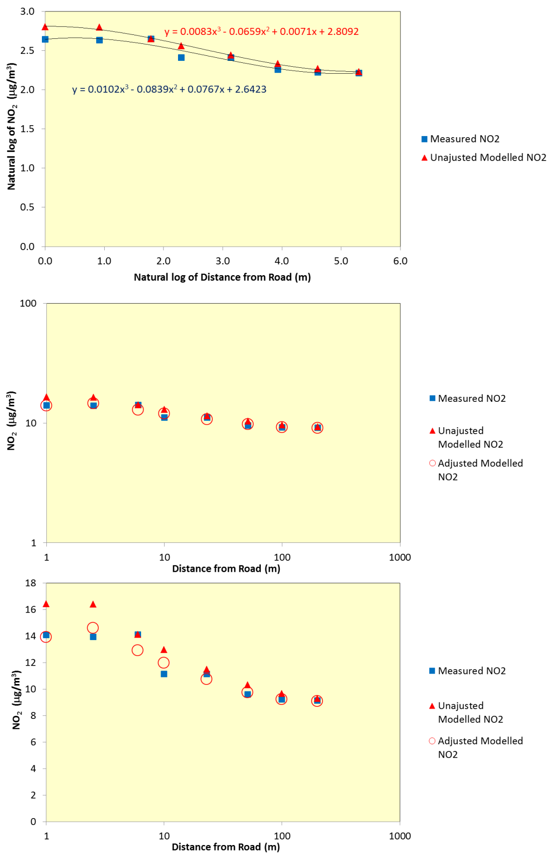
Figure 5.32: Measured vs Predicted 2-Year Average NO 2 Concentrations along Transect 3: top = unadjusted model on log scales, middle = unadjusted and adjusted models on log 'y' scale; bottom = unadjusted and adjusted models.
