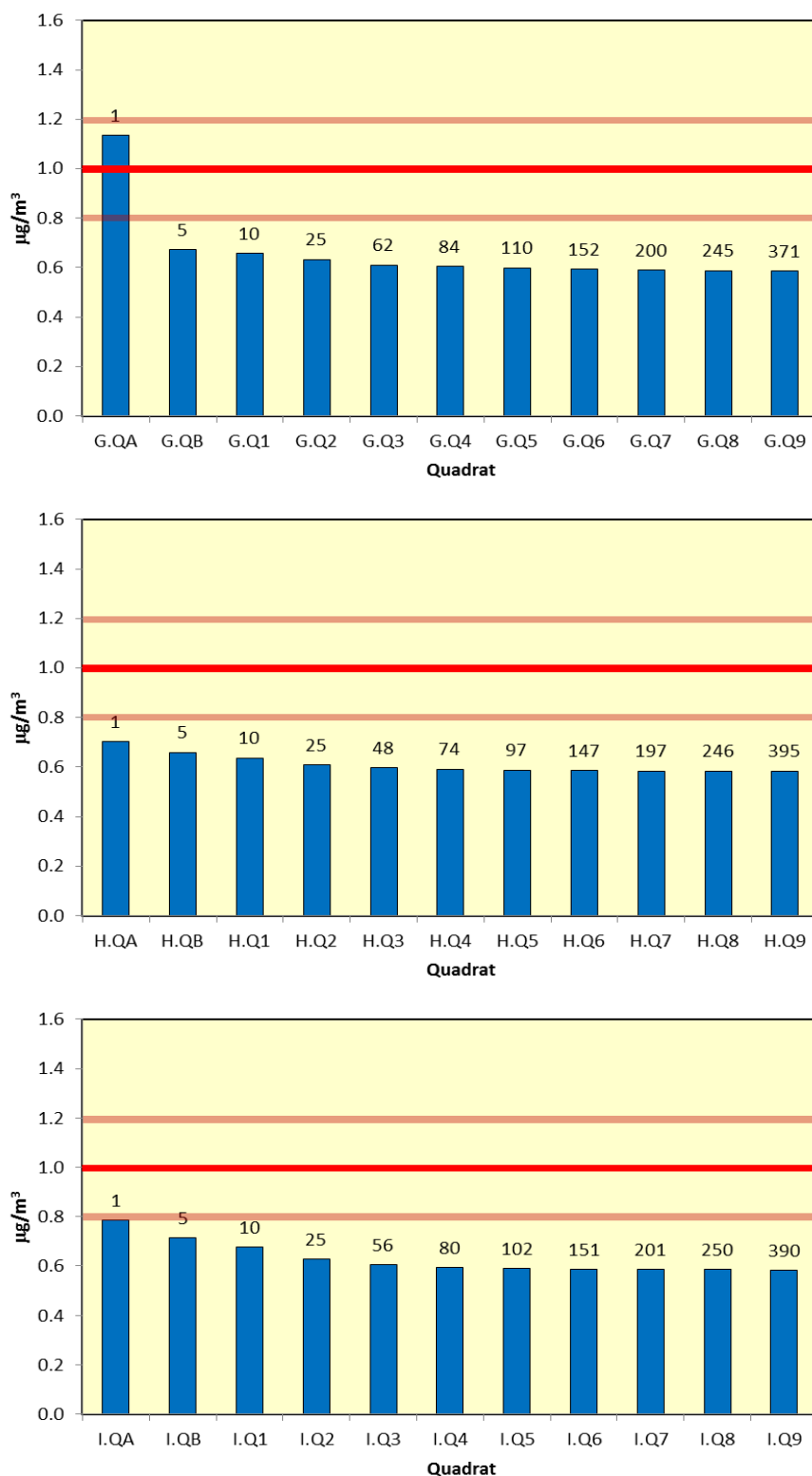
Figure 9.13: Annual Mean NH 3 Concentrations Along Transects G, H, and I. Approximate distance from the nearest main road to each quadrat to shown numerically above each column. Lines show the 1 µg/m 3 critical level and the +/-20% critical level range suggested by CEH.
