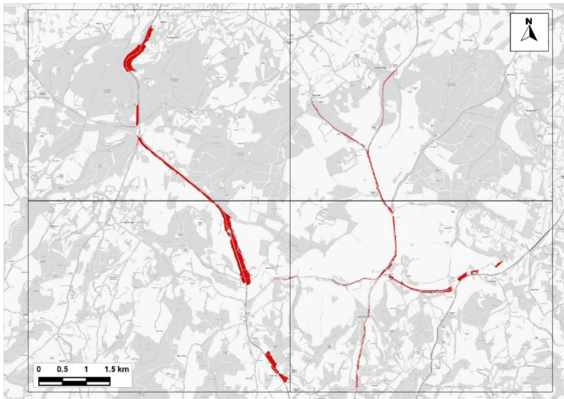
Figure 13.16: Areas in SAC Predicted to Experience an Increase in Nitrogen Deposition Greater than 1% of the 10 kg-N/ha/yr Critical Load where this Critical Load would also be Exceeded - Comparing 'With Plan' to 'No WDC-Growth' Scenarios under Emissions Scenario B (EA Method)
