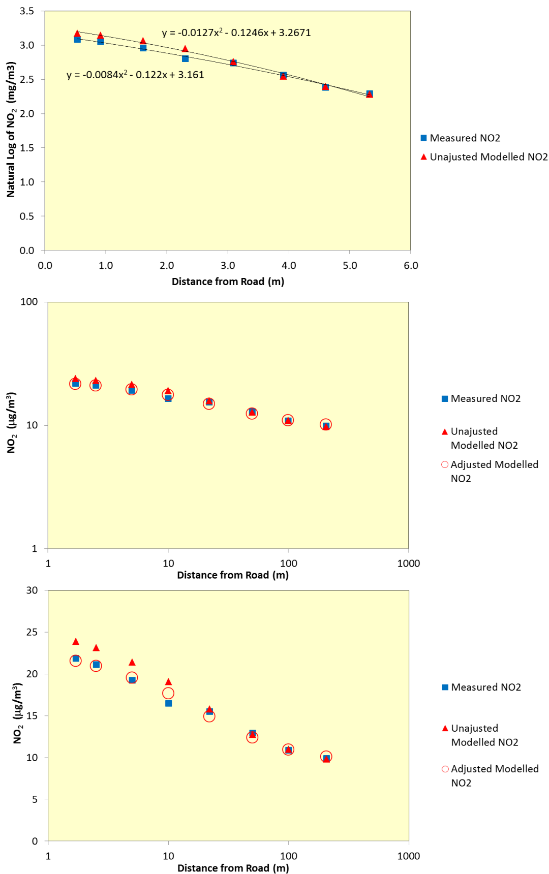
Figure 5.31: Natural Log of Measured vs Predicted 2-Year Average NO 2 Concentrations along Transect 2: top = unadjusted model on log scales, middle = unadjusted and adjusted models on log 'y' scale; bottom = unadjusted and adjusted models
