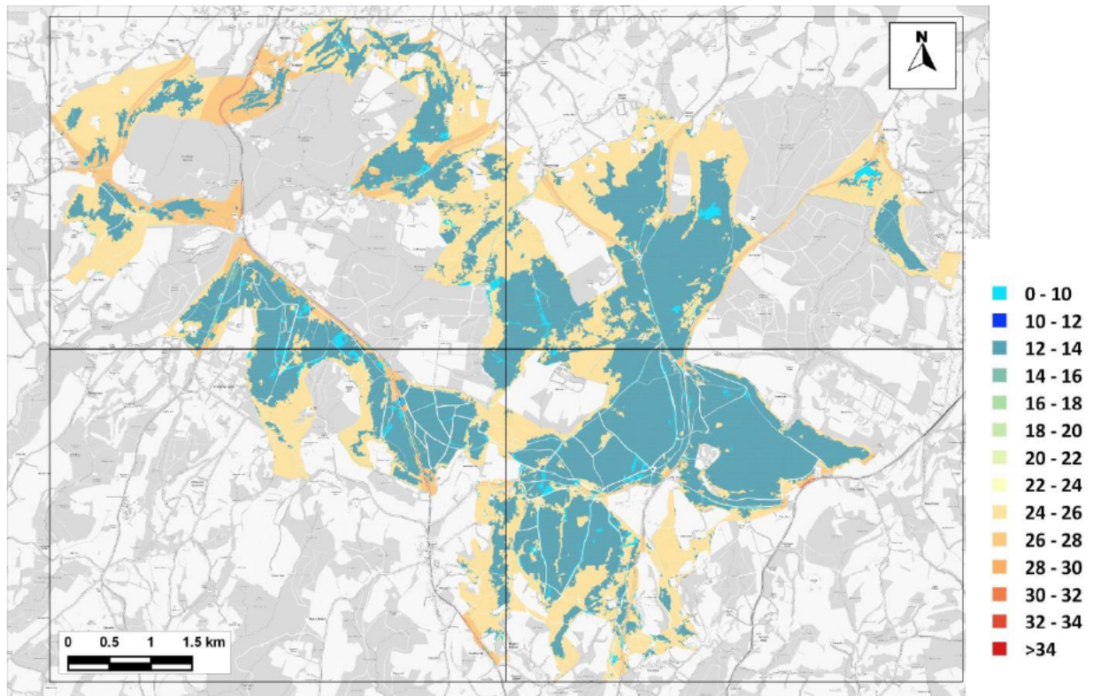
Figure 10.4: Nitrogen Deposition to SAC – 2028 No-Growth - B (AQC Method) (kg-N/ha/yr)
