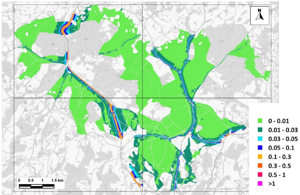
Figure 13.25: Change in Predicted Nitrogen Deposition to SAC Comparing 'With Plan' to 'No WDC-Growth' under Emissions Scenario C (AQC Method) (kg-N/ha/yr)
