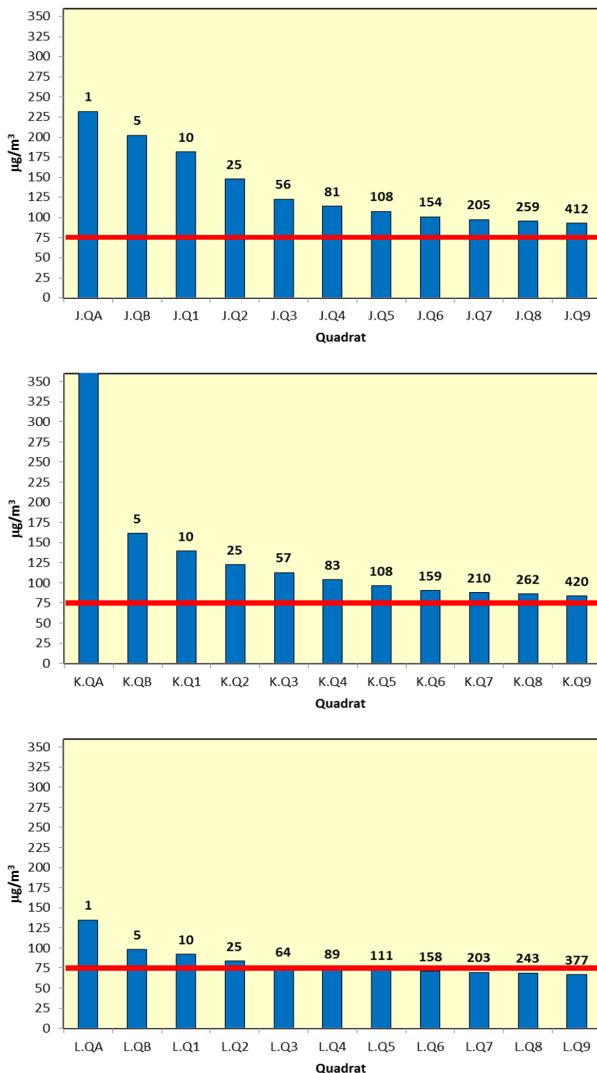
Figure 9.9: Maximum 24-hour Mean NO x Concentrations Along Transects J, K, and L. Approximate distance from the nearest main road to each quadrant to shown numerically above each column. Horizontal line shows the 75 µg/m 3 critical level. The value for Quadrat K.QA is 377 µg/m 3 .
