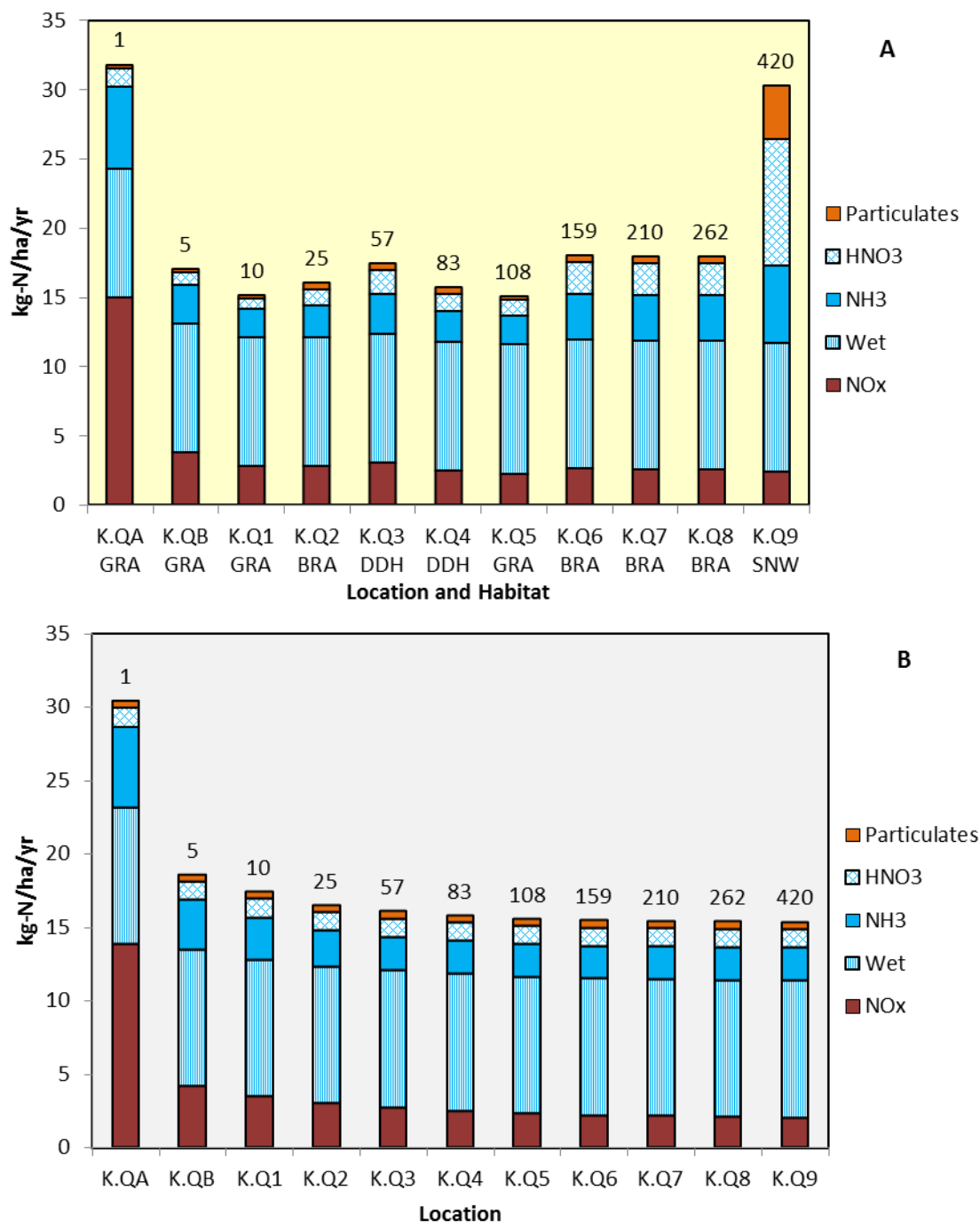
Figure 9.26: Deposition to Ecological Transect K – EA Method – A Using Current Habitat Types and B If all Habitat were Heath (approximate distance from the nearest main road to each quadrant to shown numerically above each column) 36
