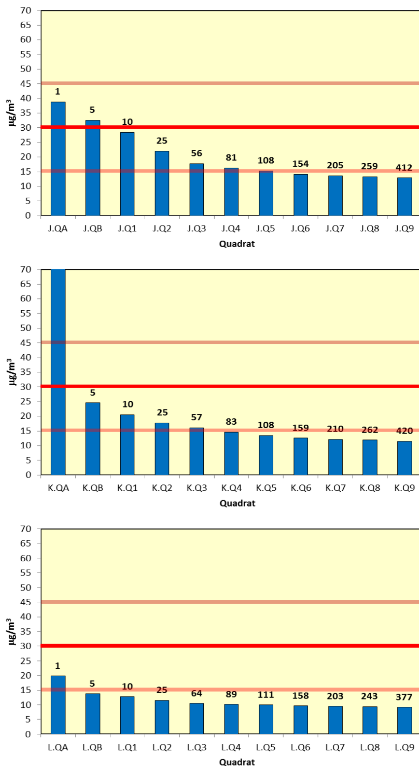
Figure 9.4: Annual Mean NO x Concentrations Along Transects J, K, and L. Approximate distance from the nearest main road to each quadrant to shown numerically above each column. Lines show the 30 µg/m 3 critical level and the 15 µg/m 3 and 45 µg/m 3 critical level range suggested by CEH. The value for Quadrat K.QA is 75.1 µg/m 3 .
