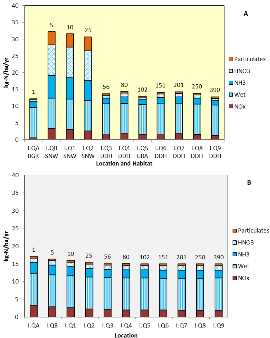
Figure 9.24: Deposition to Ecological Transect I – EA Method – A Using Current Habitat Types and B If all Habitat were Heath (approximate distance from the nearest main road to each quadrant to shown numerically above each column) 36
