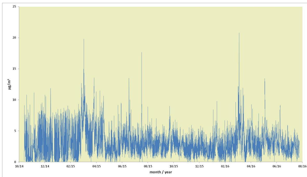
Figure 8.3: 1-hour Mean NHx Concentrations at Kingstanding between October 2014 and August 2016
