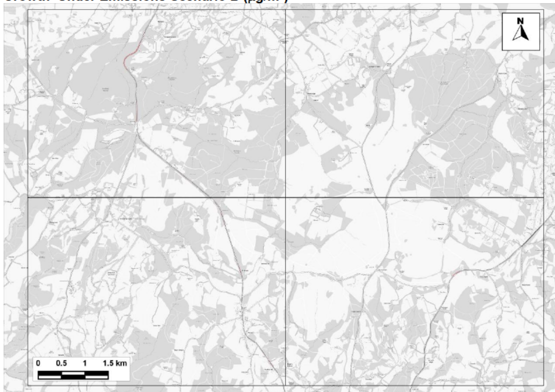
Figure 13.12: Areas in SAC Predicted to Experience an Increase in Annual Mean NO x Concentrations Greater than 1% of the 30 \mu\text{g}/\text{m}^3 Critical Level where the Critical Level would also be Exceeded - Comparing 'With Plan' to 'No WDC-Growth' Scenarios under Emissions Scenario B
