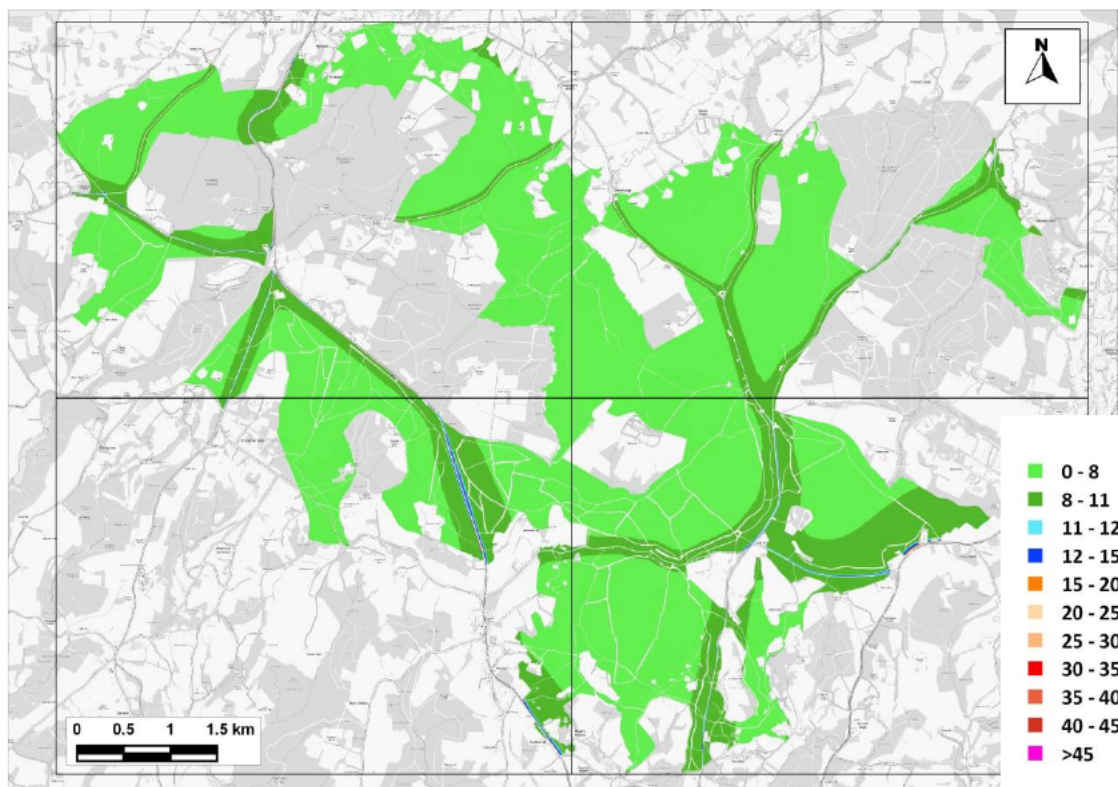
Figure 10.5: Predicted Annual Mean NO x Concentrations across the SAC– 2028 No-Growth - C ( \mu\text{g}/\text{m}^3 )
