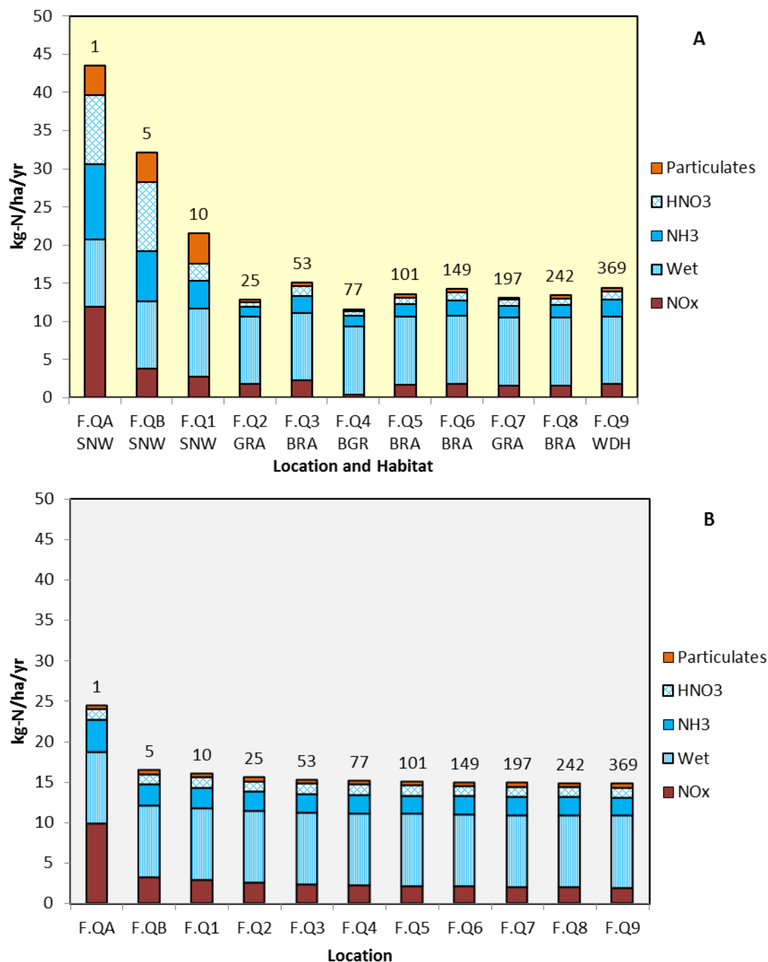
Figure 9.21: Deposition to Ecological Transect F – EA Method – A Using Current Habitat Types and B If all Habitat were Heath (approximate distance from the nearest main road to each quadrant to shown numerically above each column) 36,37
