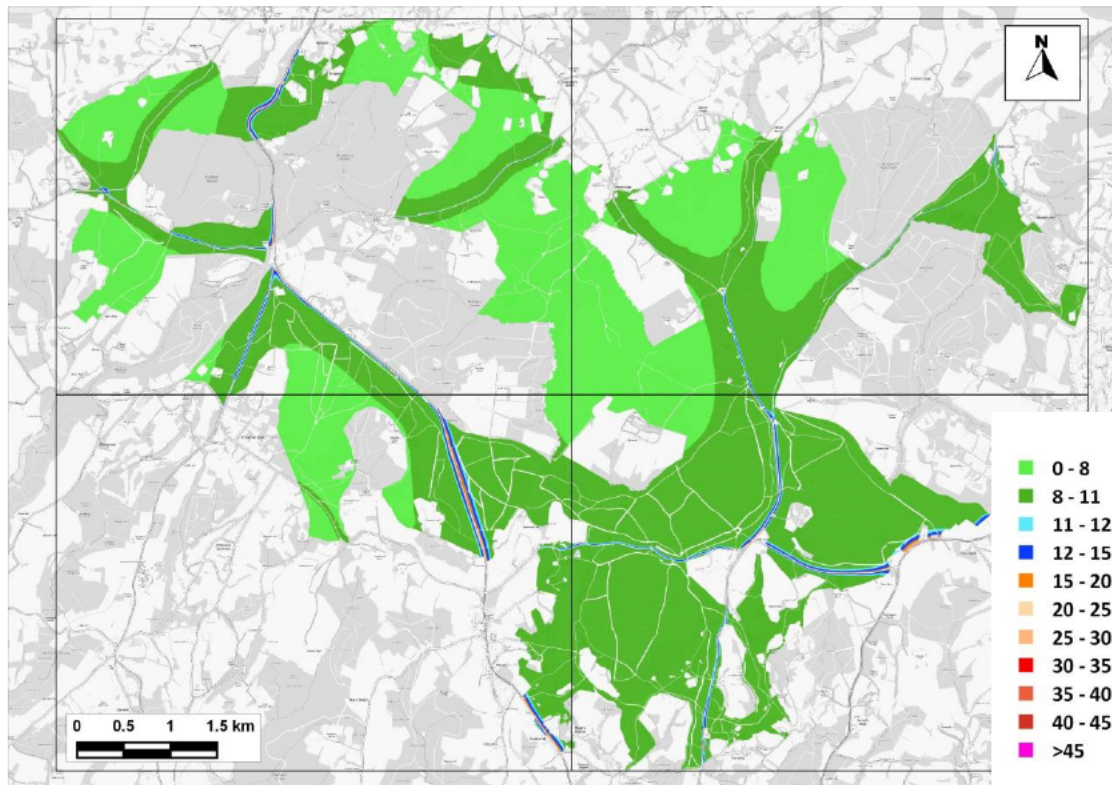
Figure 11.6: Predicted Annual Mean NOx Concentrations across the SAC– 2028 No WDC-Growth - B ( \mu\text{g}/\text{m}^3 )
