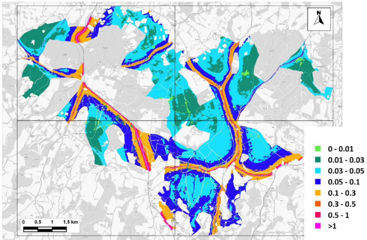
Figure 14.7: Change in Predicted Nitrogen Deposition to SAC Comparing 'With Plan' to 'No Growth' Scenarios Under Emission Scenario A (EA Method) (kg-N/ha/yr)
