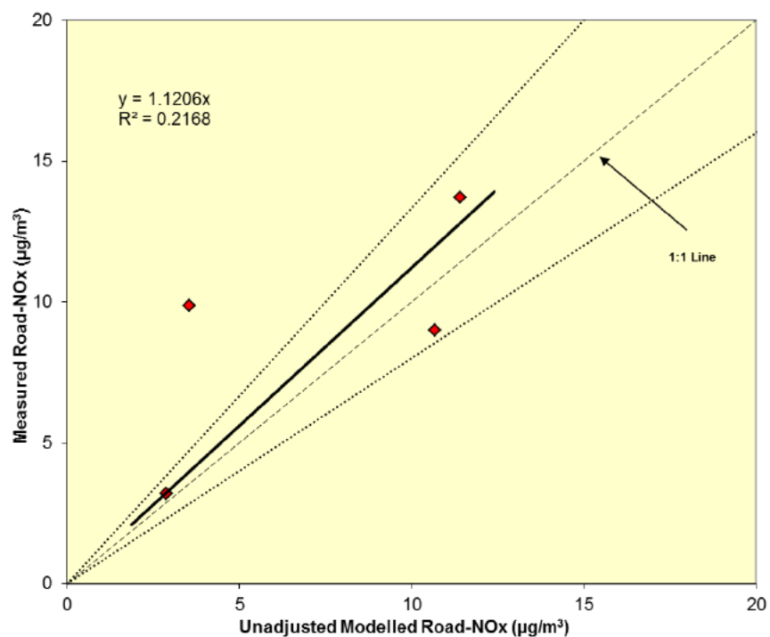
Figure 5.7: Modelled vs Measured Annual Mean Road-NOx, Link Set 3, Iteration 1
