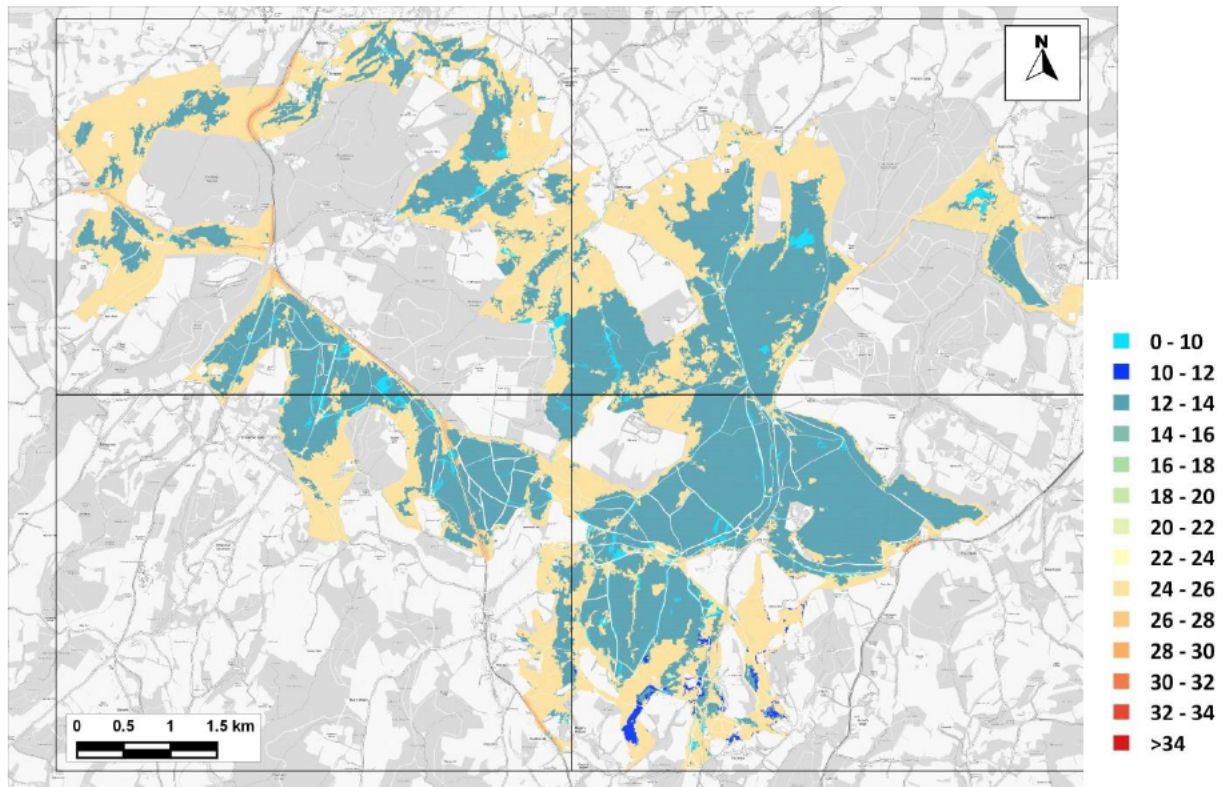
Figure 10.8: Nitrogen Deposition to SAC – 2028 No-Growth - C (AQC Method) (kg-N/ha/yr)
