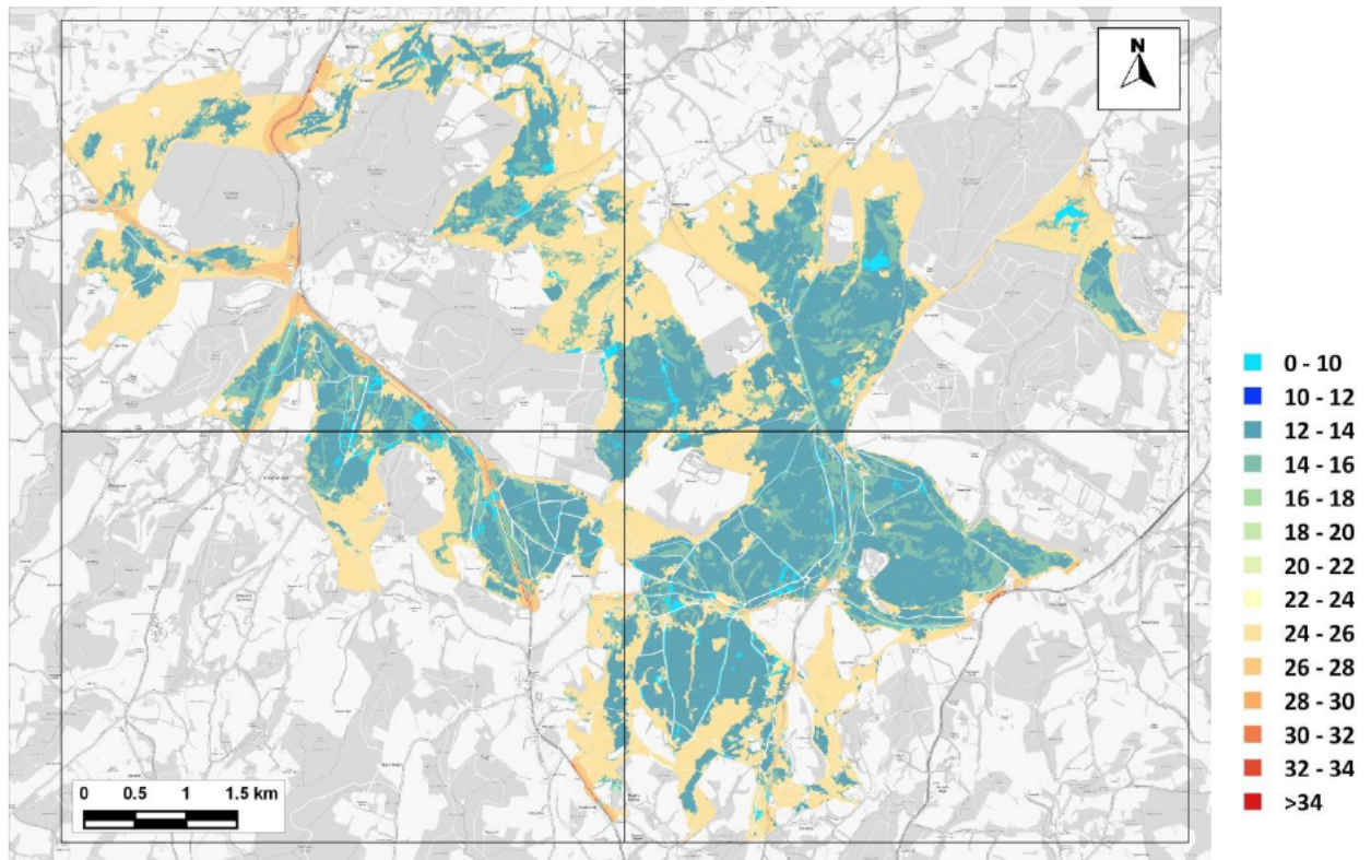
Figure 12.12: Nitrogen Deposition to SAC – 2028 With Plan – C (EA Method) (kg-N/ha/yr)
