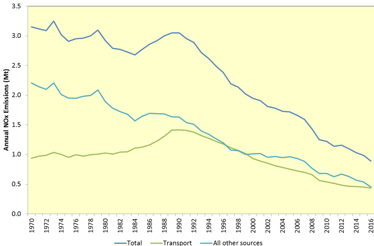
Figure 3.7: UK Total NOx Emissions: 1970 – 2016 (Defra, 2018b)
