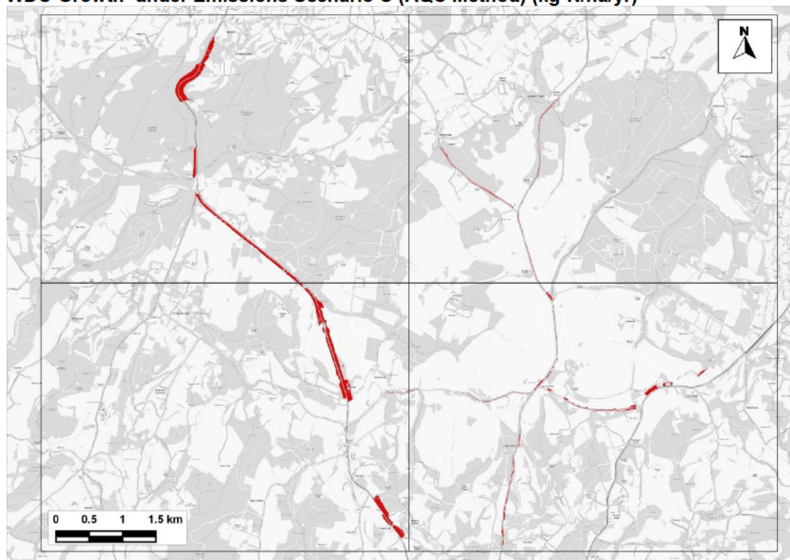
Figure 13.26: Areas in SAC Predicted to Experience an Increase in Nitrogen Deposition Greater than 1% of the 10 kg-N/ha/yr Critical Load where this Critical Load would also be Exceeded - Comparing 'With Plan' to 'No WDC-Growth' Scenarios under Emissions Scenario C (AQC Method)
