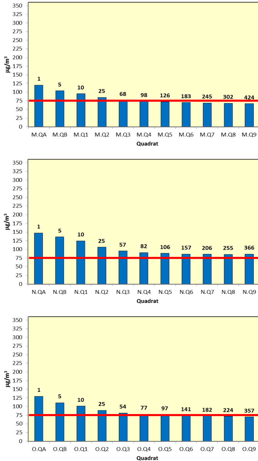
Figure 9.10: Maximum 24-hour Mean NOx Concentrations Along Transects M,N and O. Approximate distance from the nearest main road to each quadrat to shown numerically above each column. Horizontal line shows the 75 µg/m³ critical level.
