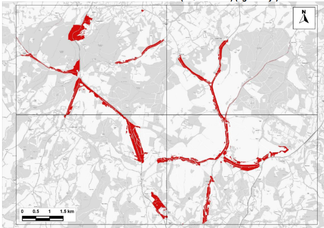
Figure 14.10: Areas in SAC Predicted to Experience an Increase in Nitrogen Deposition Greater than 1% of the 10 kg-N/ha/yr Critical Load where this Critical Load would also be Exceeded - Comparing 'With Plan' to 'No Growth' Scenarios under Emissions Scenario A (AQC Method)
