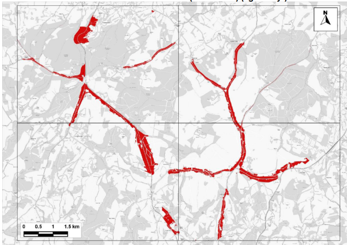
Figure 14.16: Areas in SAC Predicted to Experience an Increase in Nitrogen Deposition Greater than 1% of the 10 kg-N/ha/yr Critical Load where this Critical Load would also be Exceeded - Comparing 'With Plan' to 'No Growth' Scenarios under Emissions Scenario B (EA Method)
