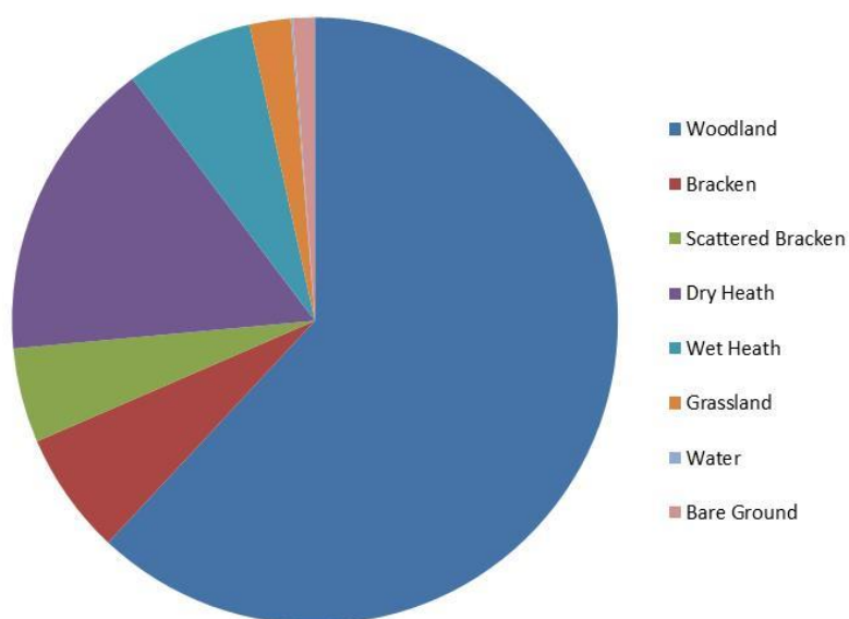
Figure 9.51: Total Nitrogen Deposition to Different Ashdown Forest SAC Land Surfaces (i.e. taking account of relative cover of each land use) (EA Method)
