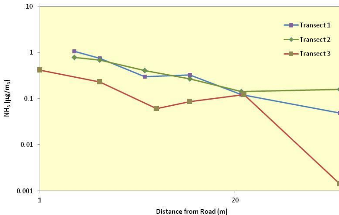
Figure 8.12: Two-year Mean Road- \text{NH}_3 (total minus assumed background) vs Distance from Roads along the Three Transects on Logarithmic Scales
