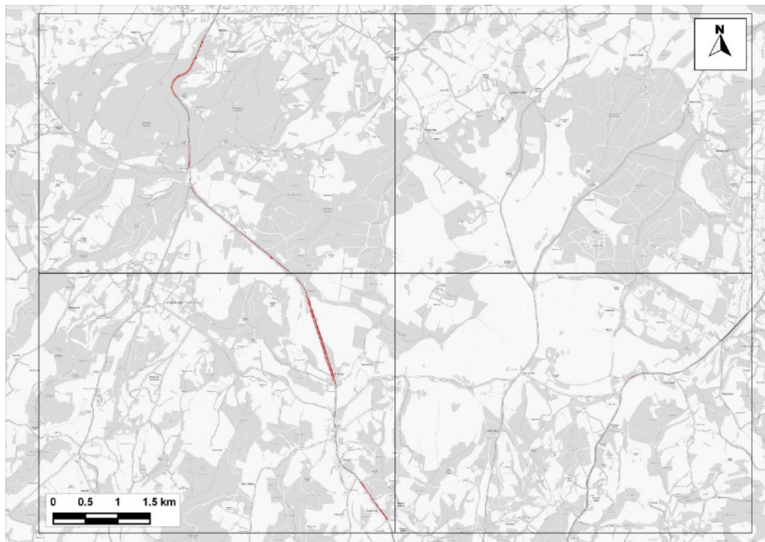
Figure 13.14: Areas in SAC Predicted to Experience an Increase in 24-hour Mean NO x Concentrations Greater than 10% of the 75 \mu\text{g}/\text{m}^3 Critical Level where the Critical Level would also be Exceeded - Comparing 'With Plan' to 'No WDC-Growth' Scenarios under Emissions Scenario B
