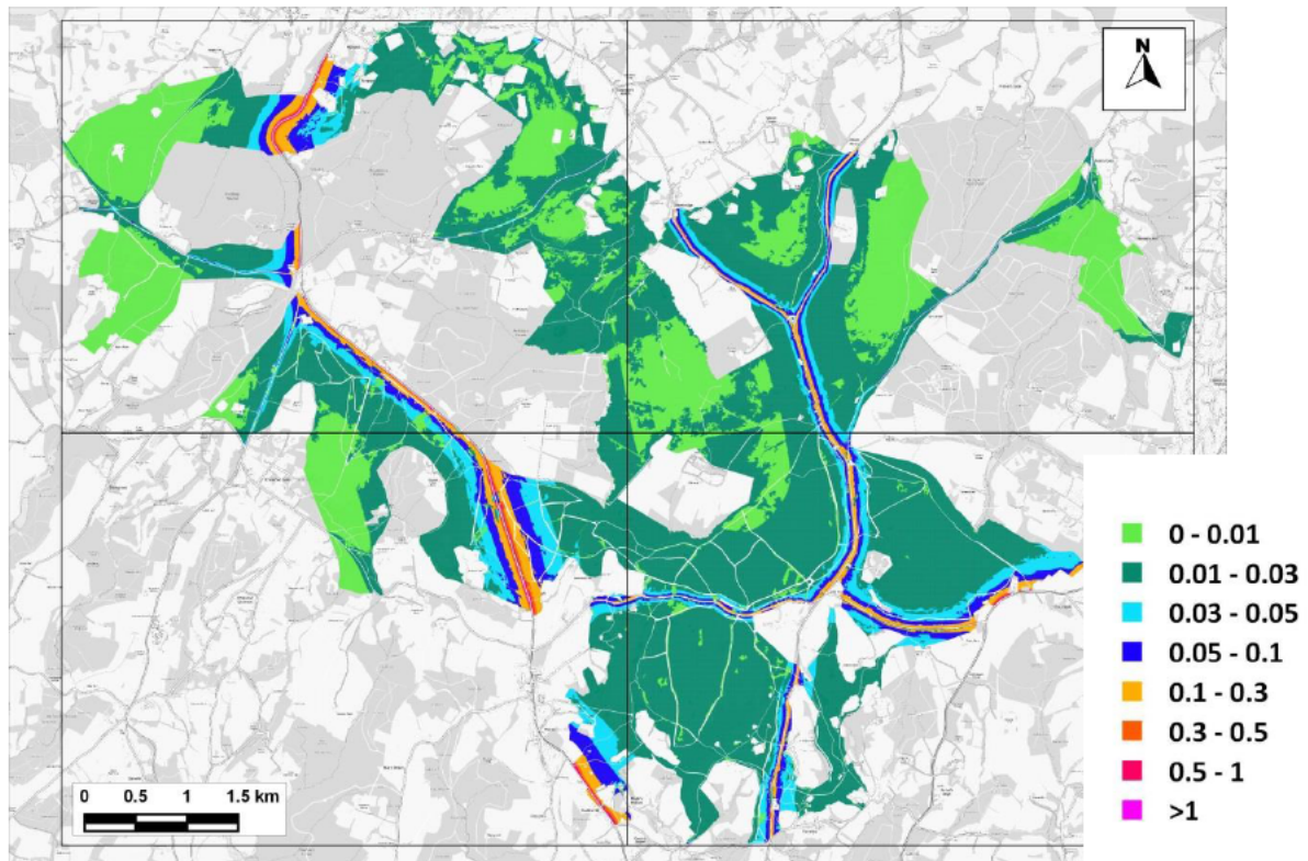
Figure 13.7: Change in Predicted Nitrogen Deposition to SAC Comparing 'With Plan' to 'No WDC-Growth' Under Emission Scenario A (EA Method) (kg-N/ha/yr)
