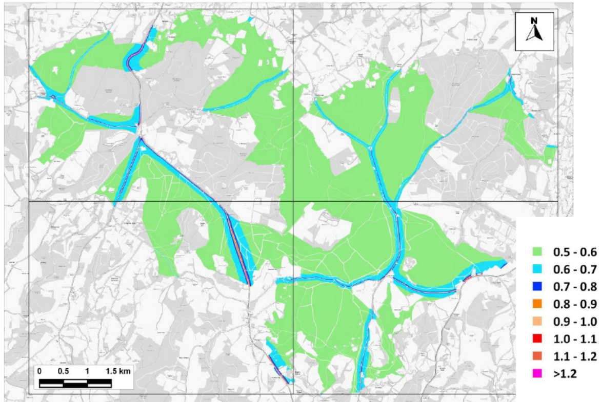
Figure 11.3: Predicted Annual Mean \text{NH}_3 Concentrations across the SAC– 2028 No WDC-Growth ( \mu\text{g}/\text{m}^3 )
