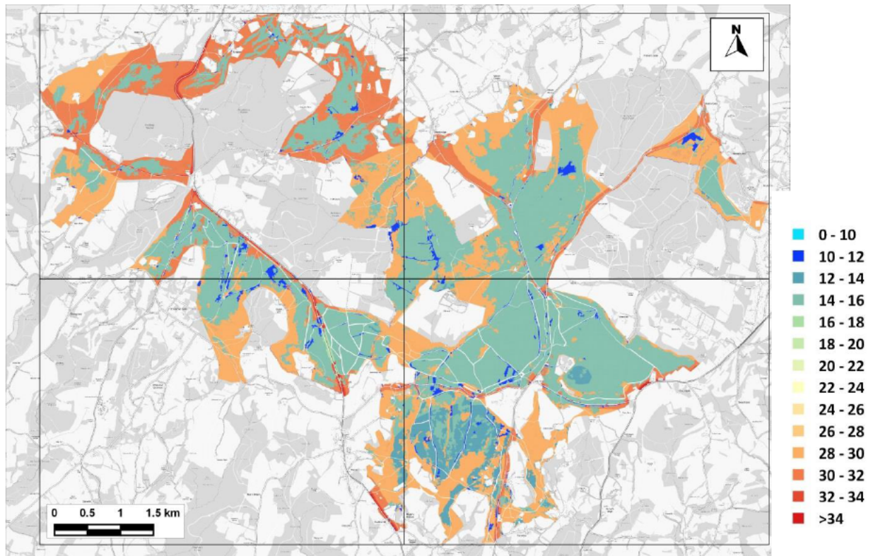
Figure 12.5: Nitrogen Deposition to SAC – 2028 With Plan - A (AQC Method) (kg-N/ha/yr)
