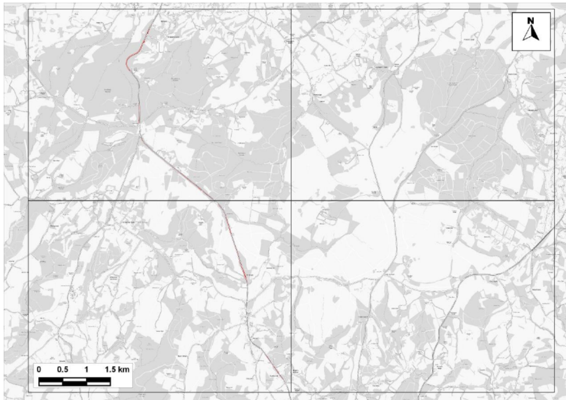
Figure 13.22: Areas in SAC Predicted to Experience an Increase in 24-hour Mean NO x Concentrations Greater than 10% of the 75 \mu\text{g}/\text{m}^3 Critical Level where the Critical Level would also be Exceeded - Comparing 'With Plan' to 'No WDC-Growth' Scenarios under Emissions Scenario C
