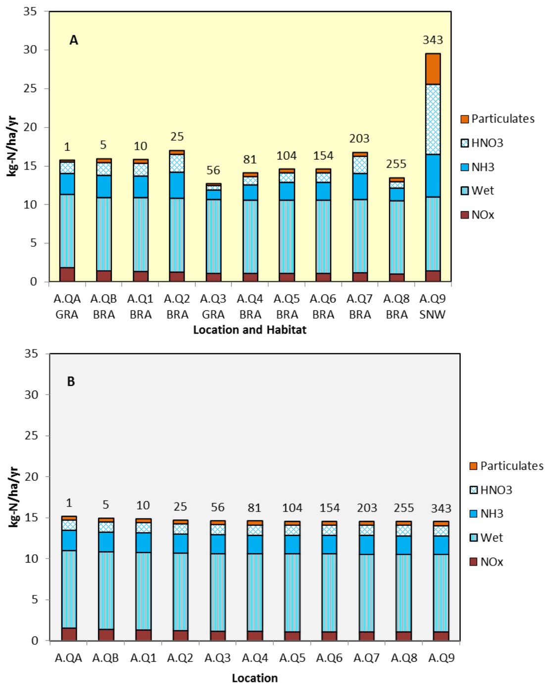
Figure 9.31: Deposition to Ecological Transect A – AQC Method – (A) Using Current Habitat Types and (B) If all Habitat were Heath (approximate distance from the nearest main road to each quadrant to shown numerically above each column) 36
