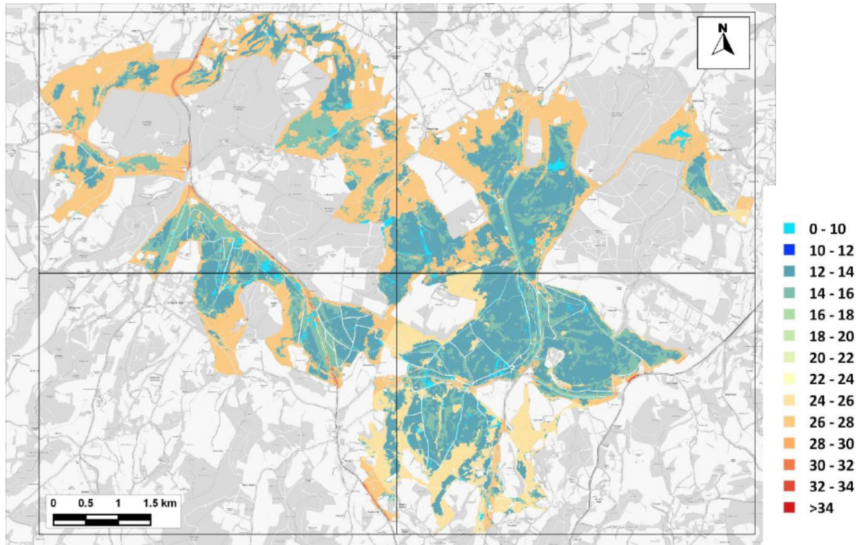
Figure 12.8: Nitrogen Deposition to SAC – 2028 With Plan - B (EA Method) (kg-N/ha/yr)
