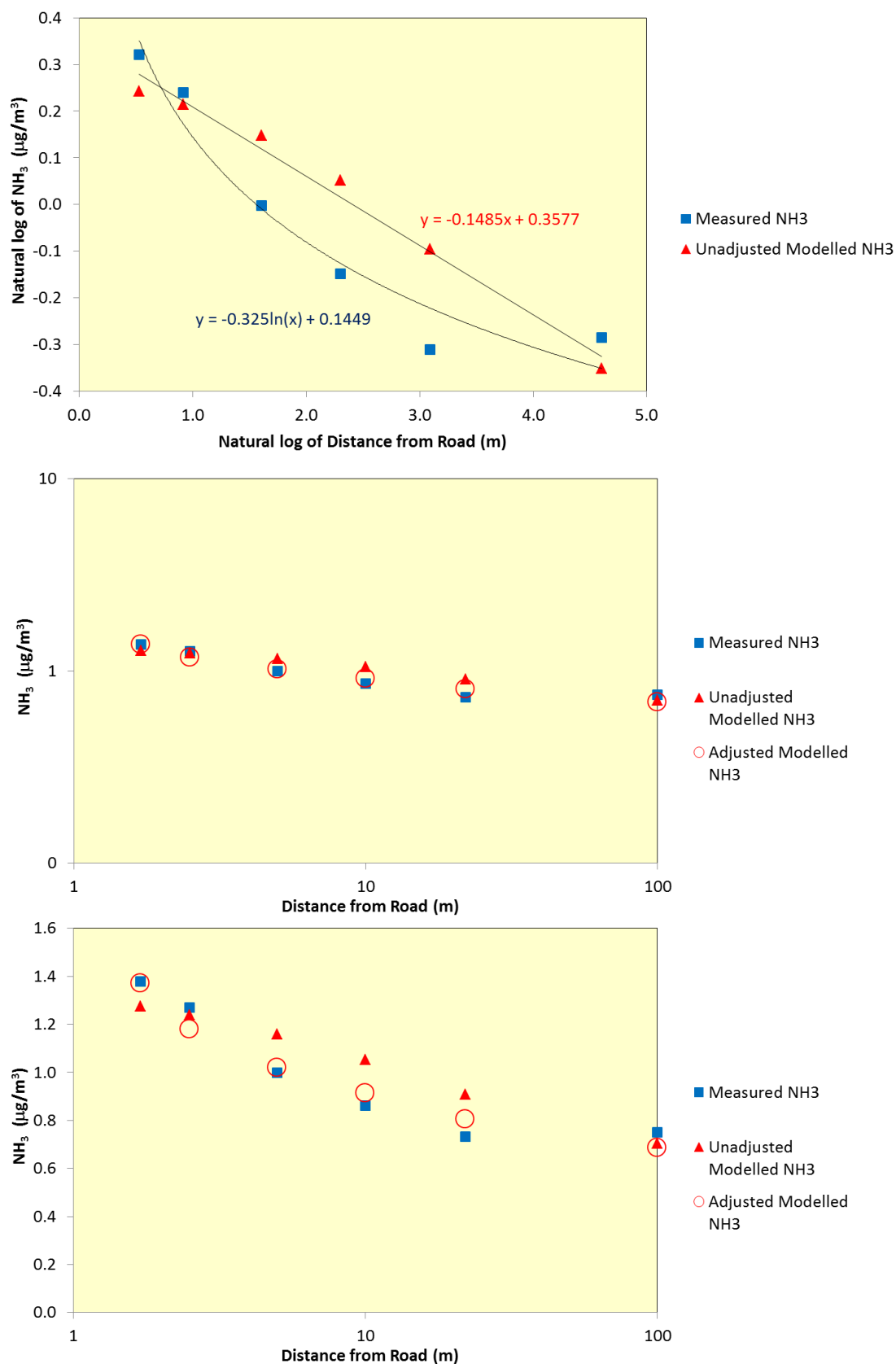
Figure 5.34: Measured vs Predicted 2-Year Average \text{NH}_3 Concentrations along Transect 2: top = unadjusted model on log scales, middle = unadjusted and adjusted models on log 'y' scale; bottom = unadjusted and adjusted models.
