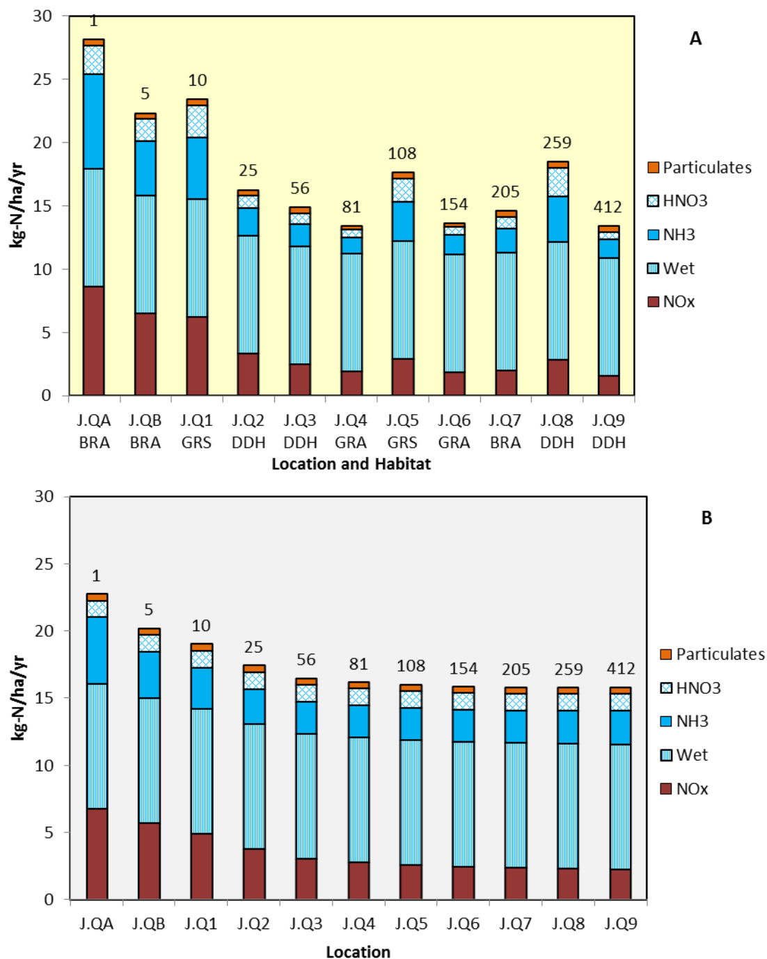
Figure 9.25: Deposition to Ecological Transect J – EA Method – A Using Current Habitat Types and B If all Habitat were Heath (approximate distance from the nearest main road to each quadrant to shown numerically above each column) 36
