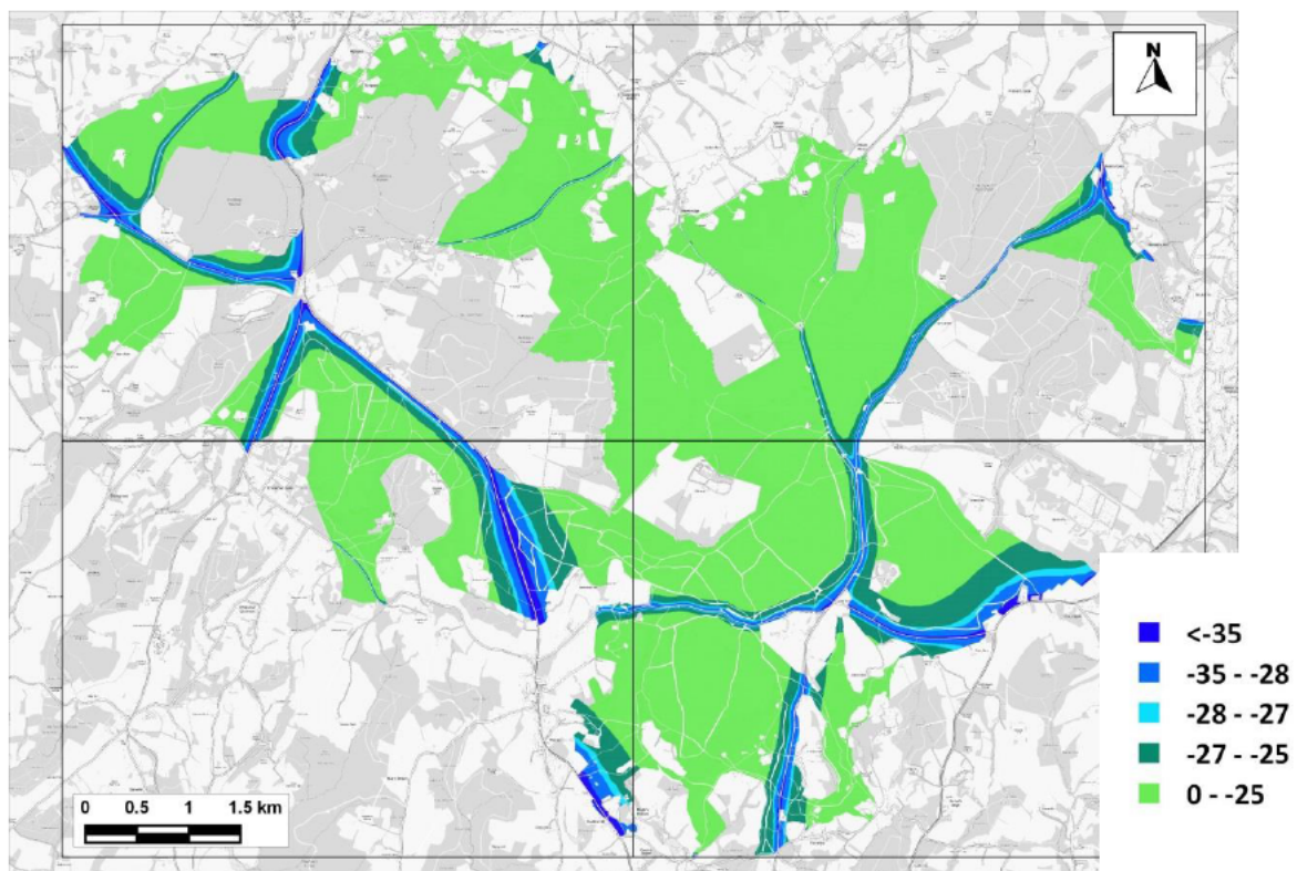
Figure 15.2: Change in Maximum Predicted 24-hour Mean NO x Comparing 'With Plan' Emissions Scenario B to 'No Growth' Emissions Scenario A ( \mu\text{g}/\text{m}^3 )
