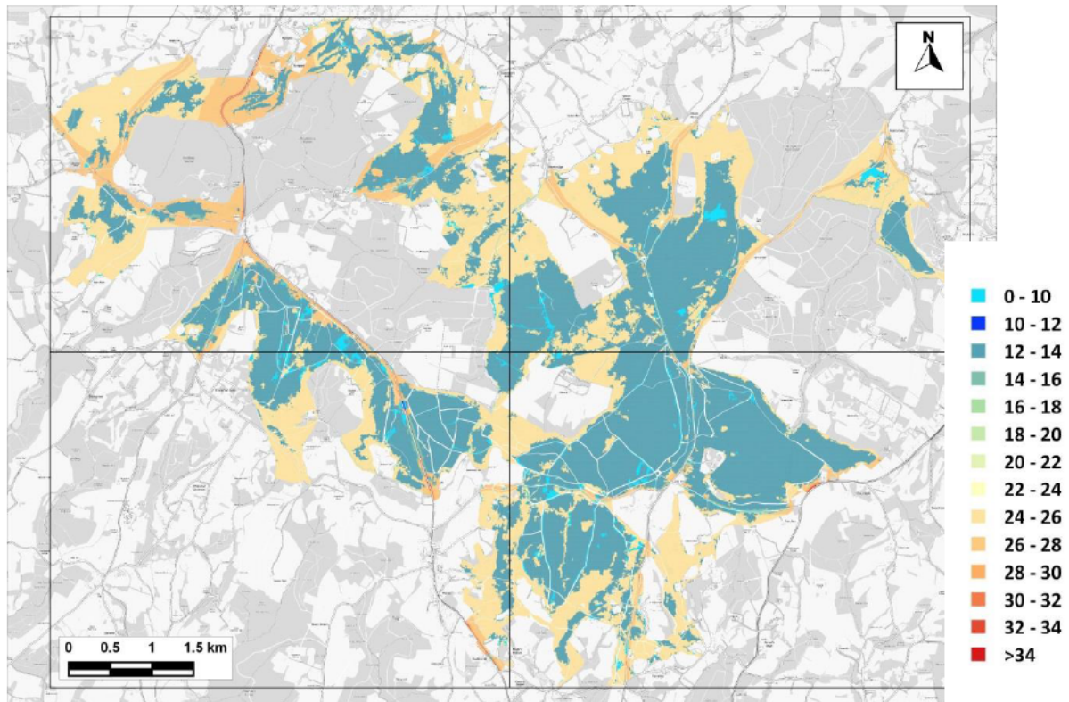
Figure 11.9: Nitrogen Deposition to SAC – 2028 No WDC-Growth - B (AQC Method) (kg-N/ha/yr)
