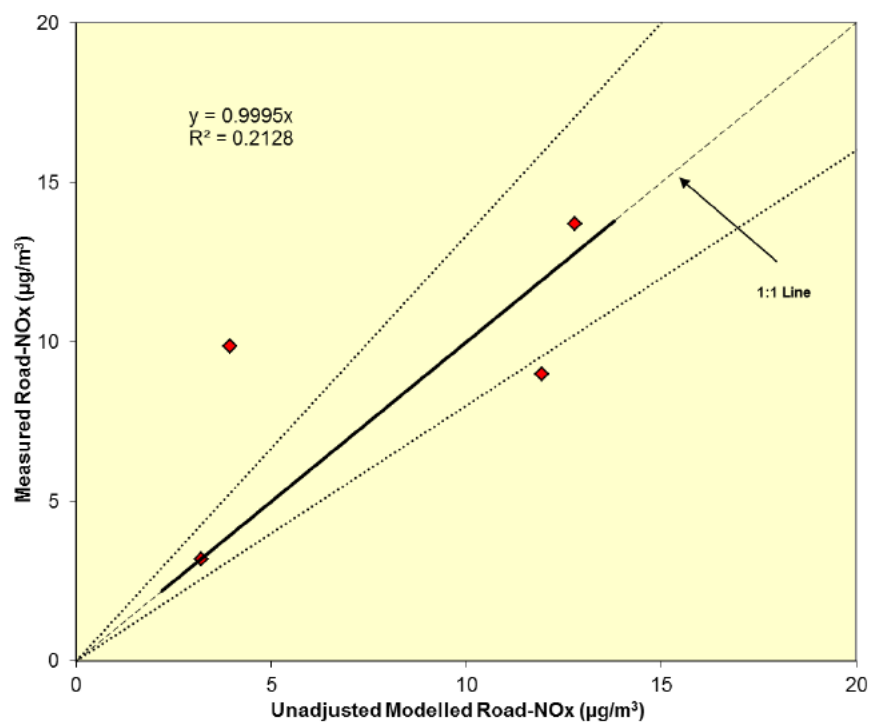
Figure 5.13: Modelled vs Measured Annual Mean Road-NOx, Link Set 3, Iteration 3
