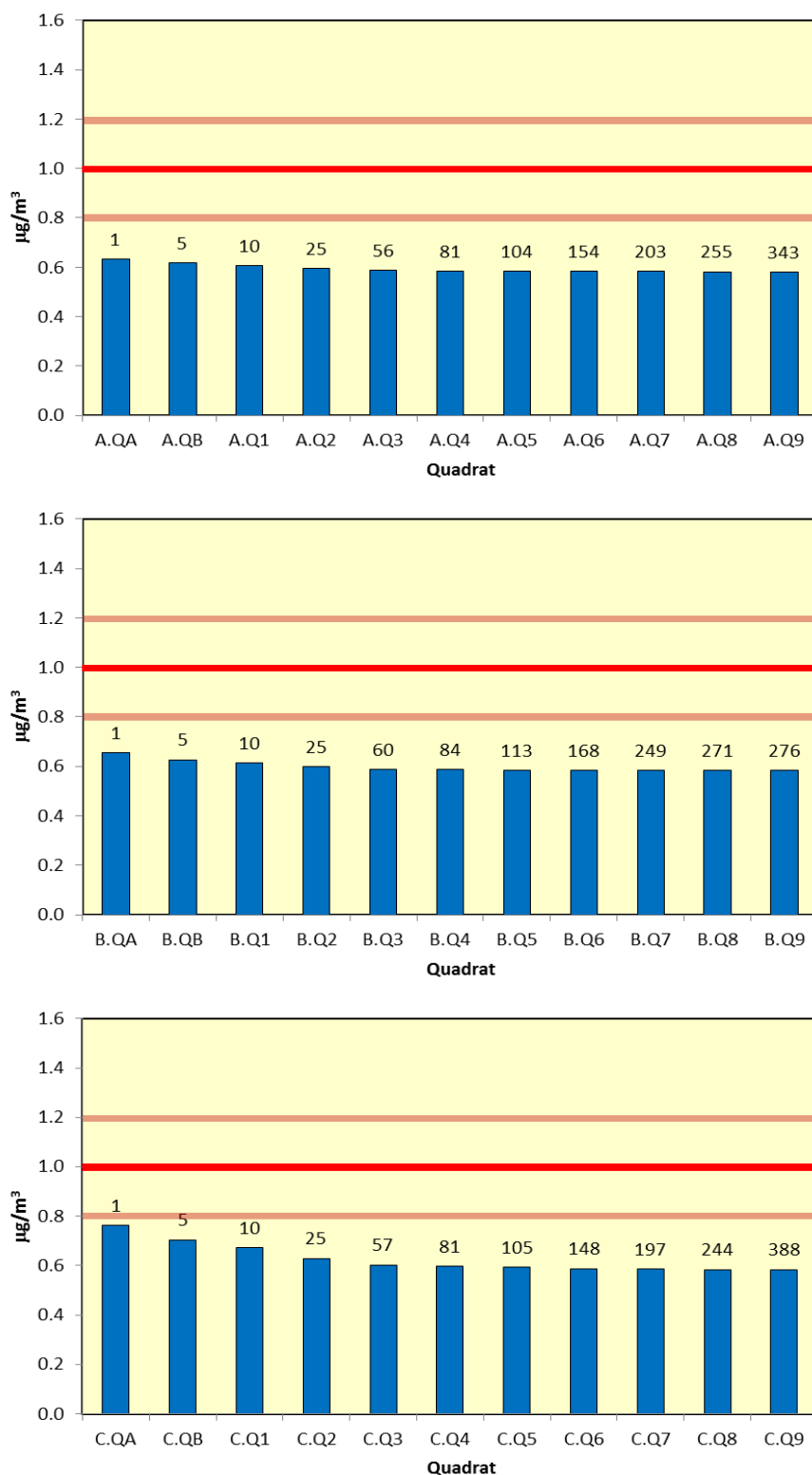
Figure 9.11: Annual Mean NH 3 Concentrations Along Transects A, B, and C. Approximate distance from the nearest main road to each quadrant to shown numerically above each column. Lines show the 1 µg/m 3 critical level and the +/-20% critical level range suggested by CEH.
