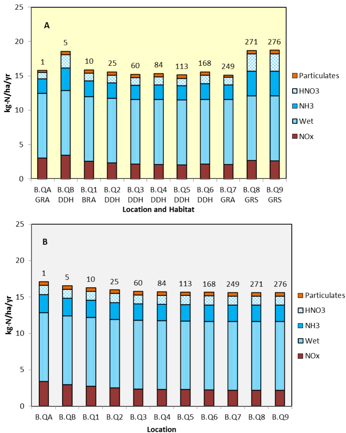
Figure 9.17: Deposition to Ecological Transect B – EA Method – A Using Current Habitat Types and B If all Habitat were Heath (approximate distance from the nearest main road to each quadrant to shown numerically above each column) 36
