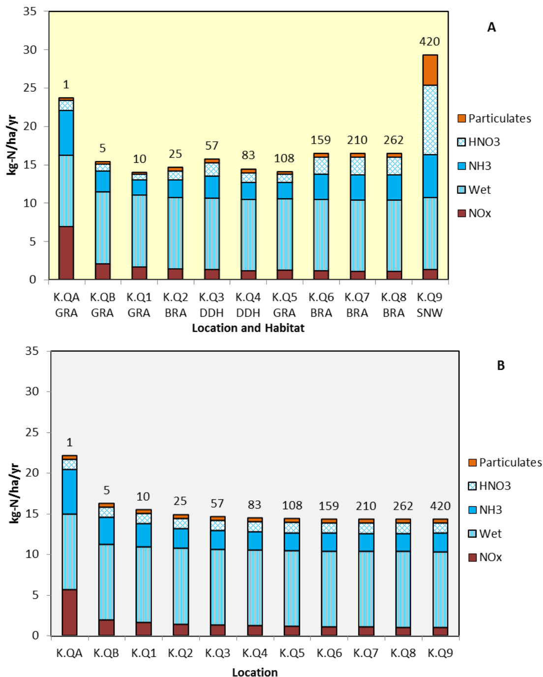
Figure 9.41: Deposition to Ecological Transect K – AQC Method – (A) Using Current Habitat Types and (B) If all Habitat were Heath (approximate distance from the nearest main road to each quadrant to shown numerically above each column) 36
