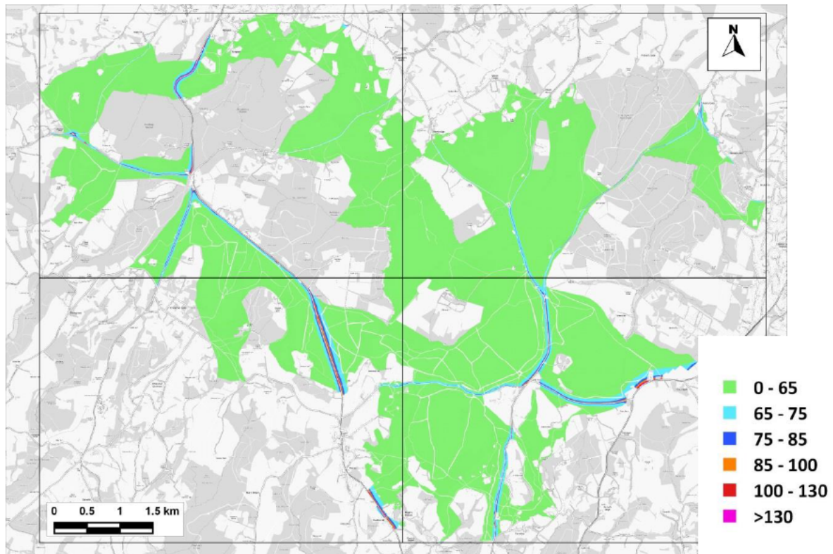
Figure 10.6: Predicted Maximum 24-hour Mean NO x Concentrations across the SAC – 2028 No-Growth - C ( \mu\text{g}/\text{m}^3 )
