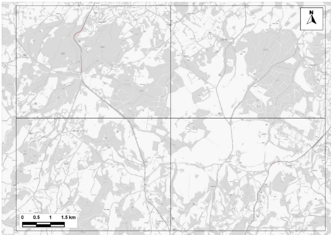
Figure 14.12: Areas in SAC Predicted to Experience an Increase in Annual Mean NO x Concentrations Greater than 1% of the 30 µg/m 3 Critical Level where the Critical Level would also be Exceeded - Comparing 'With Plan' to 'No Growth' Scenarios under Emissions Scenario B
