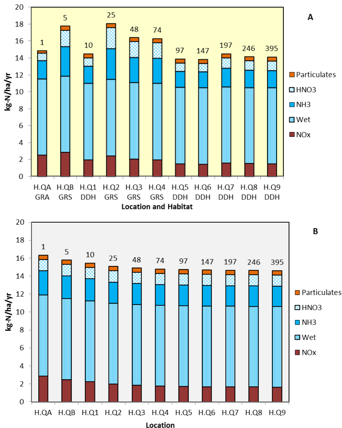
Figure 9.23: Deposition to Ecological Transect H – EA Method – A Using Current Habitat Types and B If all Habitat were Heath (approximate distance from the nearest main road to each quadrant to shown numerically above each column) 36
