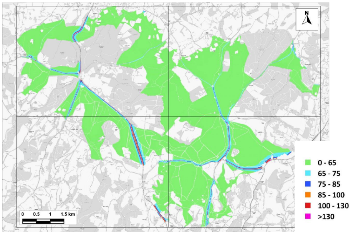
Figure 11.11: Predicted Maximum 24-hour Mean NO x Concentrations across the SAC – 2028 No WDC-Growth - C ( \mu\text{g}/\text{m}^3 )
