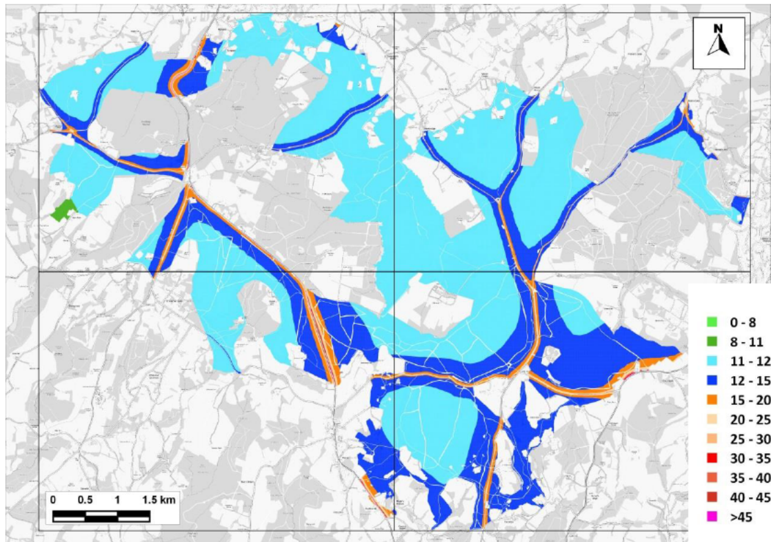
Figure 11.1: Predicted Annual Mean NO x Concentrations across the SAC– 2028 No WDC-Growth - A (µg/m 3 )
