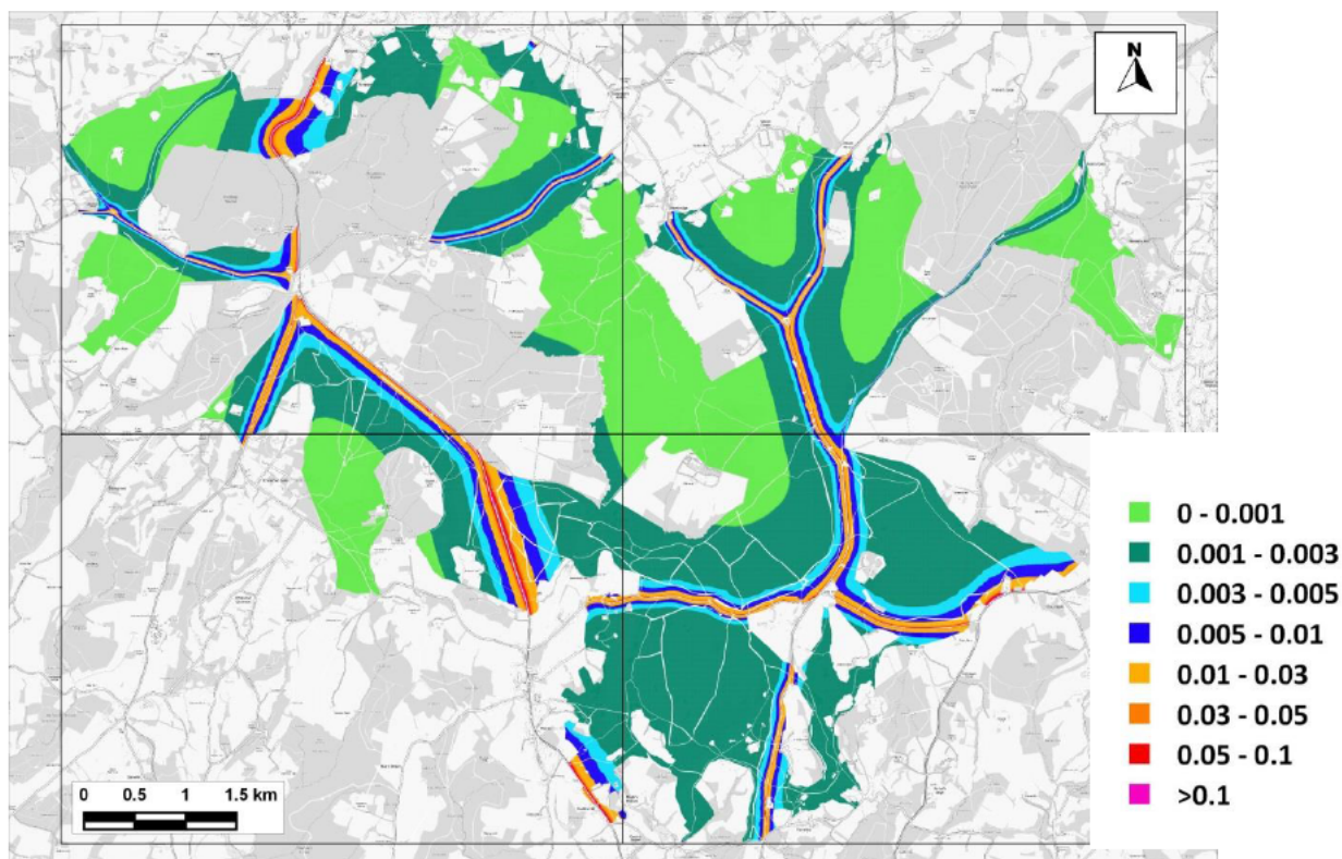
Figure 14.5: Change in Predicted Annual Mean \text{NH}_3 Comparing 'With Plan' to 'No Growth' Scenarios ( \mu\text{g}/\text{m}^3 )
