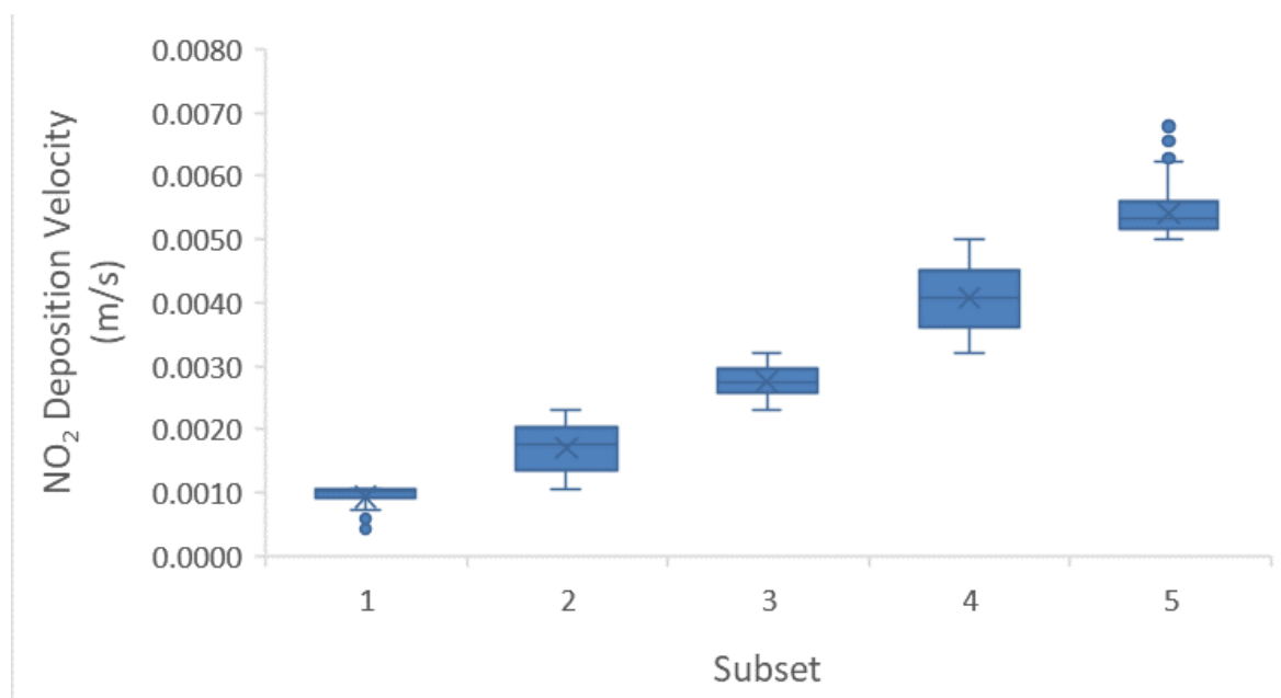
Figure 5.42: Hourly Values of V_d ( \text{NO}_2 ) to Heath During Summer Daytime, separated into Five Subsets
