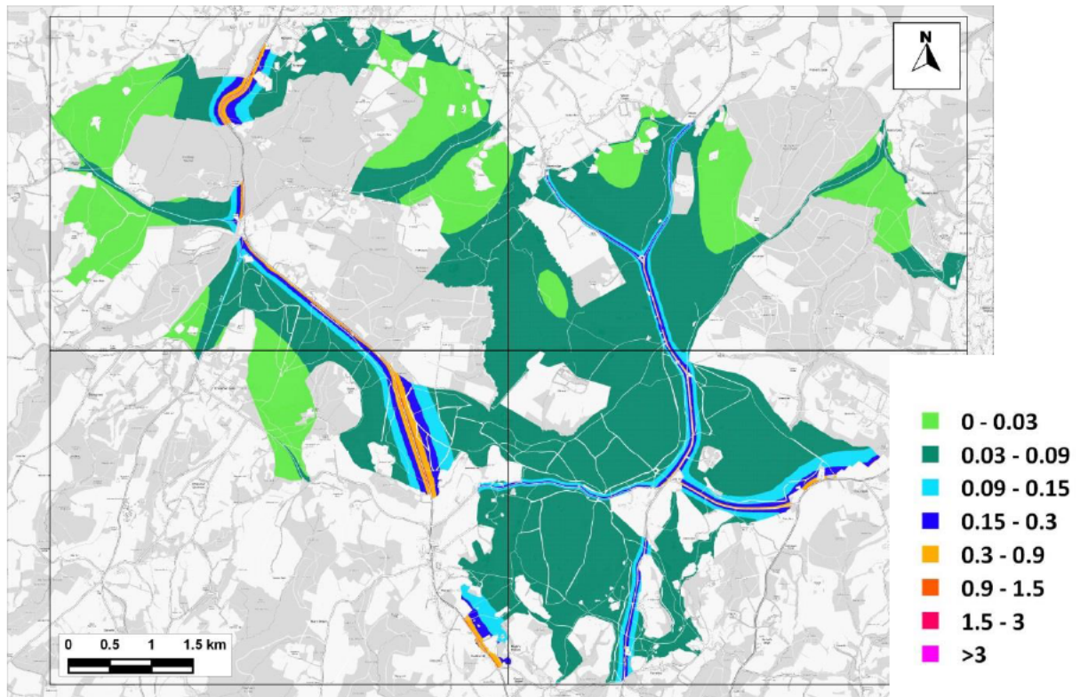
Figure 13.19: Change in Predicted Annual Mean NO x Comparing 'With Plan' to 'No WDC-Growth' Under Emissions Scenario C ( \mu\text{g}/\text{m}^3 )
