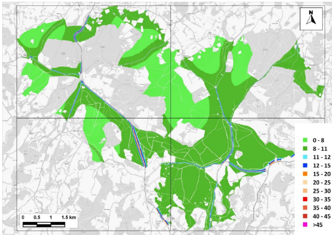
Figure 12.6: Predicted Annual Mean NO x Concentrations across the SAC– 2028 With Plan - B ( \mu\text{g}/\text{m}^3 )
