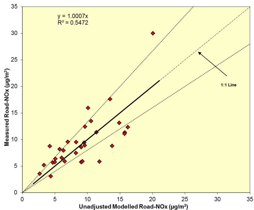
Figure 5.18: Modelled vs Measured Annual Mean Road-NOx, Link Set 2, Iteration 5
