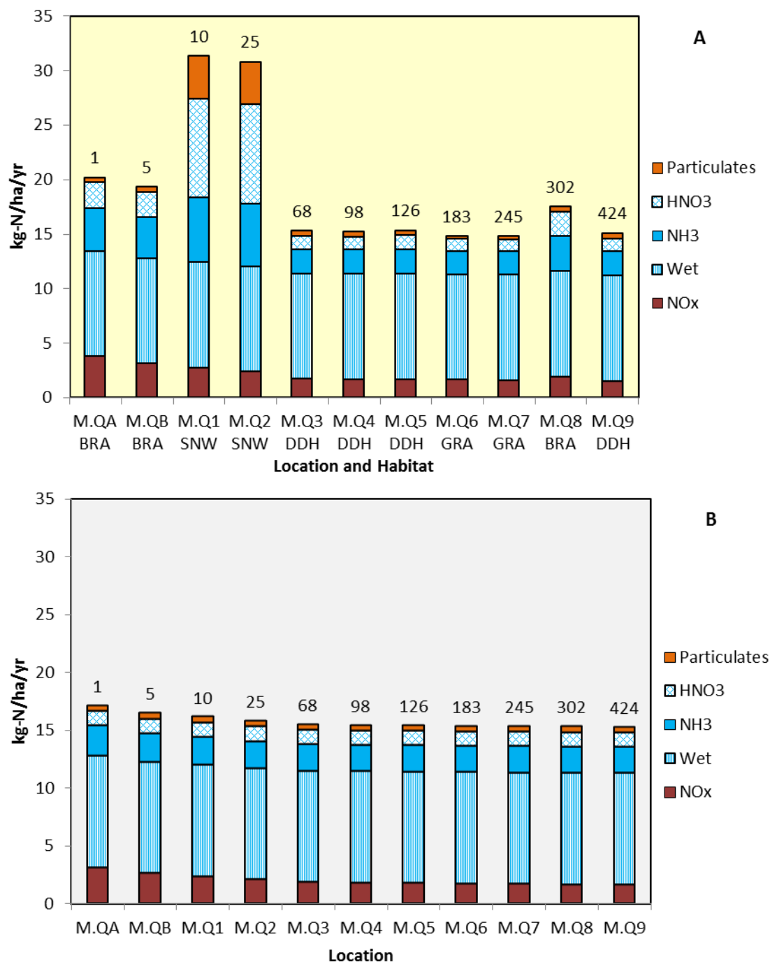
Figure 9.28: Deposition to Ecological Transect M – EA Method – A Using Current Habitat Types and B If all Habitat were Heath (approximate distance from the nearest main road to each quadrant to shown numerically above each column) 36
