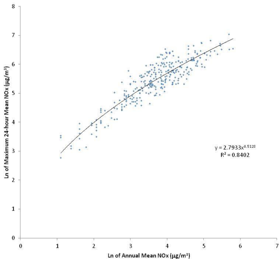
Figure 5.38: Natural Logarithm of Annual Mean NOx vs Maximum 24-hour Mean NOx at all Suitable AURN Sites over 3 Years, Excluding Industrial Sites
