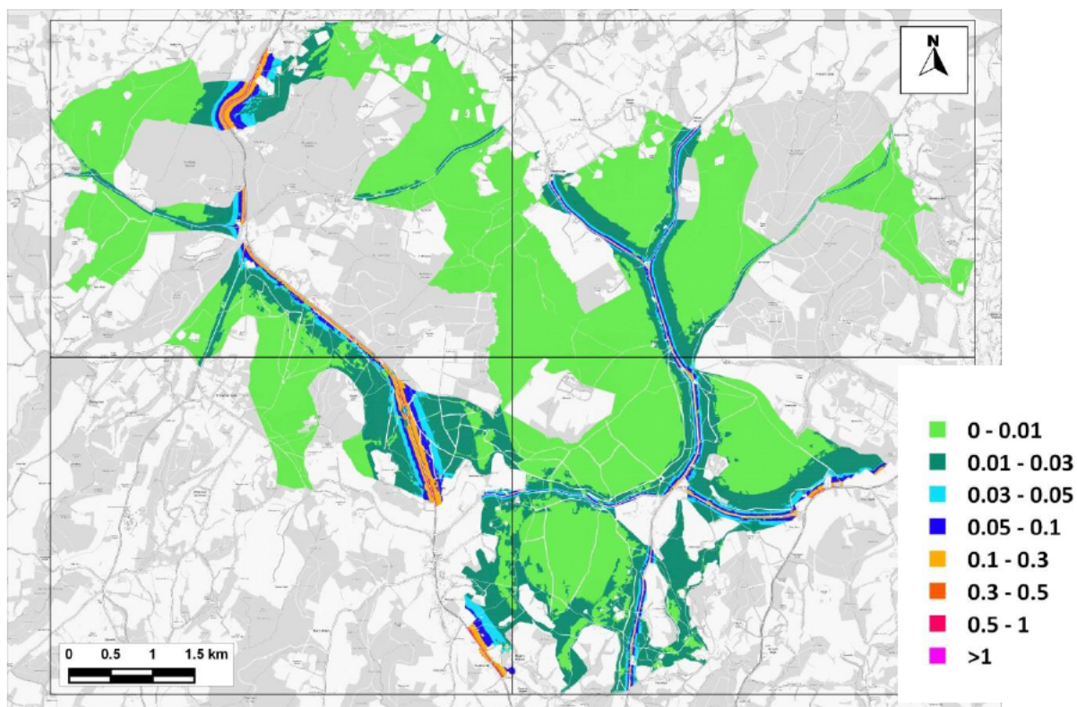
Figure 13.23: Change in Predicted Nitrogen Deposition to SAC Comparing 'With Plan' to 'No WDC-Growth' Under Emission Scenario C (EA Method) (kg-N/ha/yr)
