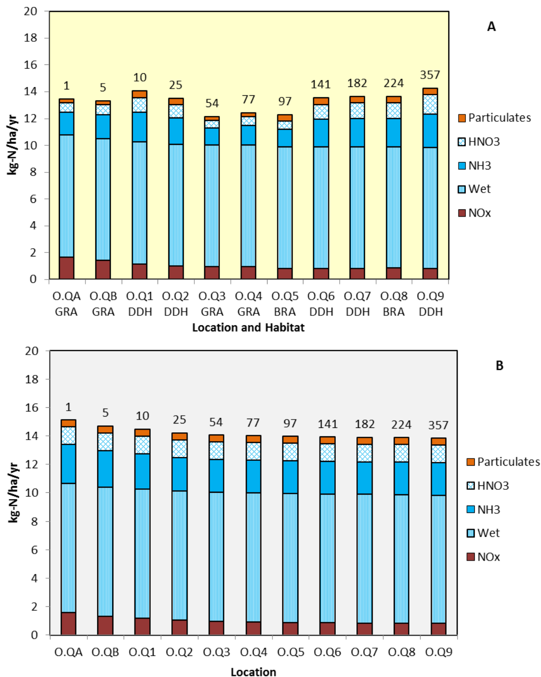
Figure 9.45: Deposition to Ecological Transect O – AQC Method – (A) Using Current Habitat Types and (B) If all Habitat were Heath (approximate distance from the nearest main road to each quadrant to shown numerically above each column) 36
