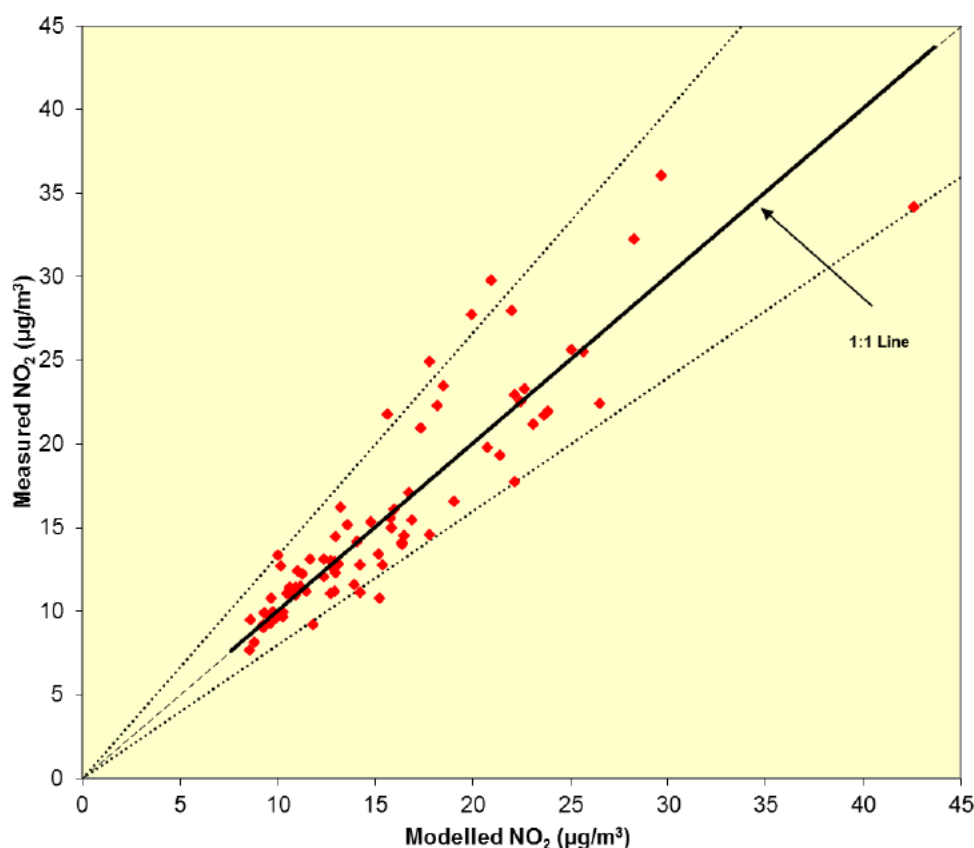
Figure 5.24: Modelled vs Measured Total Annual Mean NO 2 Concentrations following All Adjustments
