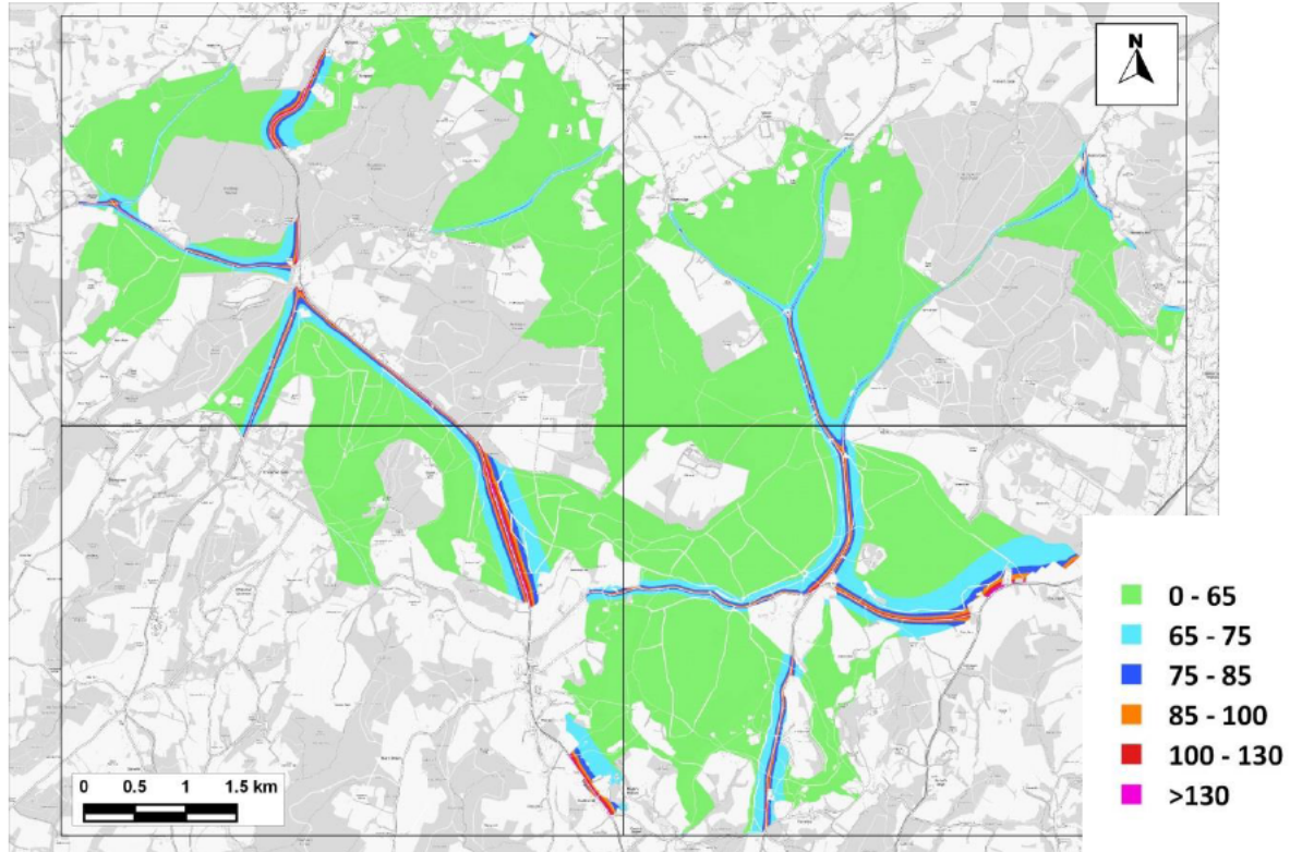
Figure 12.7: Predicted Maximum 24-hour Mean NO x Concentrations across the SAC– 2028 With Plan - B ( \mu\text{g}/\text{m}^3 )
