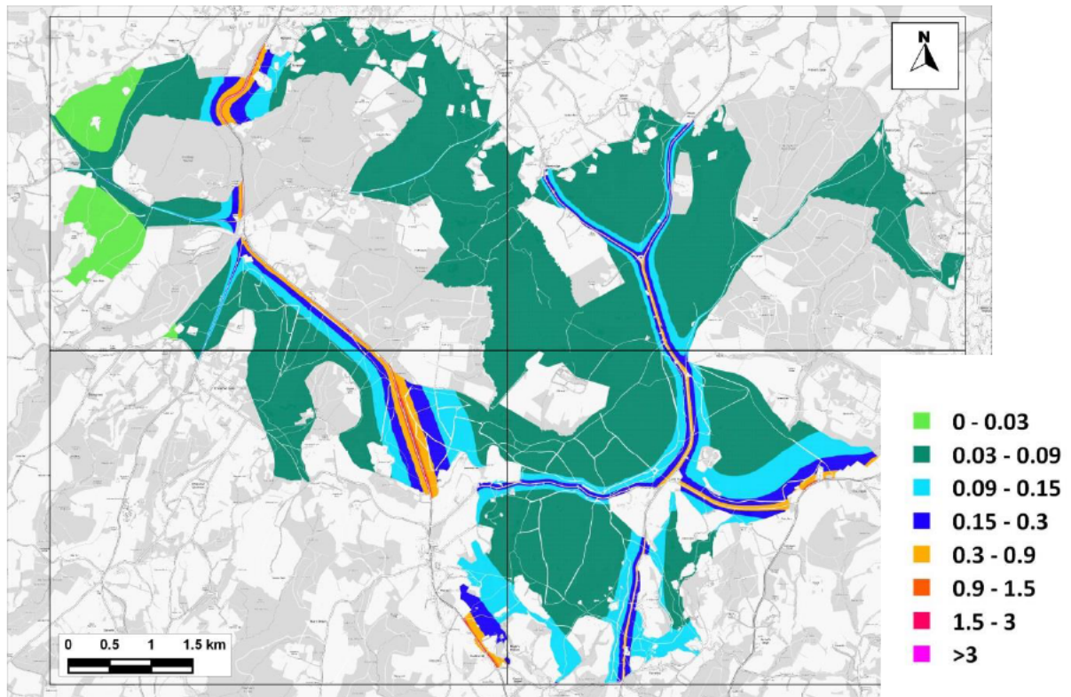
Figure 13.11: Change in Predicted Annual Mean NO x Comparing 'With Plan' to 'No WDC-Growth' Under Emissions Scenario B ( \mu\text{g}/\text{m}^3 )
