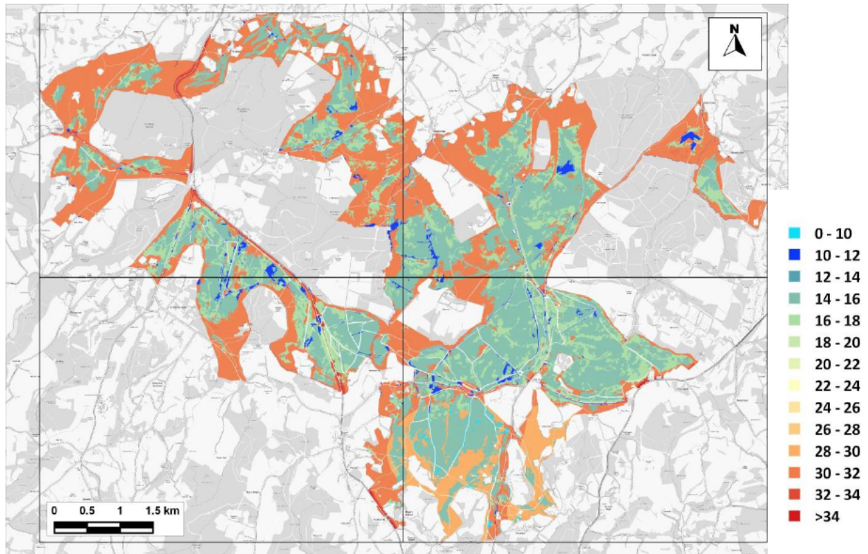
Figure 9.49: Nitrogen Deposition to SAC – Existing Baseline (EA Method) (kg-N/ha/yr)
