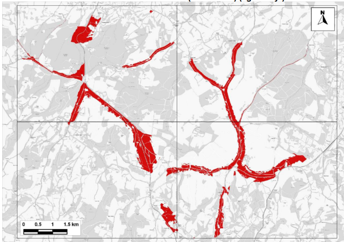
Figure 14.8: Areas in SAC Predicted to Experience an Increase in Nitrogen Deposition Greater than 1% of the 10 kg-N/ha/yr Critical Load where this Critical Load would also be Exceeded - Comparing 'With Plan' to 'No Growth' Scenarios under Emissions Scenario A (EA Method)
