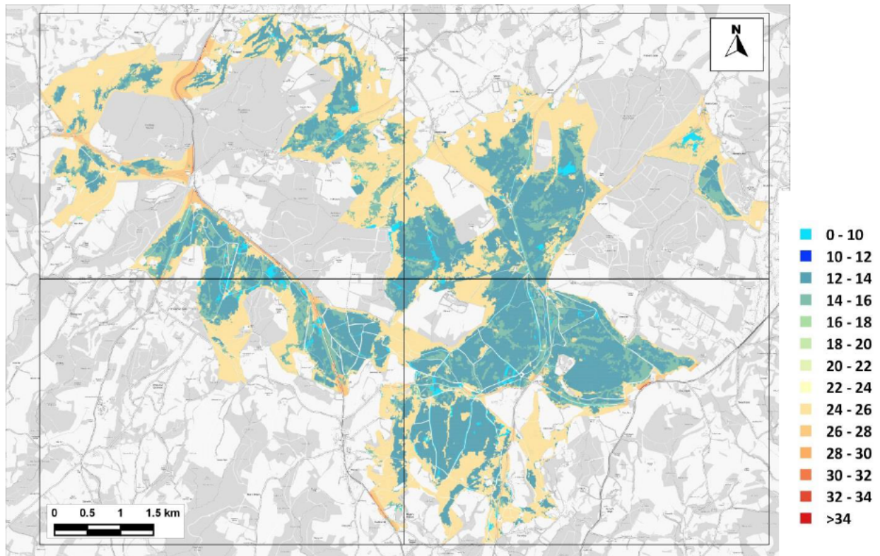
Figure 11.12: Nitrogen Deposition to SAC – 2028 No WDC-Growth - C (EA Method) (kg-N/ha/yr)
