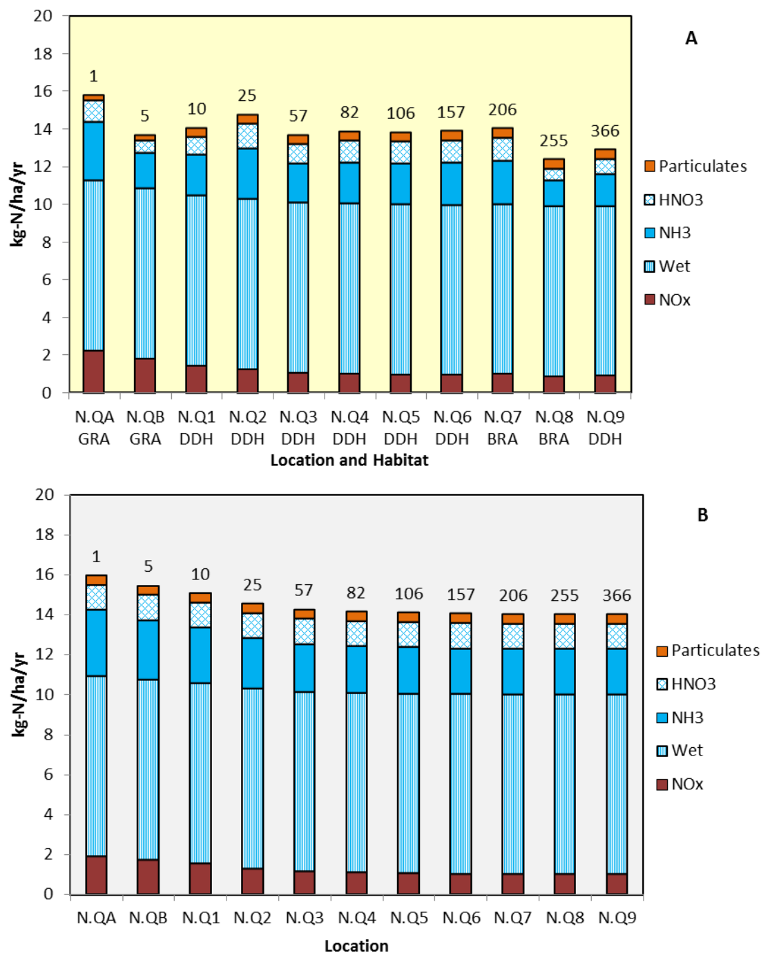
Figure 9.44: Deposition to Ecological Transect N – AQC Method – (A) Using Current Habitat Types and (B) If all Habitat were Heath (approximate distance from the nearest main road to each quadrant to shown numerically above each column) 36
