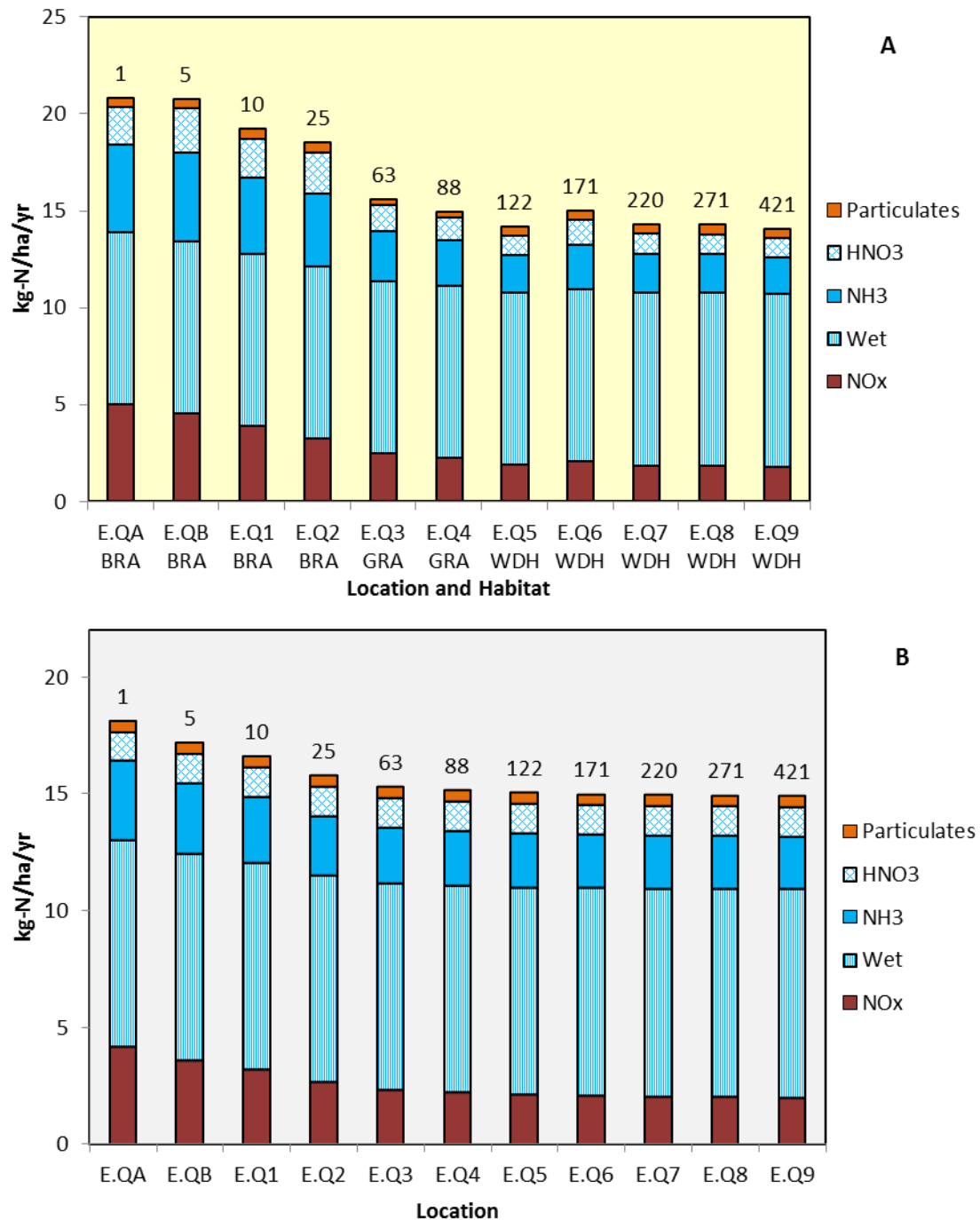
Figure 9.20: Deposition to Ecological Transect E – EA Method – A Using Current Habitat Types and B If all Habitat were Heath (approximate distance from the nearest main road to each quadrant to shown numerically above each column) 36
