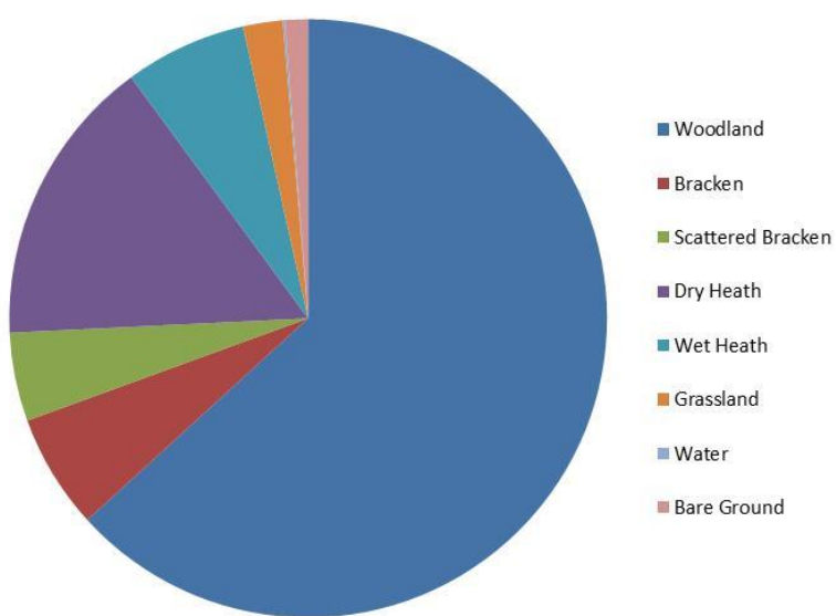
Figure 9.55: Total Nitrogen Deposition to Different Ashdown Forest SAC Land Surfaces (i.e. taking account of relative cover of each land use) (AQC Method)
