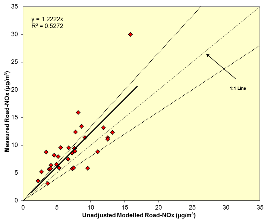
Figure 5.6: Modelled vs Measured Annual Mean Road-NOx, Link Set 2, Iteration 1
