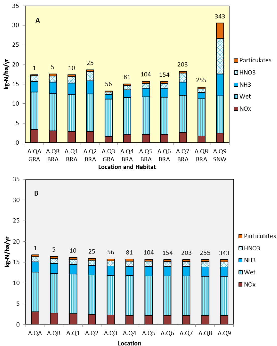
Figure 9.16: Deposition to Ecological Transect A – EA Method – A Using Current Habitat Types and B If all Habitat were Heath (approximate distance from the nearest main road to each quadrant to shown numerically above each column) 36
