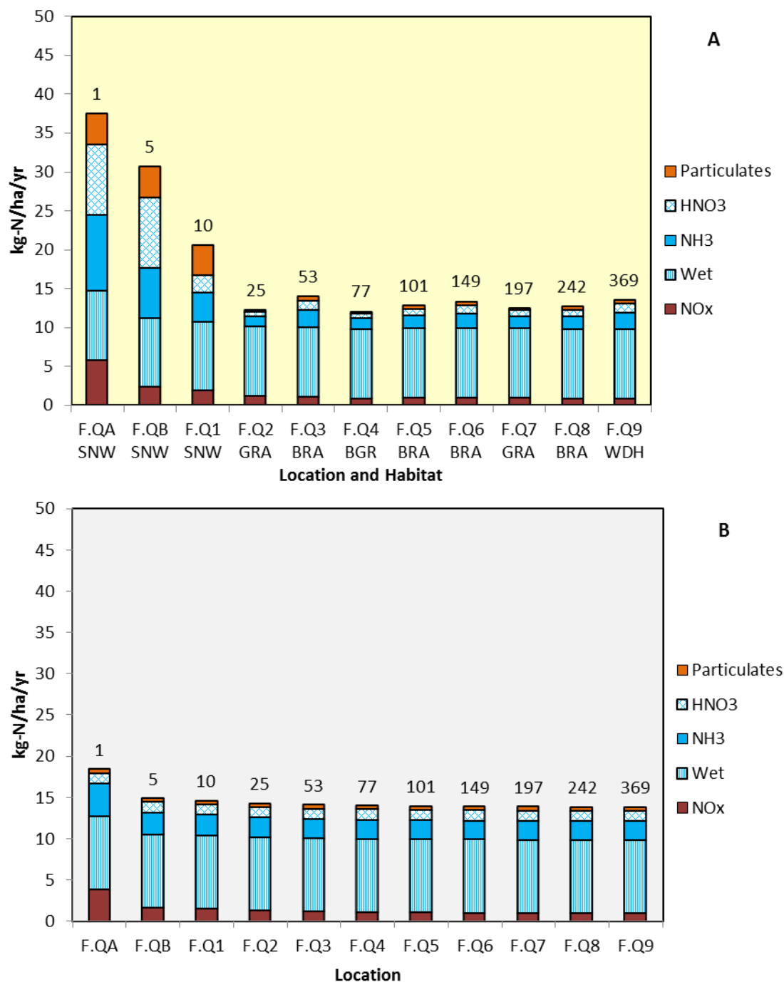
Figure 9.36: Deposition to Ecological Transect F – AQC Method – (A) Using Current Habitat Types and (B) If all Habitat were Heath (approximate distance from the nearest main road to each quadrat to shown numerically above each column) 36,38
