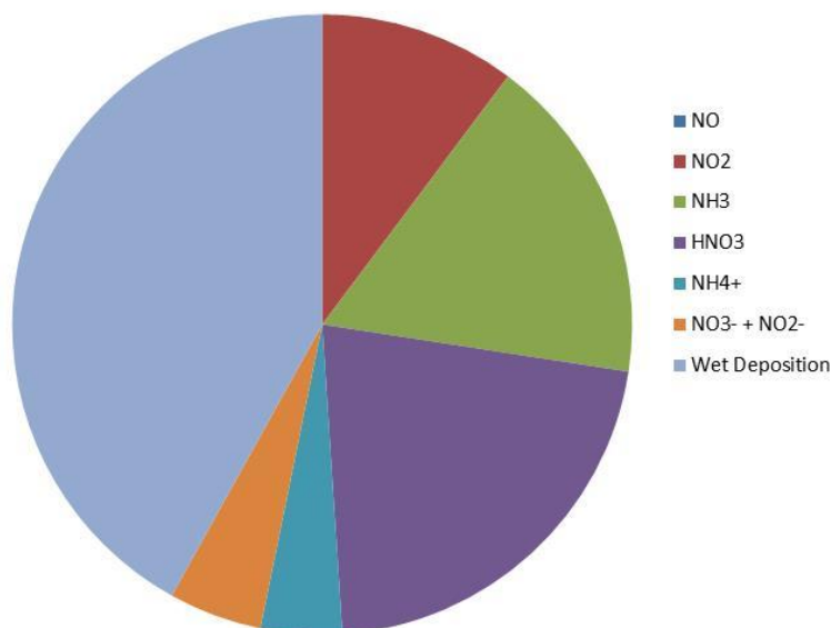
Figure 9.52: Total Nitrogen Deposition to the Ashdown Forest SAC by Pollutant (taking account of relative cover of each land use) (EA Method)
