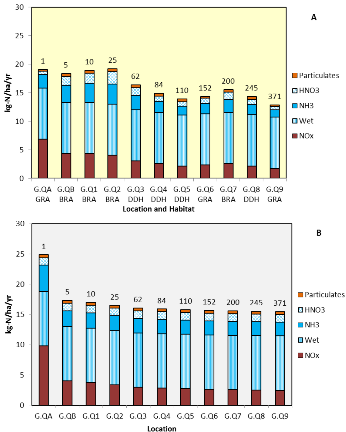
Figure 9.22: Deposition to Ecological Transect G – EA Method – A Using Current Habitat Types and B If all Habitat were Heath (approximate distance from the nearest main road to each quadrant to shown numerically above each column) 36
