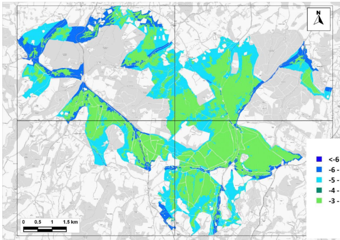
Figure 15.7: Change in Predicted Nitrogen Deposition to SAC Comparing 'With Plan' Emissions Scenario C to 'No Growth' Emission Scenario A (EA Method) (kg-N/ha/yr)
