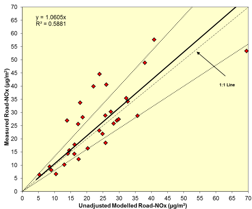
Figure 5.5: Modelled vs Measured Annual Mean Road-NOx, Link Set 1, Iteration 1
