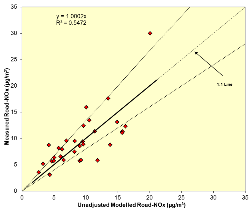
Figure 5.21: Modelled vs Measured Annual Mean Road-NOx, Link Set 2, Iteration 6
