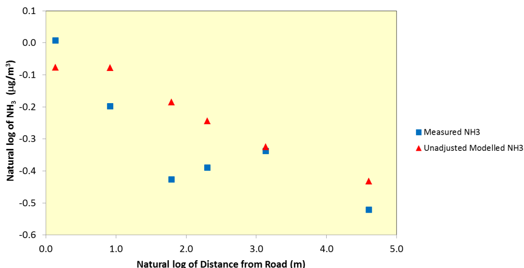
Figure 5.35: Measured vs Predicted 2-Year Average NH 3 Concentrations along Transect 3
