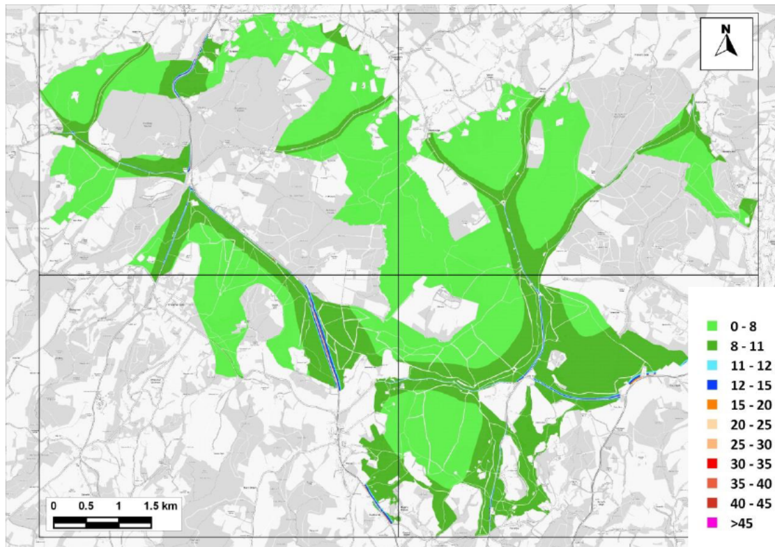
Figure 12.10: Predicted Annual Mean NOx Concentrations across the SAC– 2028 With Plan - C ( \mu\text{g}/\text{m}^3 )
