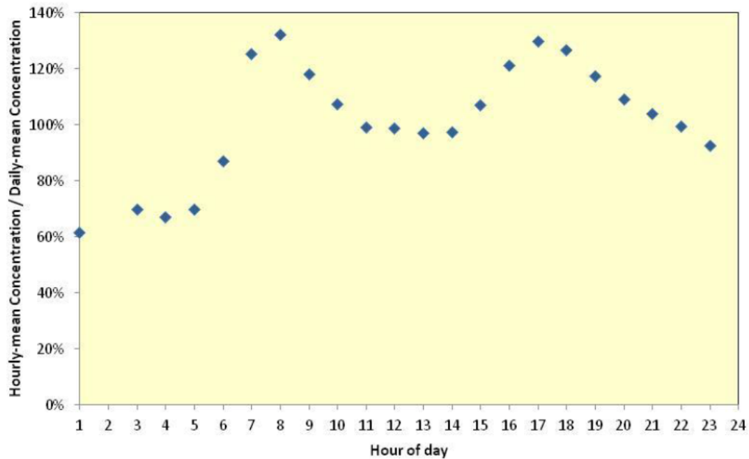
Figure 8.5: Hourly-mean NO 2 / Average Daily-mean NO 2 between October 2014 and August 2016 (GMT) 31
