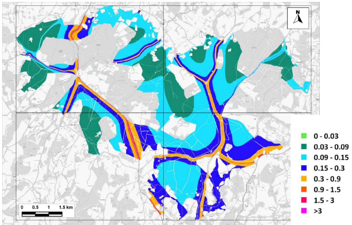
Figure 14.19: Change in Predicted Annual Mean NO x Comparing 'With Plan' to 'No Growth' Under Emissions Scenario C ( \mu\text{g}/\text{m}^3 )
