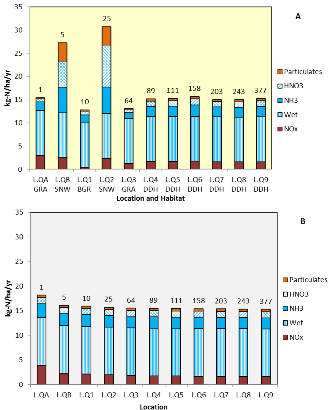
Figure 9.27: Deposition to Ecological Transect L – EA Method – A Using Current Habitat Types and B If all Habitat were Heath (approximate distance from the nearest main road to each quadrant to shown numerically above each column) 36
