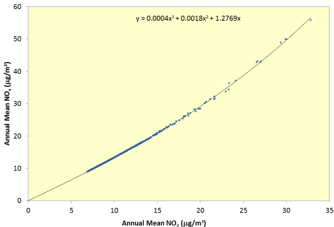
Figure 5.2: Local Background NO x to NO 2 Relationship
