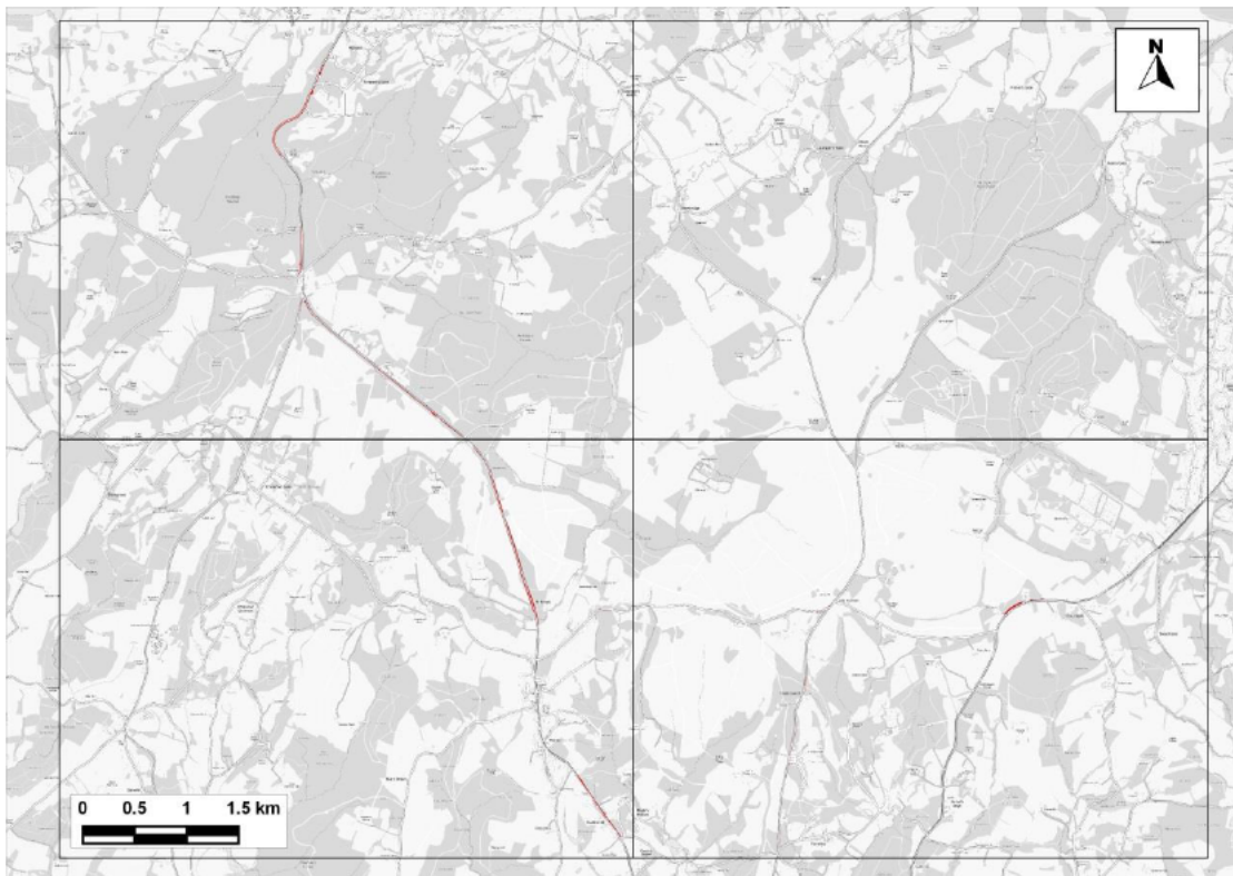
Figure 13.6: Areas in SAC Predicted to Experience an Increase in Annual Mean NH 3 Concentrations Greater than 1% of the 1 µg/m 3 Critical Level where the Critical Level would also be Exceeded (Comparing 'With Plan' to 'No WDC-Growth' Scenarios)
