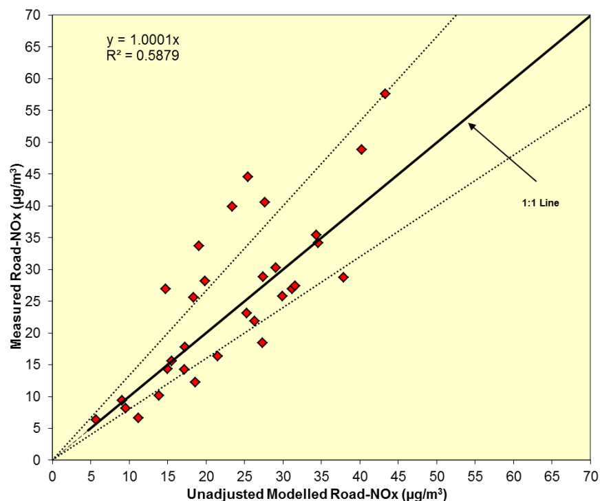
Figure 5.20: Modelled vs Measured Annual Mean Road-NOx, Link Set 1, Iteration 6
