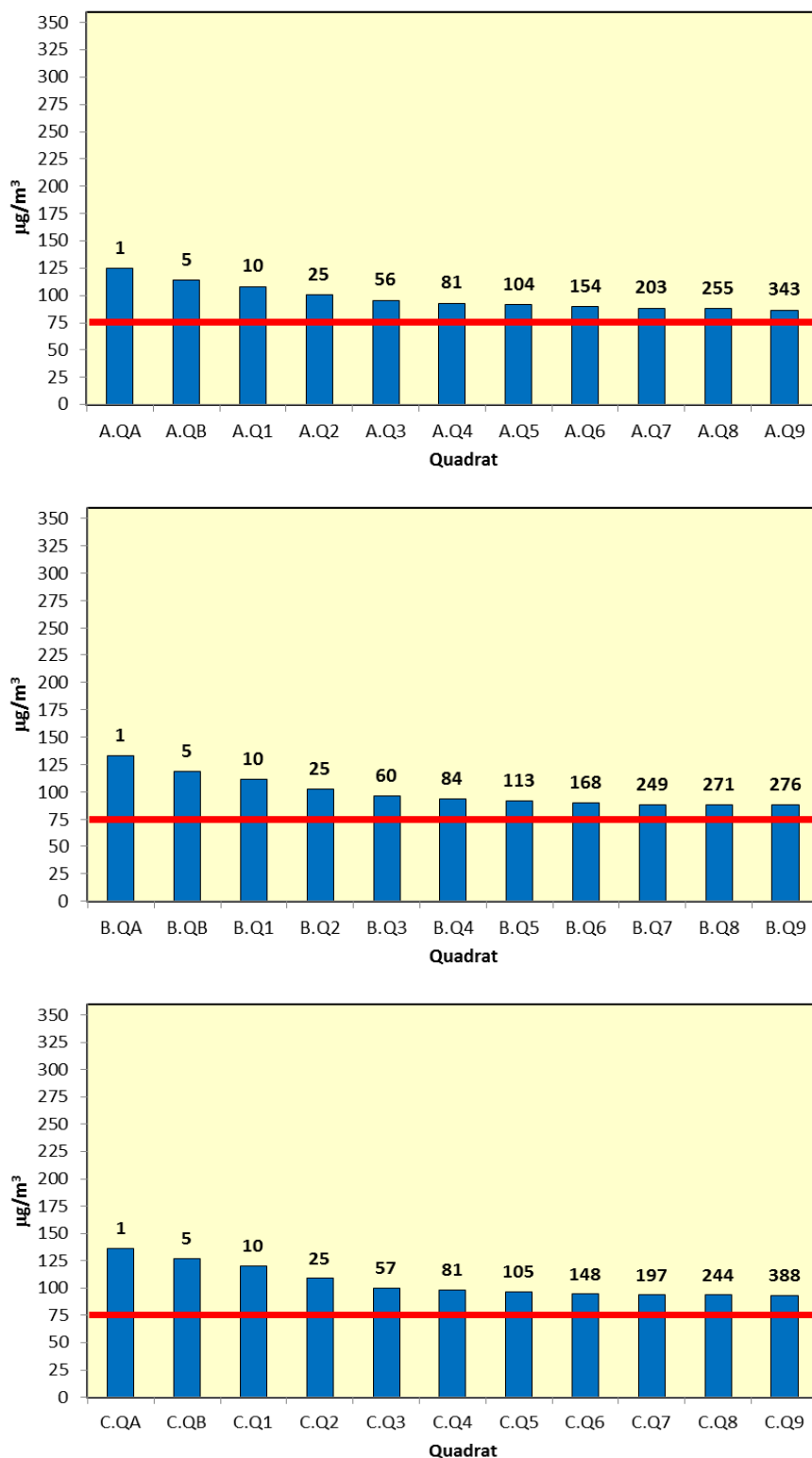
Figure 9.6: Maximum 24-hour Mean NO x Concentrations Along Transects A, B, and C. Approximate distance from the nearest main road to each quadrat to shown numerically above each column. Horizontal line shows the 75 µg/m 3 critical level.
