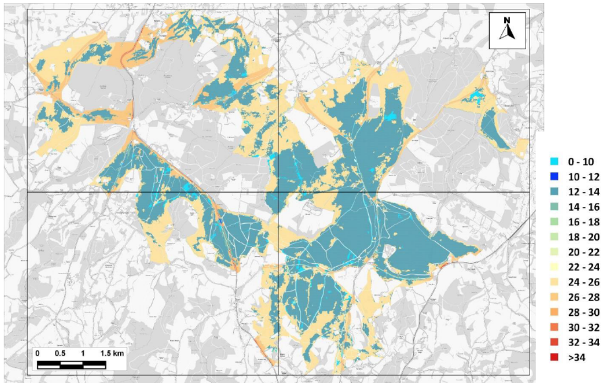
Figure 12.9: Nitrogen Deposition to SAC – 2028 With Plan - B (AQC Method) (kg-N/ha/yr)
