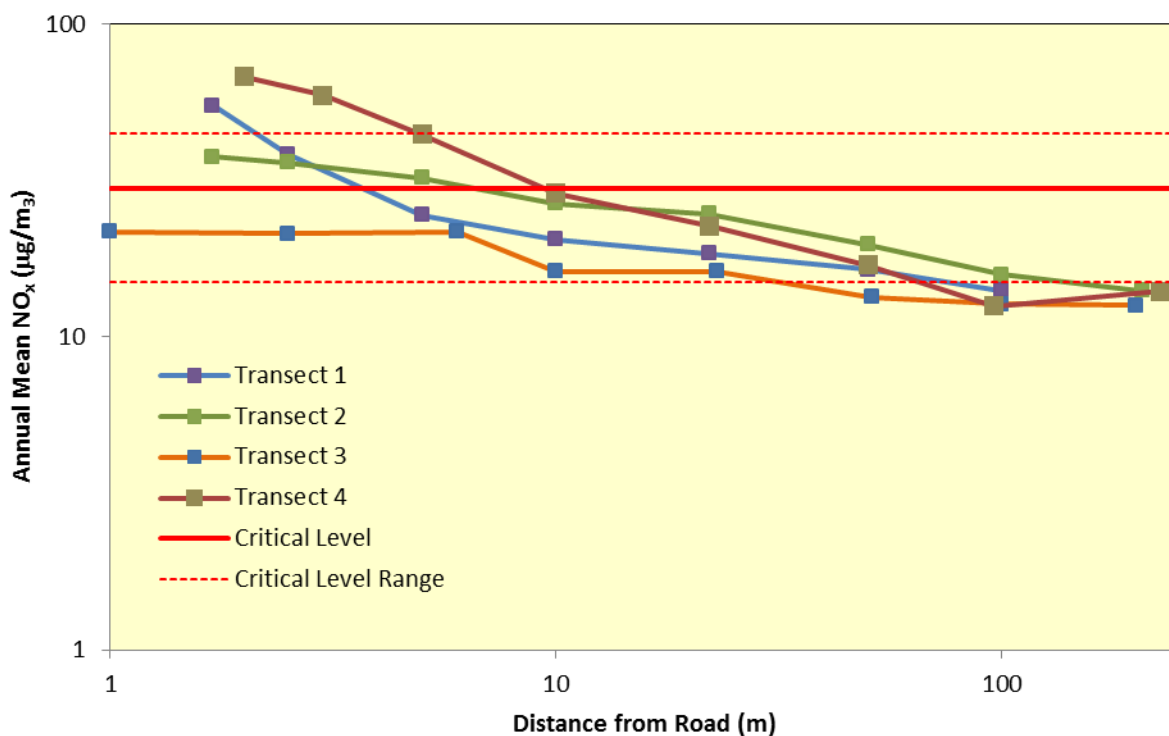
Figure 8.10: Two-year Mean NO x Concentration vs Distance from Roads along the Four Transects on Logarithmic Scales
