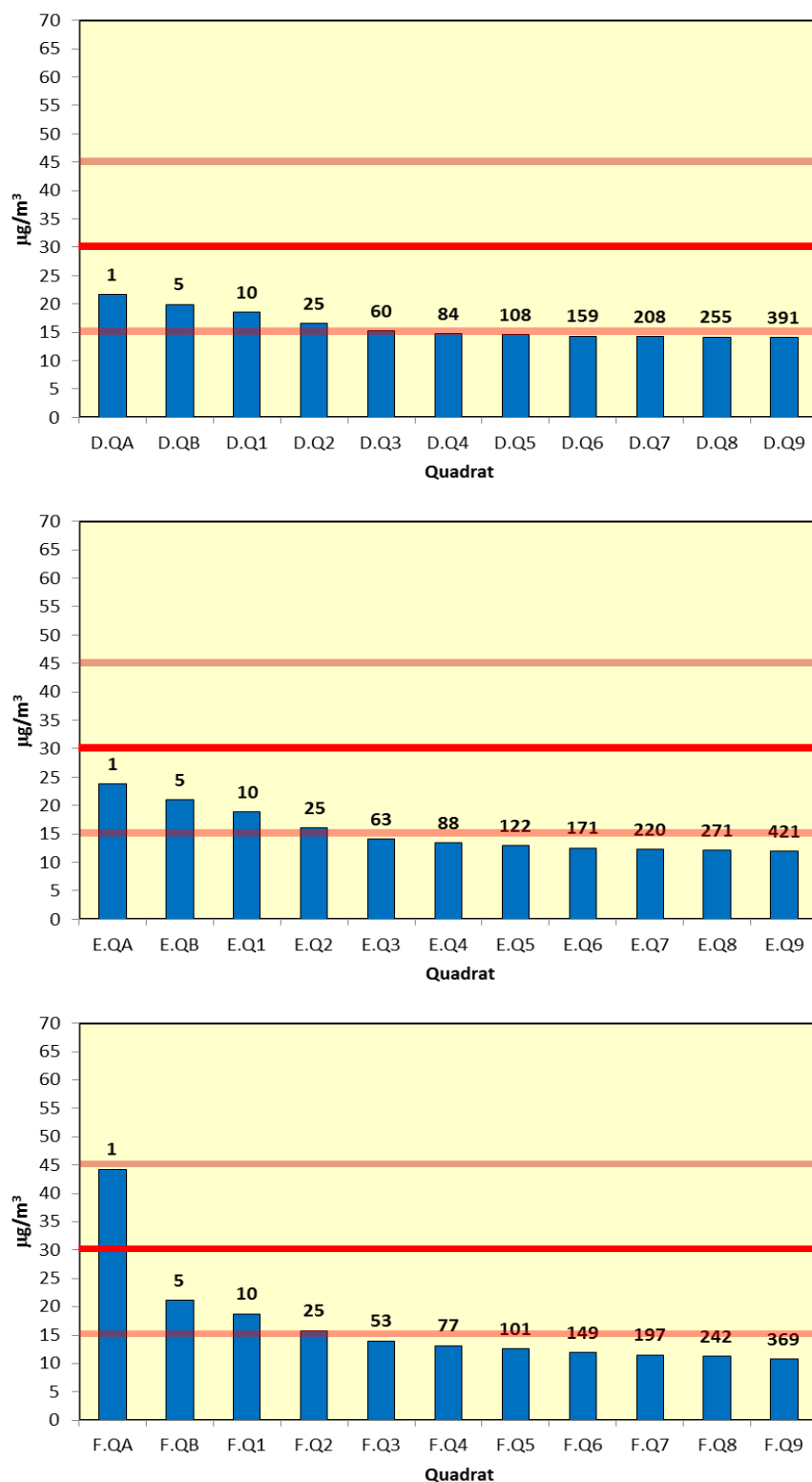
Figure 9.2: Annual Mean NO x Concentrations Along Transects D, E, and F. Approximate distance from the nearest main road to each quadrant to shown numerically above each column. Lines show the 30 µg/m 3 critical level and the 15 µg/m 3 and 45 µg/m 3 critical level range suggested by CEH.
