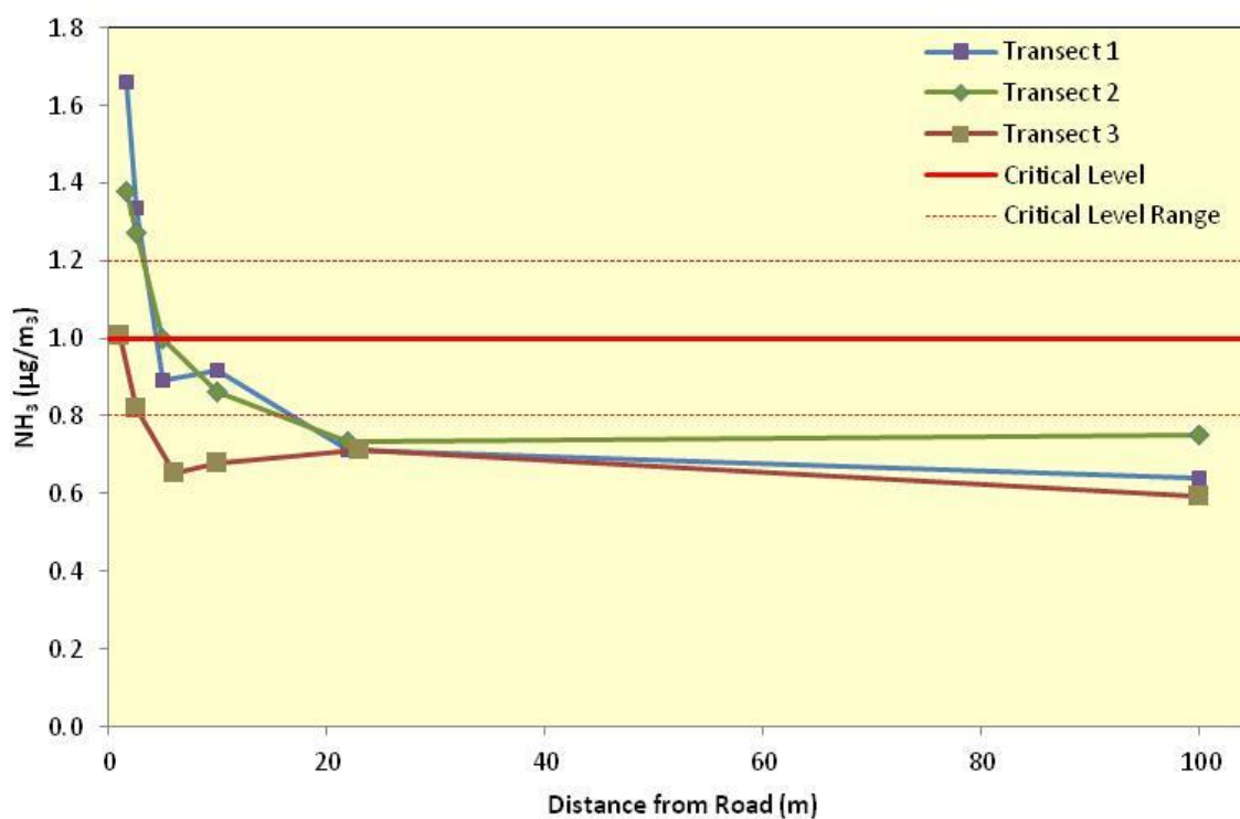
Figure 8.11: Two-year Mean Measured \text{NH}_3 vs Distance from Roads along the Three Transects
