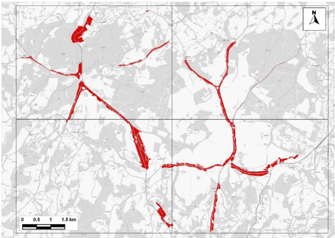
Figure 14.24: Areas in SAC Predicted to Experience an Increase in Nitrogen Deposition Greater than 1% of the 10 kg-N/ha/yr Critical Load where this Critical Load would also be Exceeded - Comparing 'With Plan' to 'No Growth' Scenarios under Emissions Scenario C (EA Method)
