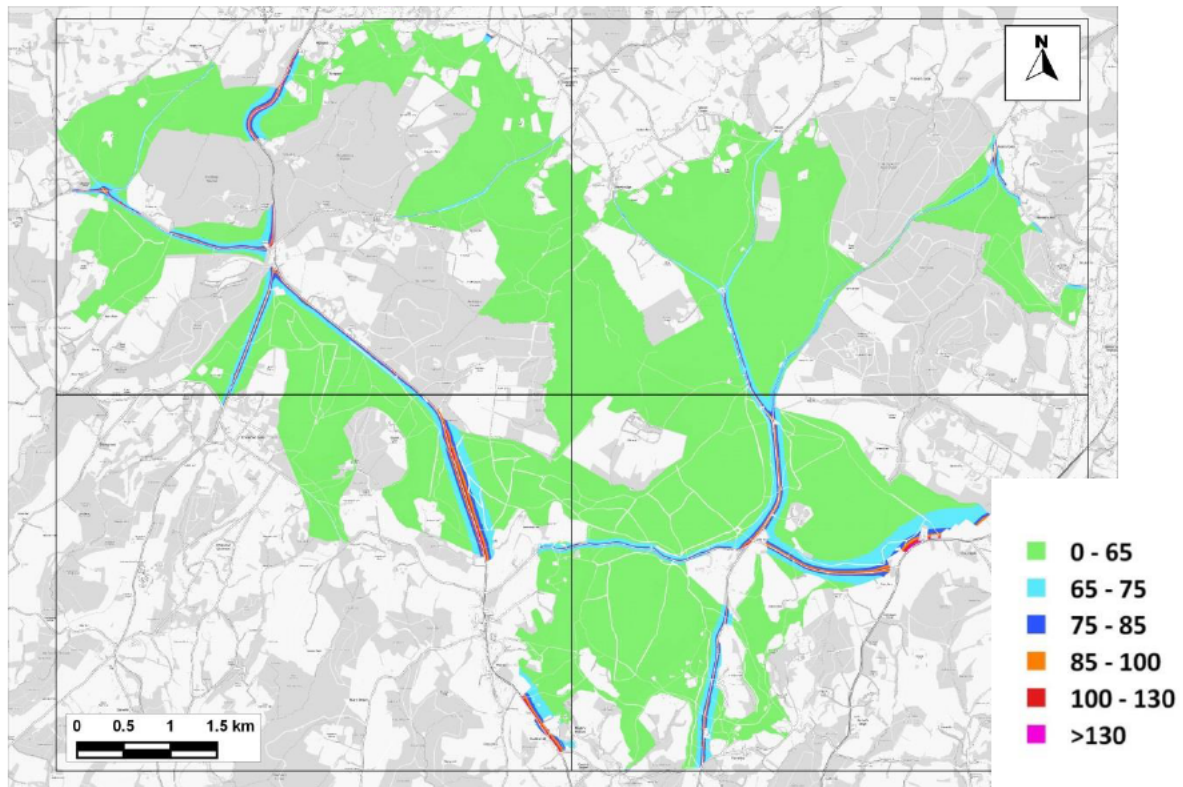
Figure 10.2: Predicted Maximum 24-hour Mean NO x Concentrations across the SAC – 2028 No-Growth - B ( \mu\text{g}/\text{m}^3 )
