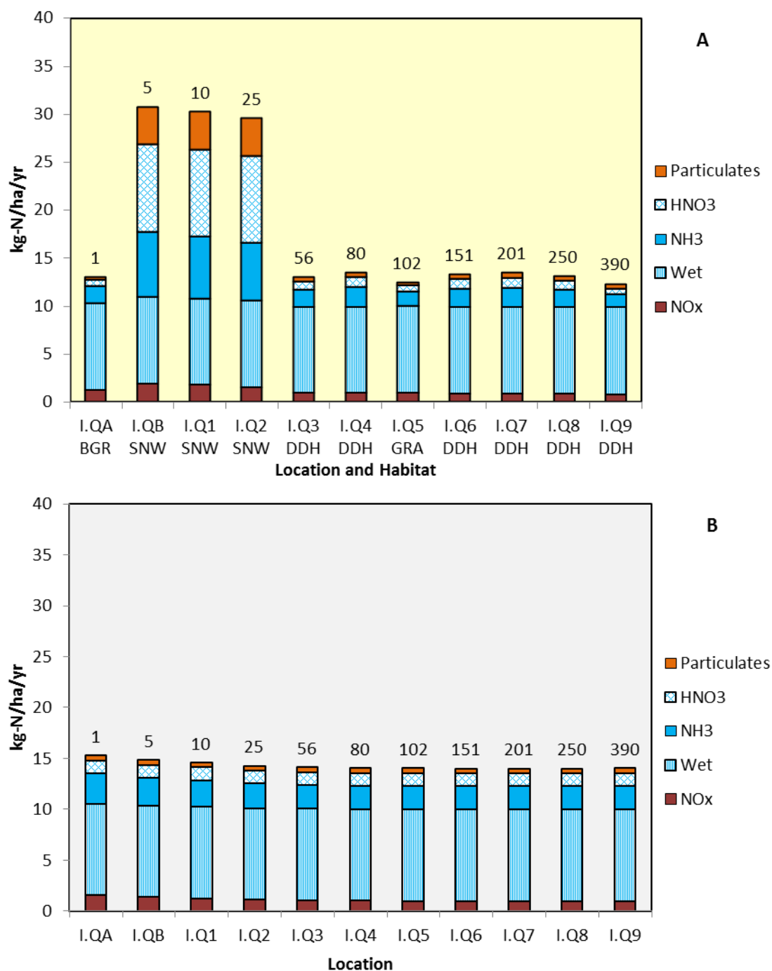
Figure 9.39: Deposition to Ecological Transect I – AQC Method – (A) Using Current Habitat Types and (B) If all Habitat were Heath (approximate distance from the nearest main road to each quadrant to shown numerically above each column) 36
