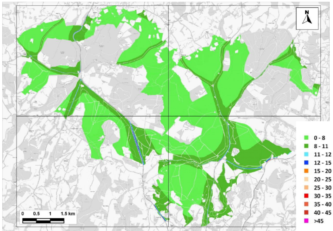
Figure 11.10: Predicted Annual Mean NOx Concentrations across the SAC– 2028 No WDC-Growth - C ( \mu\text{g}/\text{m}^3 )
