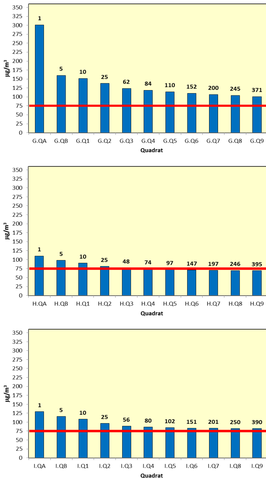
Figure 9.8: Maximum 24-hour Mean NO x Concentrations Along Transects G, H, and I. Approximate distance from the nearest main road to each quadrat to shown numerically above each column. Horizontal line shows the 75 µg/m 3 critical level.
