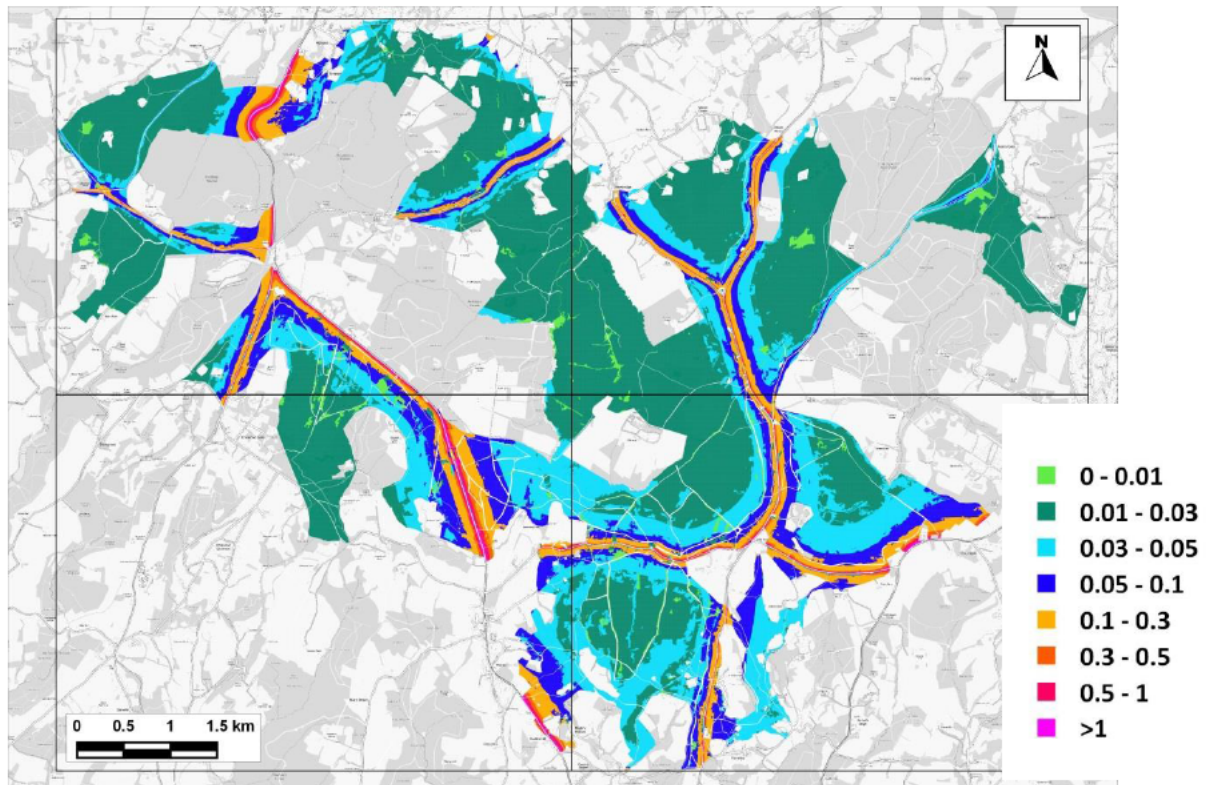
Figure 14.15: Change in Predicted Nitrogen Deposition to SAC Comparing 'With Plan' to 'No Growth' Scenarios Under Emission Scenario B (EA Method) (kg-N/ha/yr)
