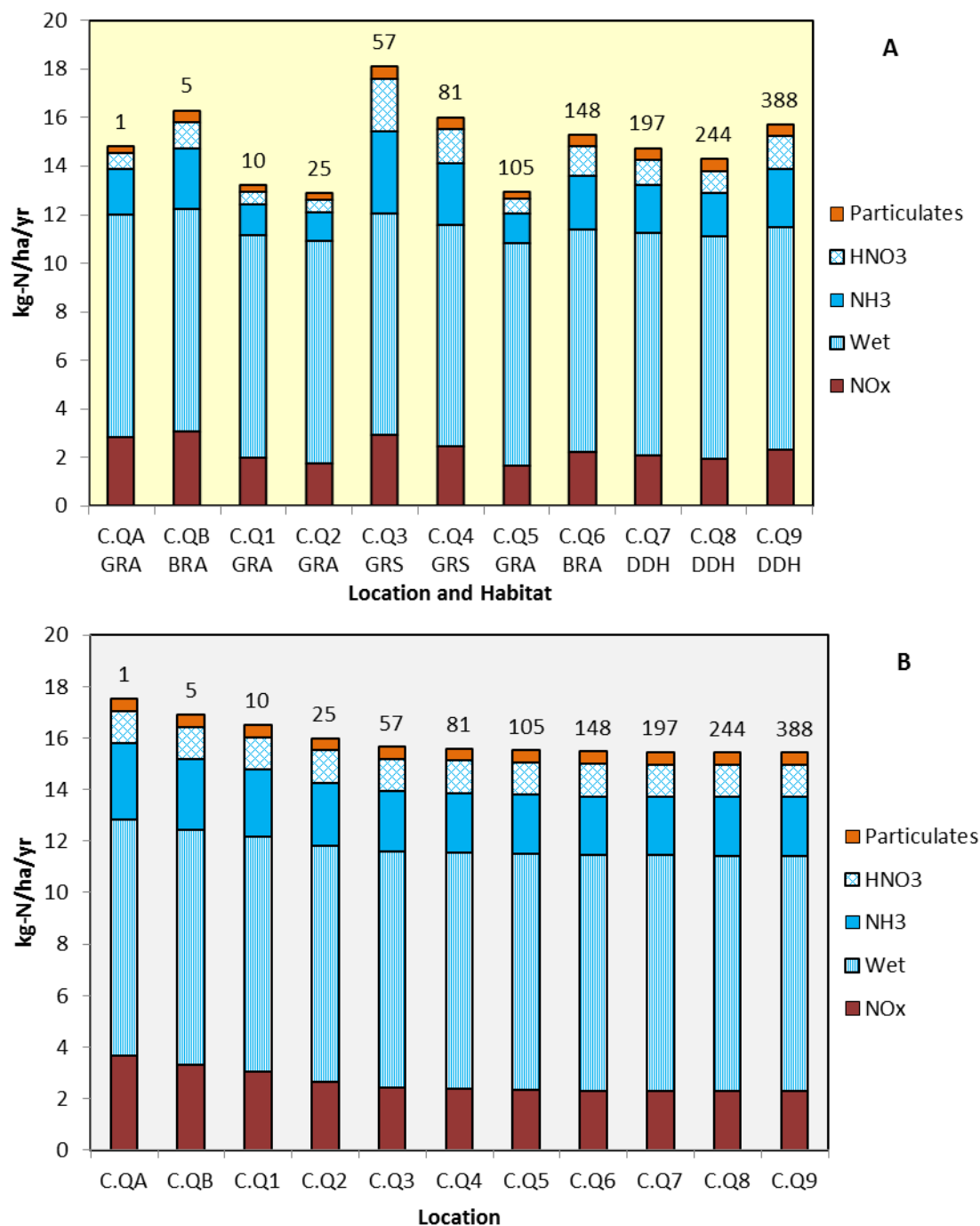
Figure 9.18: Deposition to Ecological Transect C – EA Method – A Using Current Habitat Types and B If all Habitat were Heath (approximate distance from the nearest main road to each quadrant to shown numerically above each column) 36
