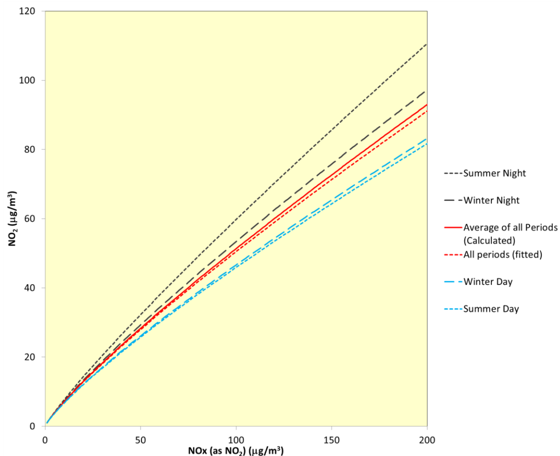
Figure 5.26: Lines of Best-fit for Period-specific NO x to NO 2 Relationships at Eight Automatic Monitoring Sites (four periods) as a Function of the Total NO x Concentration
