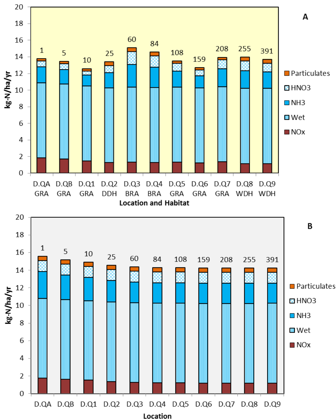
Figure 9.34: Deposition to Ecological Transect D – AQC Method – (A) Using Current Habitat Types and (B) If all Habitat were Heath (approximate distance from the nearest main road to each quadrant to shown numerically above each column) 36
