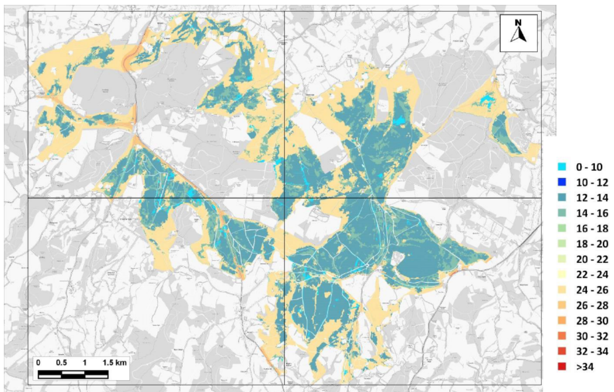
Figure 10.7: Nitrogen Deposition to SAC – 2028 No-Growth - C (EA Method) (kg-N/ha/yr)
