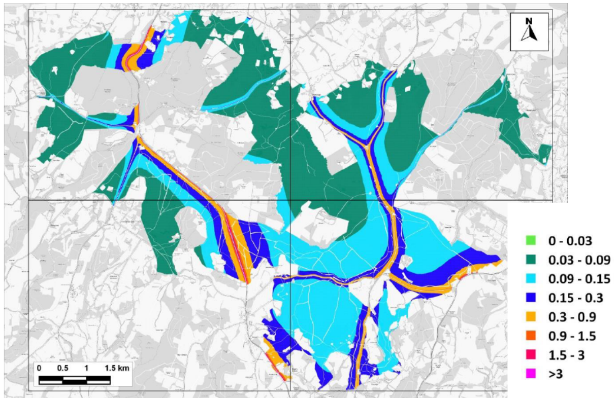
Figure 13.1: Change in Predicted Annual Mean NO x Comparing 'With Plan' to 'No WDC-Growth' Under Emissions Scenario A ( \mu\text{g}/\text{m}^3 )
