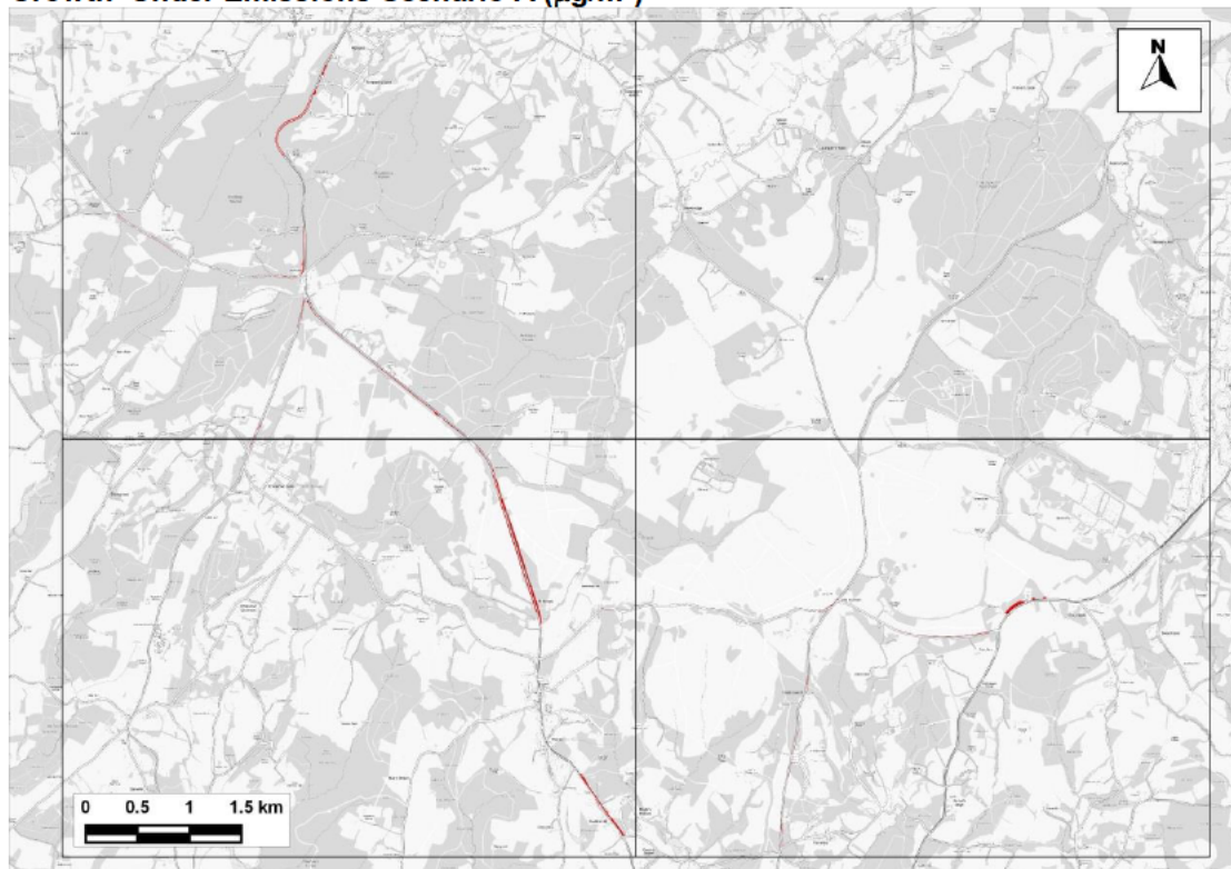
Figure 13.2: Areas in SAC Predicted to Experience an Increase in Annual Mean NO x Concentrations Greater than 1% of the 30 \mu\text{g}/\text{m}^3 Critical Level where the Critical Level would also be Exceeded - Comparing 'With Plan' to 'No WDC-Growth' Scenarios under Emissions Scenario A
