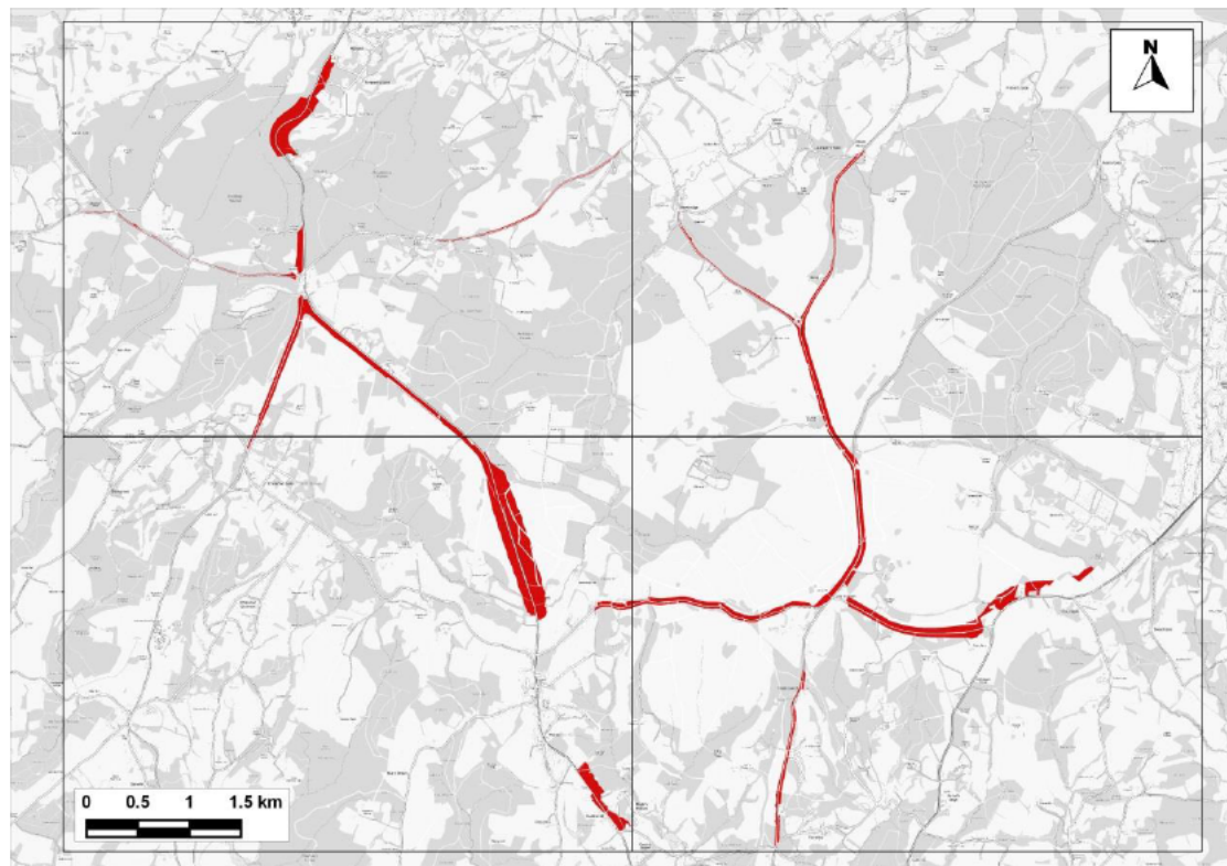
Figure 14.4: Areas in SAC Predicted to Experience an Increase in 24-hour Mean NO x Concentrations Greater than 10% of the 75 \mu\text{g}/\text{m}^3 Critical Level where the Critical Level would also be Exceeded - Comparing 'With Plan' to 'No Growth' Scenarios under Emissions Scenario A
