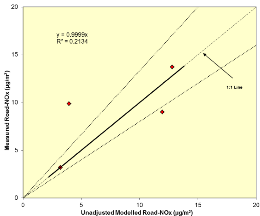
Figure 5.19: Modelled vs Measured Annual Mean Road-NOx, Link Set 3, Iteration 5
