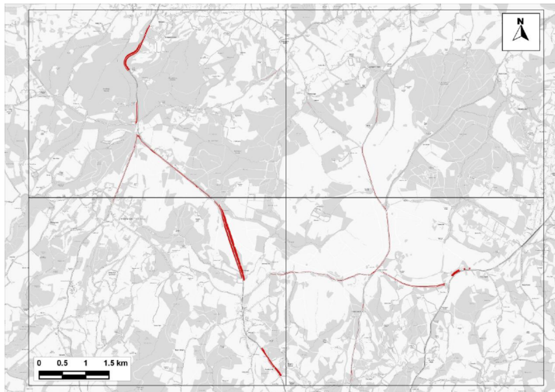
Figure 14.22: Areas in SAC Predicted to Experience an Increase in 24-hour Mean NO x Concentrations Greater than 10% of the 75 \mu\text{g}/\text{m}^3 Critical Level where the Critical Level would also be Exceeded - Comparing 'With Plan' to 'No Growth' Scenarios under Emissions Scenario C
