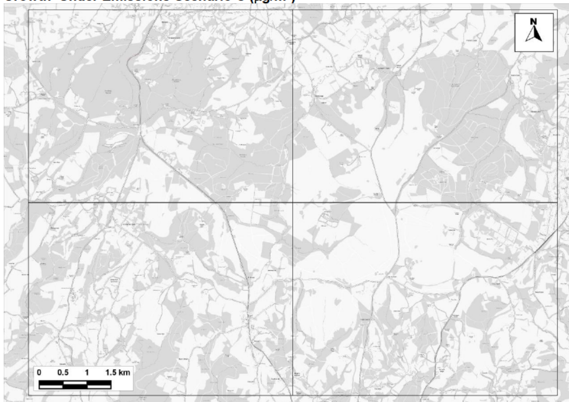
Figure 13.20: Areas in SAC Predicted to Experience an Increase in Annual Mean NO x Concentrations Greater than 1% of the 30 \mu\text{g}/\text{m}^3 Critical Level where the Critical Level would also be Exceeded - Comparing 'With Plan' to 'No WDC-Growth' Scenarios under Emissions Scenario C
