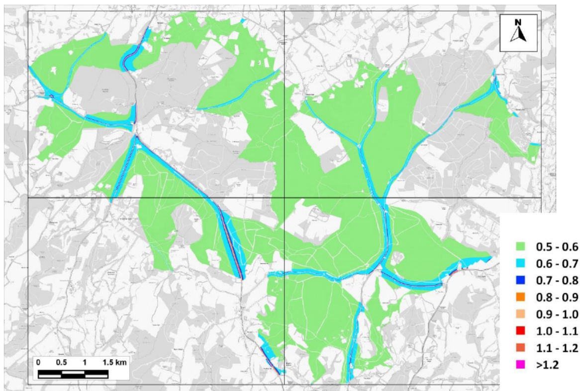
Figure 9.48: Predicted Annual Mean \text{NH}_3 Concentrations across the SAC– Existing Baseline ( \mu\text{g}/\text{m}^3 )
