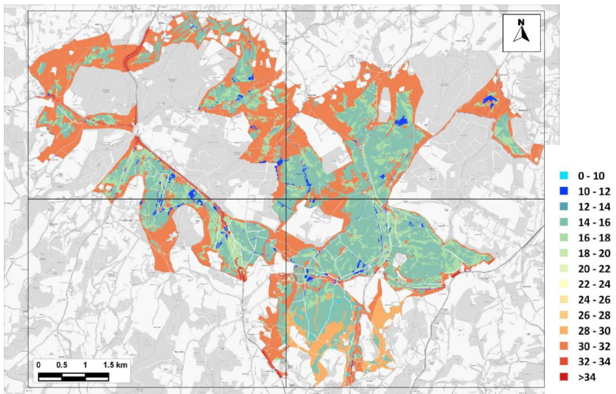
Figure 11.4: Nitrogen Deposition to SAC – 2028 No WDC-Growth - A (EA Method) (kg-N/ha/yr)
