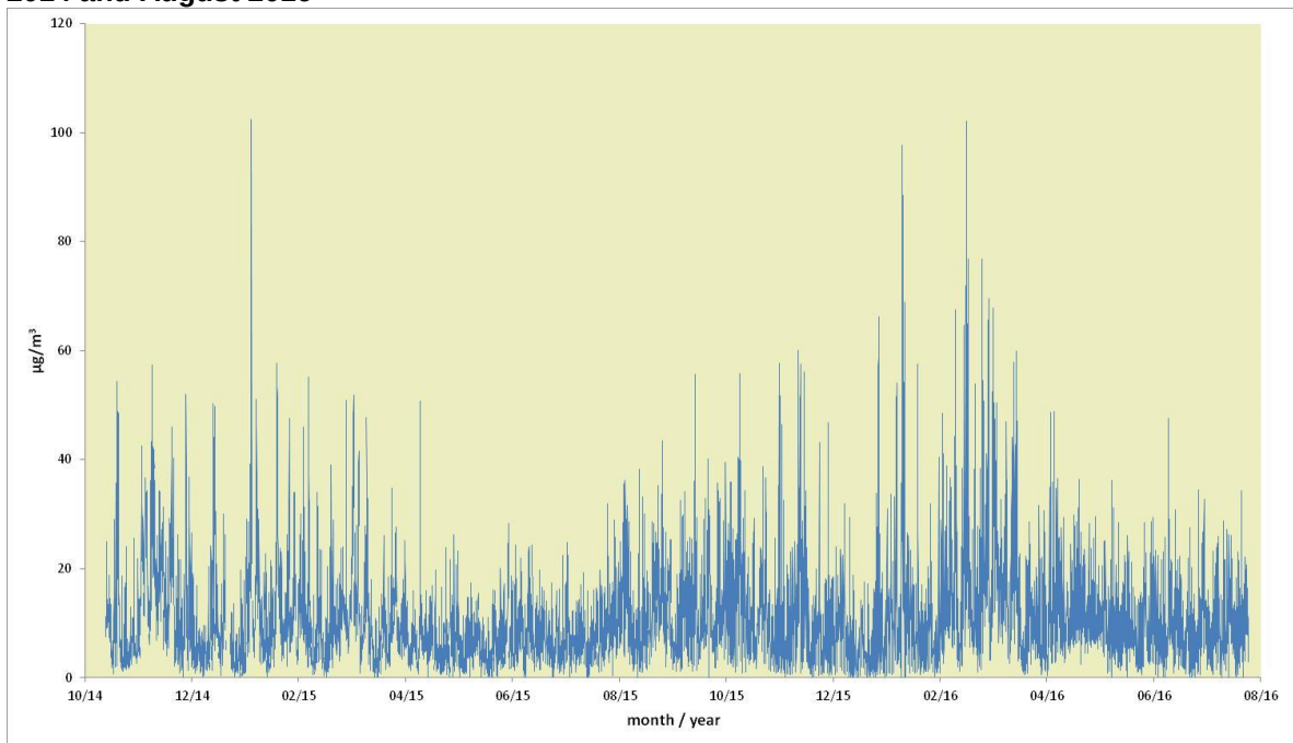
Figure 8.2: 1-hour Mean Nitrogen Dioxide Concentrations at Kingstanding between October 2014 and August 2016
