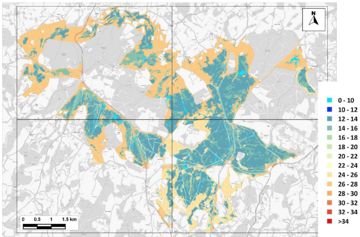
Figure 10.3: Nitrogen Deposition to SAC – 2028 No-Growth - B (EA Method) (kg-N/ha/yr)
