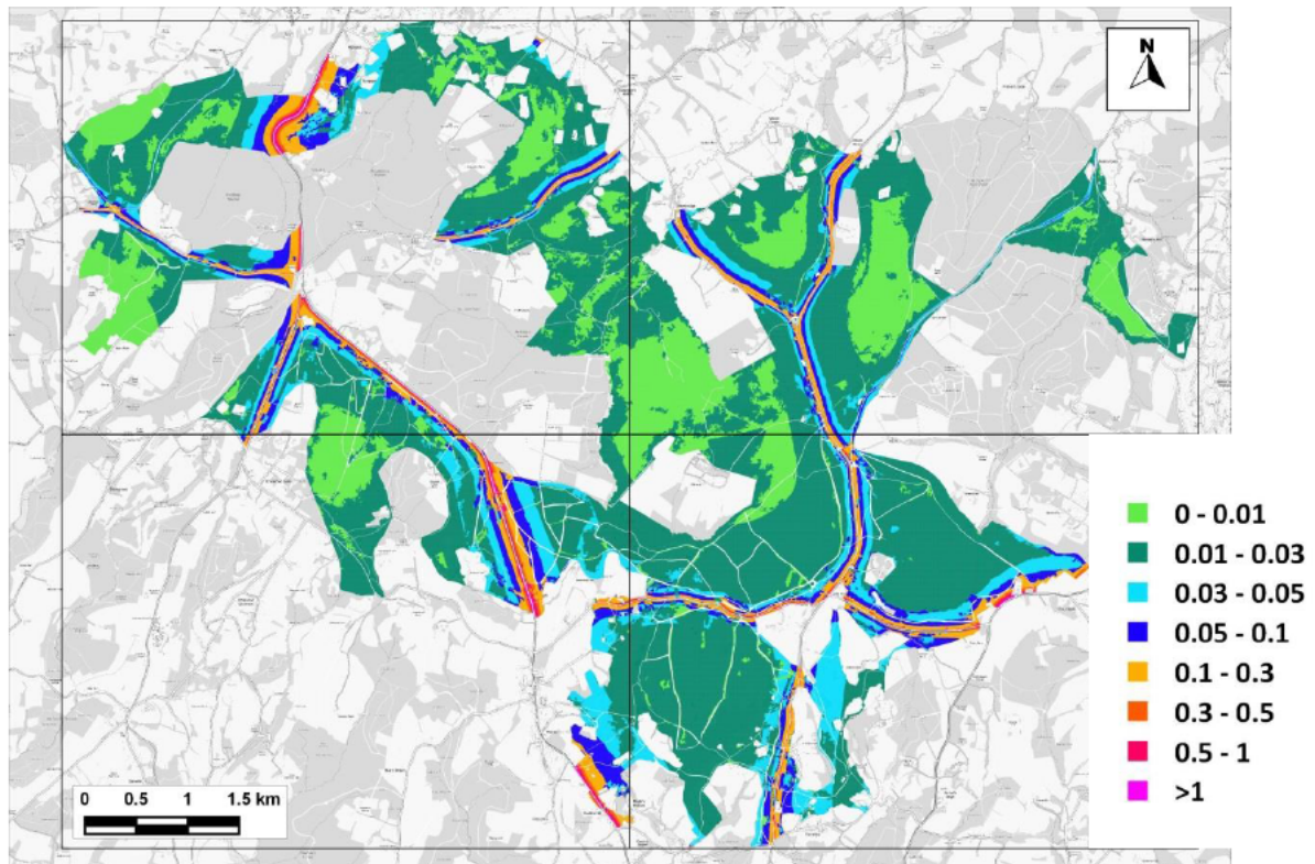
Figure 14.25: Change in Predicted Nitrogen Deposition to SAC Comparing 'With Plan' to 'No Growth' Scenarios under Emissions Scenario C (AQC Method) (kg-N/ha/yr)
