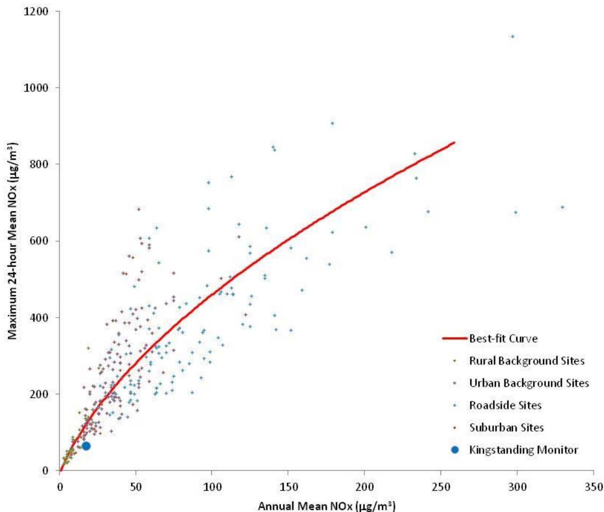
Figure 5.39: Annual Mean NOx vs Maximum 24-hour Mean NOx at all Suitable AURN Sites over 3 Years, also Showing Kingstanding Site and Best-fit Curve. The Best-fit Curve is that shown in Figure 5.37, which is on a logarithmic scale. It can be described as: \text{Exp}(2.7924 \times \text{Ln}(X)^{0.5149})
