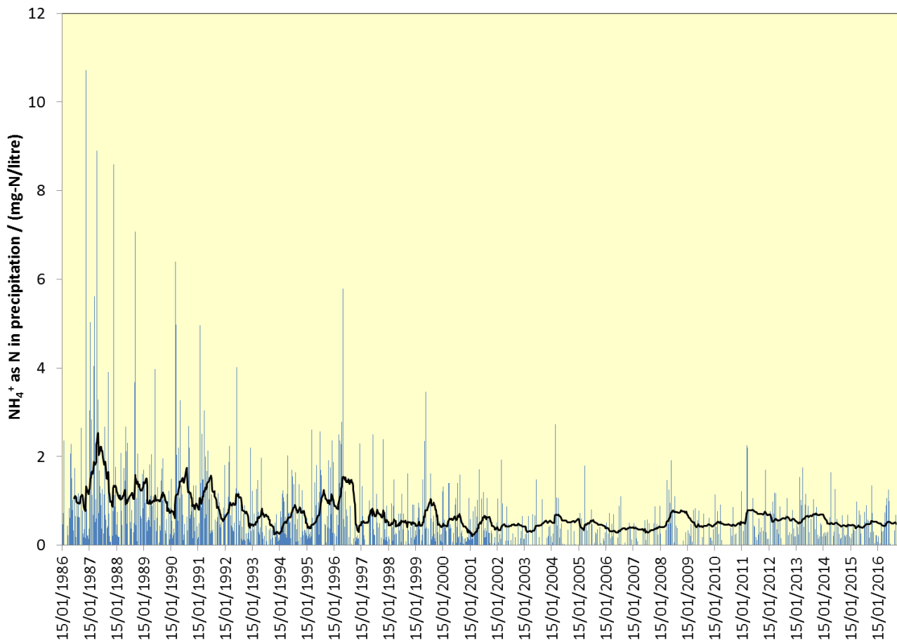
Figure 3.3: \text{NH}_4^+ in Precipitation Measured at Barcombe Mills over 30 Years (blue line) and 24-month rolling average (black line) (mg-N/litre)
