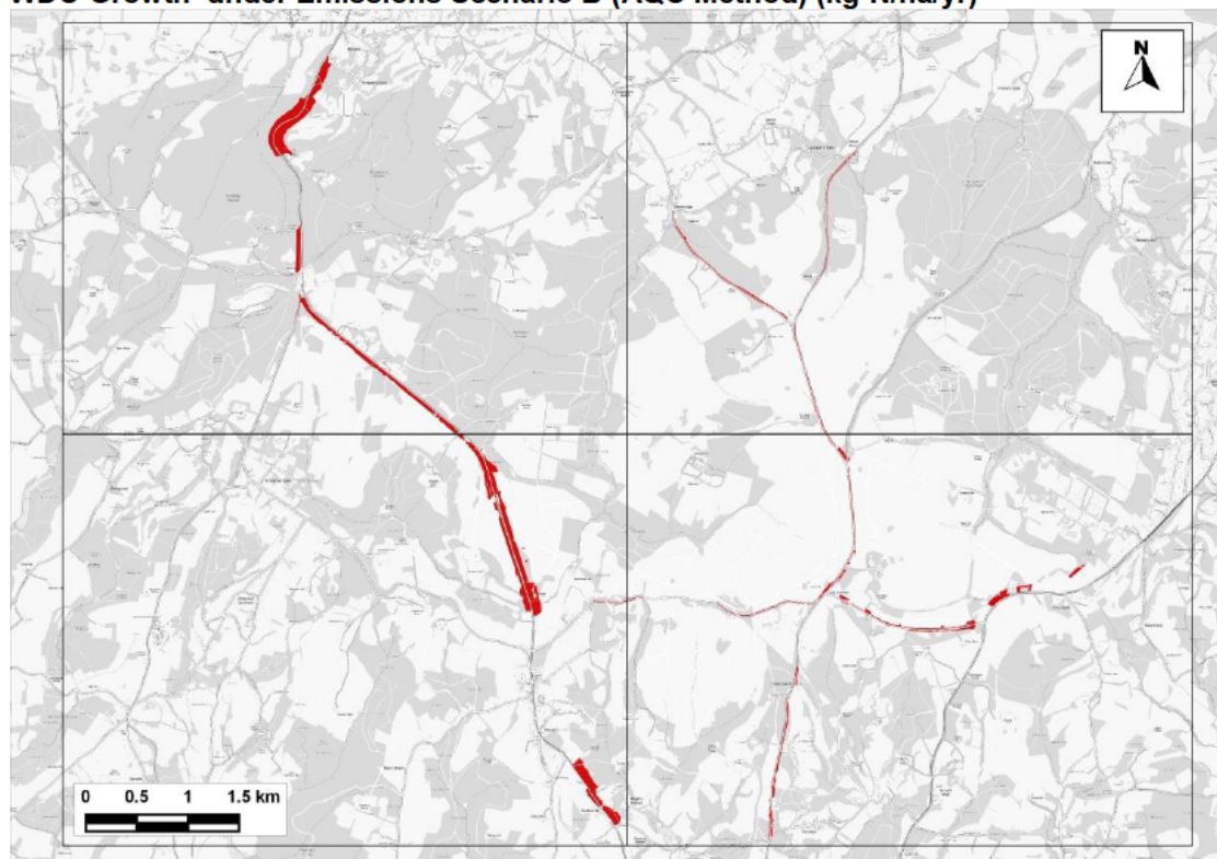
Figure 13.18: Areas in SAC Predicted to Experience an Increase in Nitrogen Deposition Greater than 1% of the 10 kg-N/ha/yr Critical Load where this Critical Load would also be Exceeded - Comparing 'With Plan' to 'No WDC-Growth' Scenarios under Emissions Scenario B (AQC Method)
