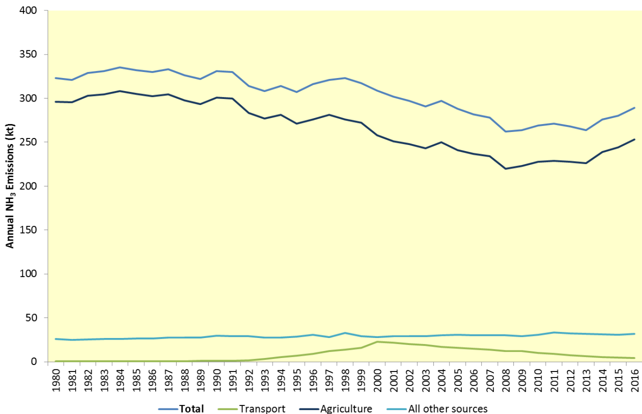
Figure 3.6: UK Total \text{NH}_3 Emissions: 1980 – 2016 (Defra, 2018b)
