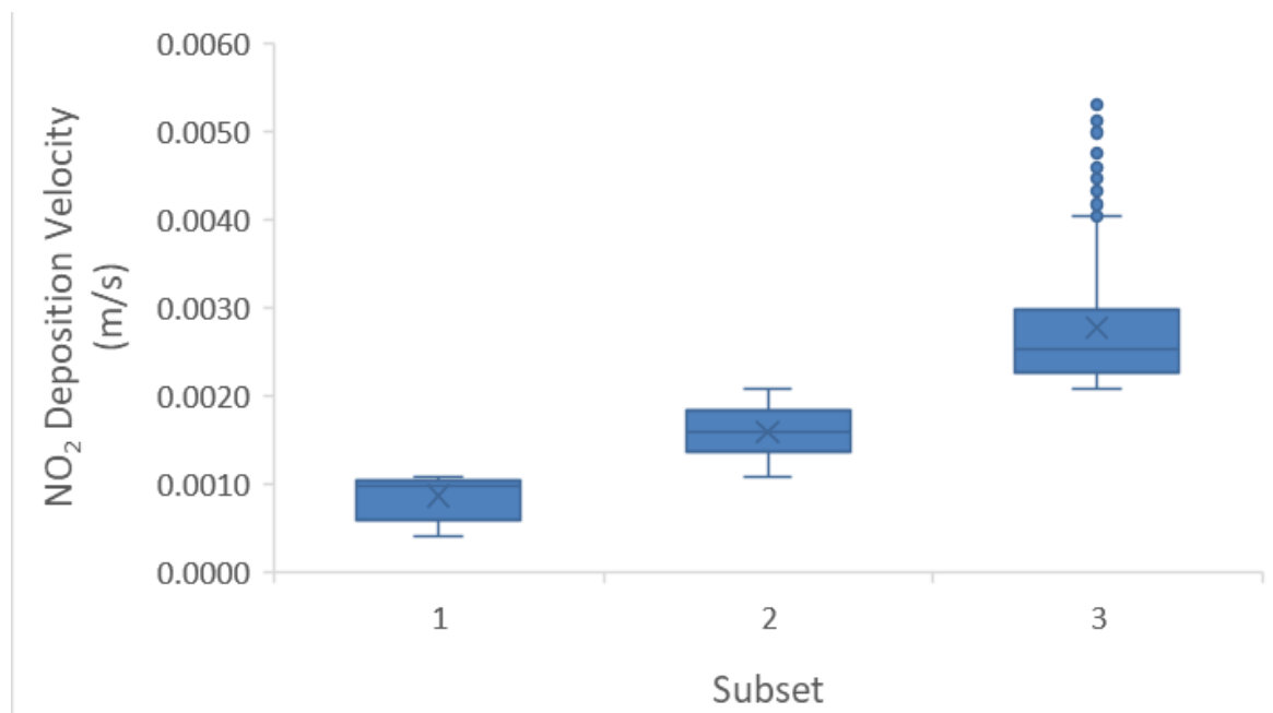
Figure 5.43: Hourly Values of V_d ( \text{NO}_2 ) to Heath During Winter Daytime, separated into Three Subsets
