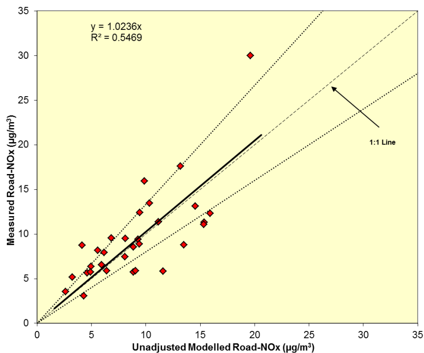
Figure 5.12: Modelled vs Measured Annual Mean Road-NOx, Link Set 2, Iteration 3
