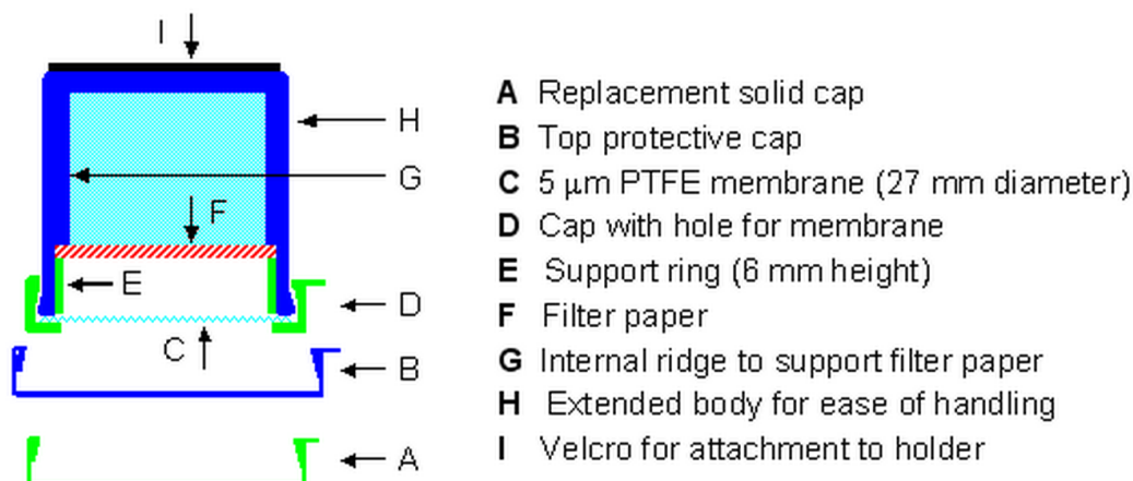
Figure 4.4: Diagram of an ALPHA sampler 14
