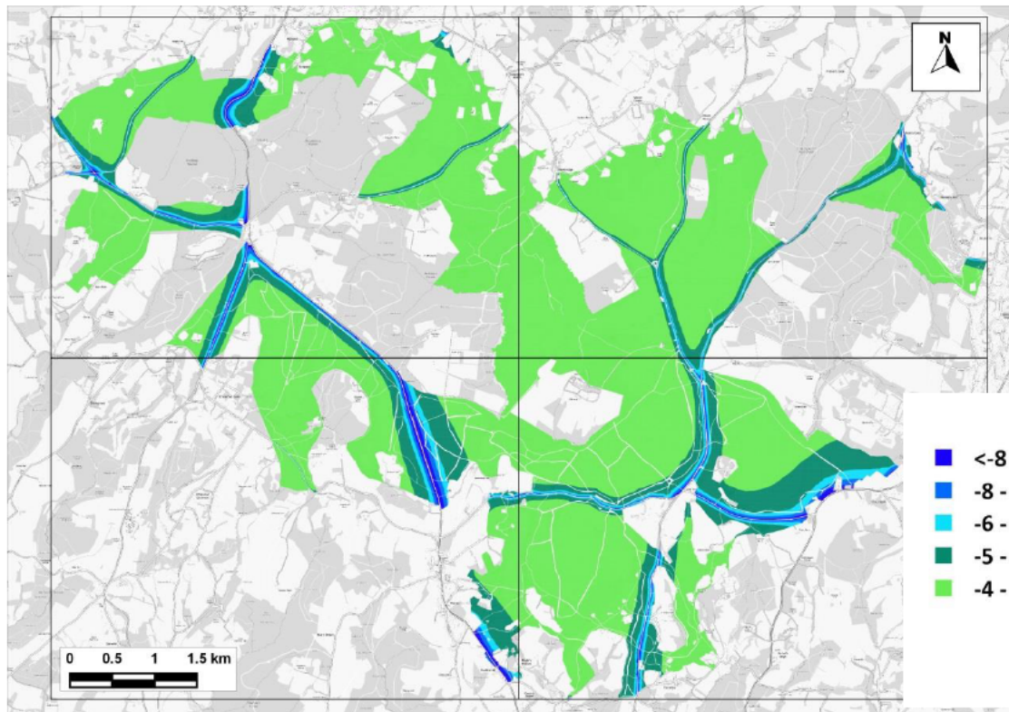
Figure 15.5: Change in Predicted Annual Mean NO x Comparing 'With Plan' Emissions Scenario C to 'No Growth' Emissions Scenario A ( \mu\text{g}/\text{m}^3 )
