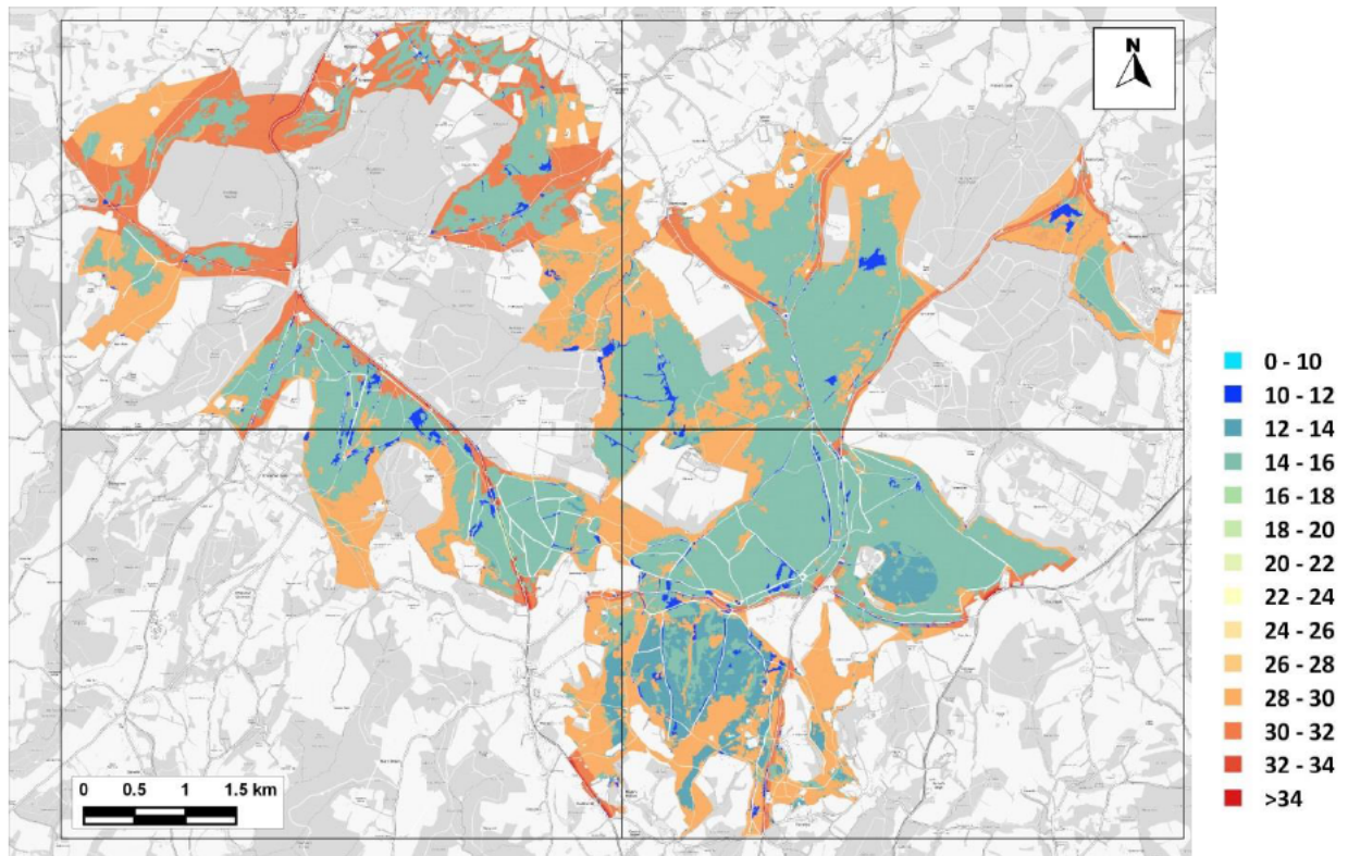
Figure 9.53: Nitrogen Deposition to SAC – Existing Baseline (AQC Method) (kg-N/ha/yr)
