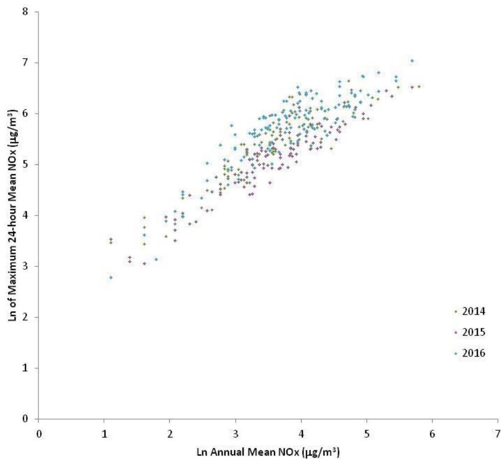
Figure 5.36: Natural Logarithm of Annual Mean NOx vs Maximum 24-hour Mean NOx at all Suitable AURN Sites over 3 Years
