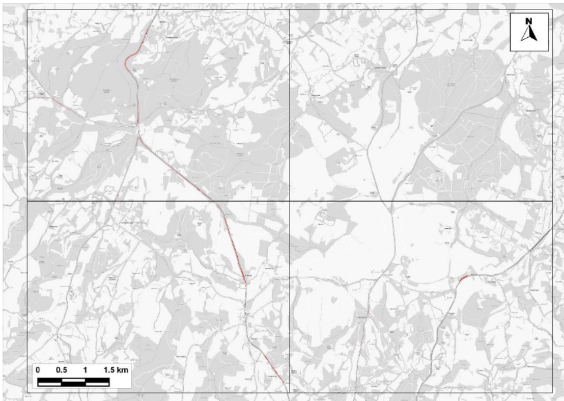
Figure 14.6: Areas in SAC Predicted to Experience an Increase in Annual Mean NH 3 Concentrations Greater than 1% of the 1 µg/m 3 Critical Level where the Critical Level would also be Exceeded (Comparing 'With Plan' to 'No Growth Scenarios')
