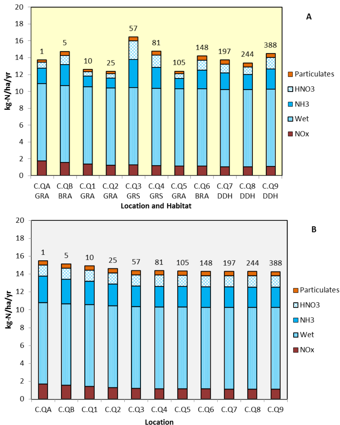
Figure 9.33: Deposition to Ecological Transect C – AQC Method – (A) Using Current Habitat Types and (B) If all Habitat were Heath (approximate distance from the nearest main road to each quadrant to shown numerically above each column) 36
