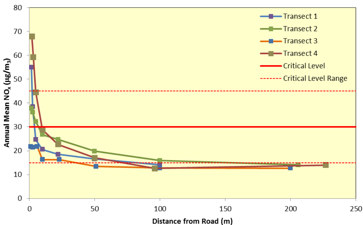
Figure 8.9: Two-year Mean NO x Concentration vs Distance from Roads along the Four Transects
