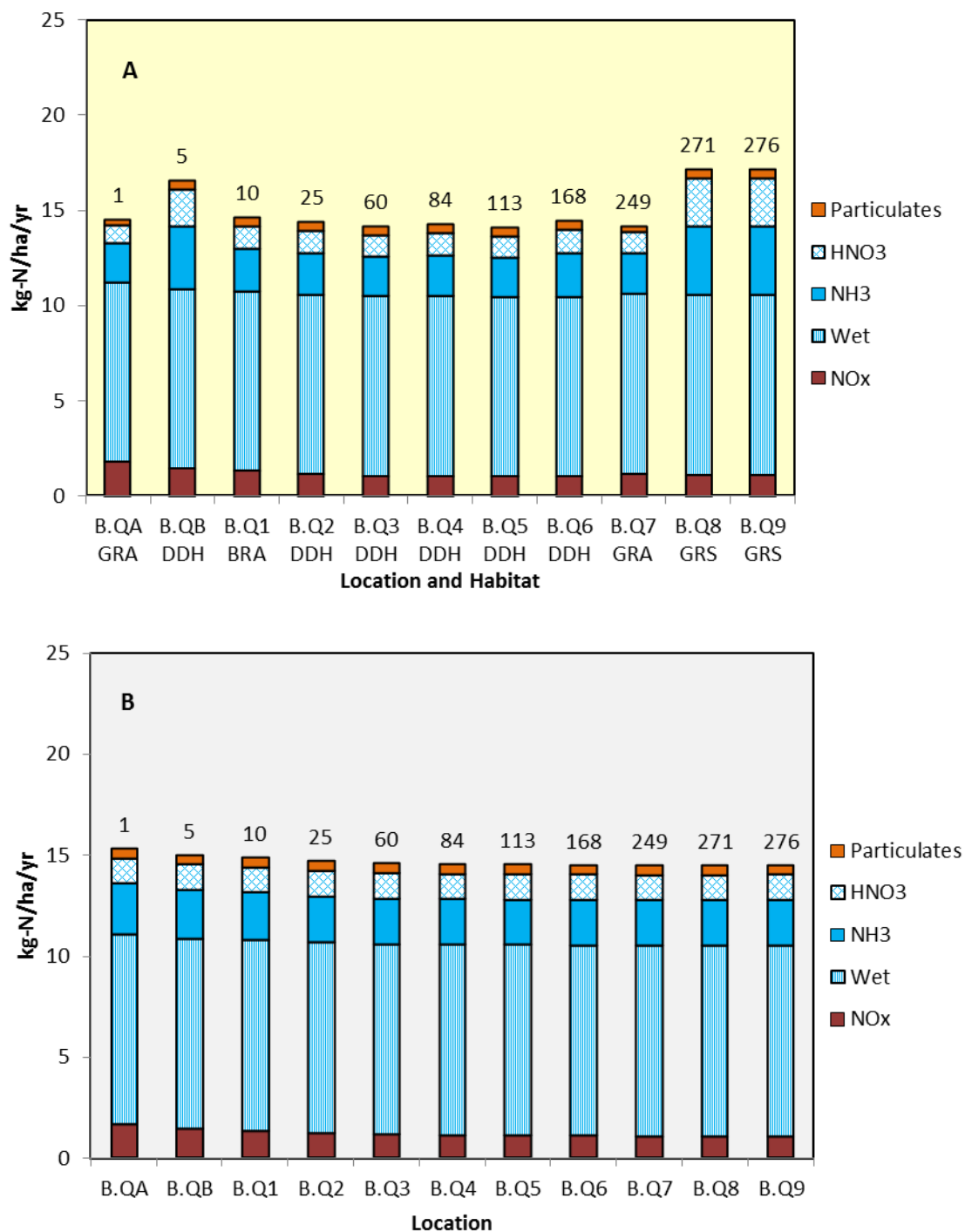
Figure 9.32: Deposition to Ecological Transect B – AQC Method – (A) Using Current Habitat Types and (B) If all Habitat were Heath (approximate distance from the nearest main road to each quadrant to shown numerically above each column) 36
