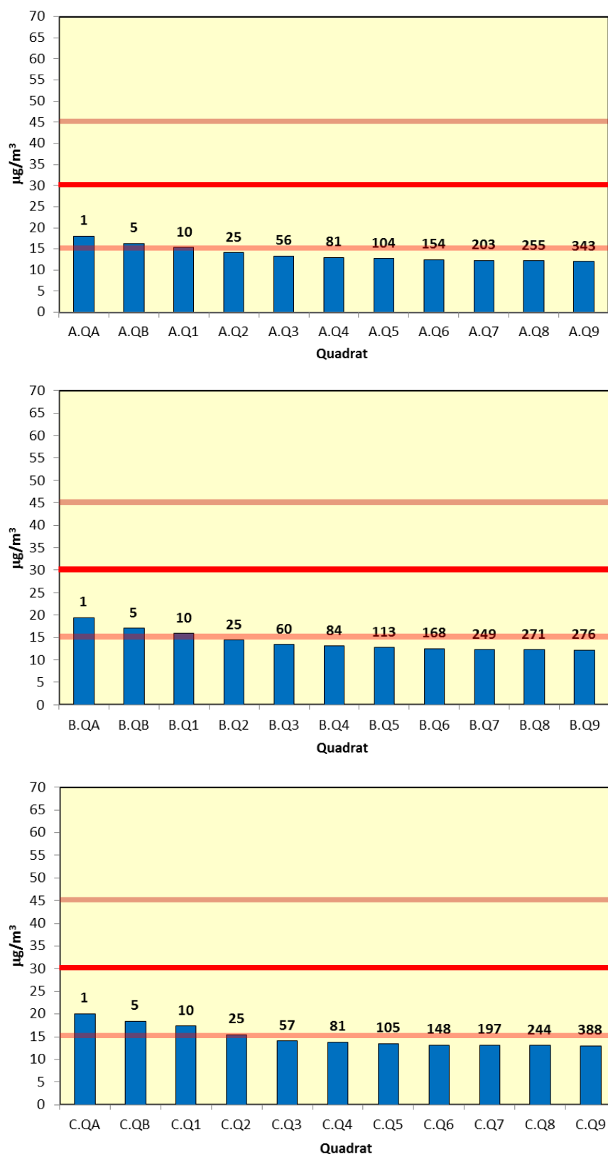
Figure 9.1: Annual Mean NOx Concentrations Along Transects A, B, and C. Approximate distance from the nearest main road to each quadrant to shown numerically above each column. Lines show the 30 \mu\text{g}/\text{m}^3 critical level and the 15 \mu\text{g}/\text{m}^3 and 45 \mu\text{g}/\text{m}^3 critical level range suggested by CEH.
