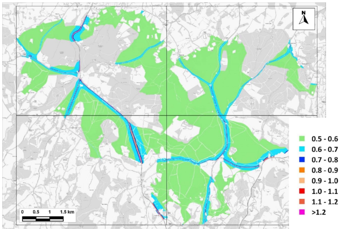
Figure 12.3: Predicted Annual Mean \text{NH}_3 Concentrations across the SAC– 2028 With Plan ( \mu\text{g}/\text{m}^3 )
