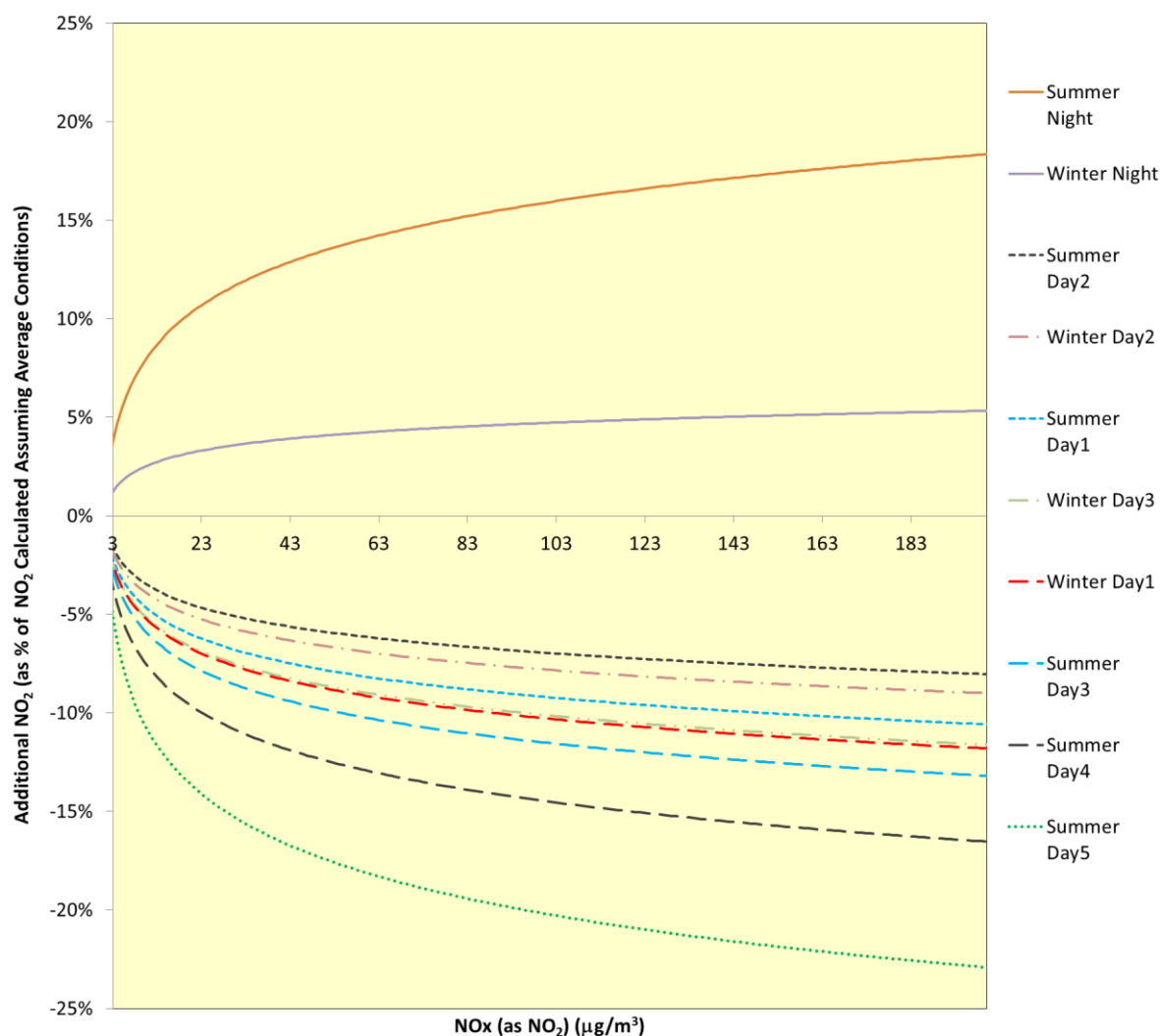
Figure 5.29: Period-specific Uplifts Applied to NO 2 Concentrations Calculated using Defra's NO x to NO 2 Calculator (ten periods)
