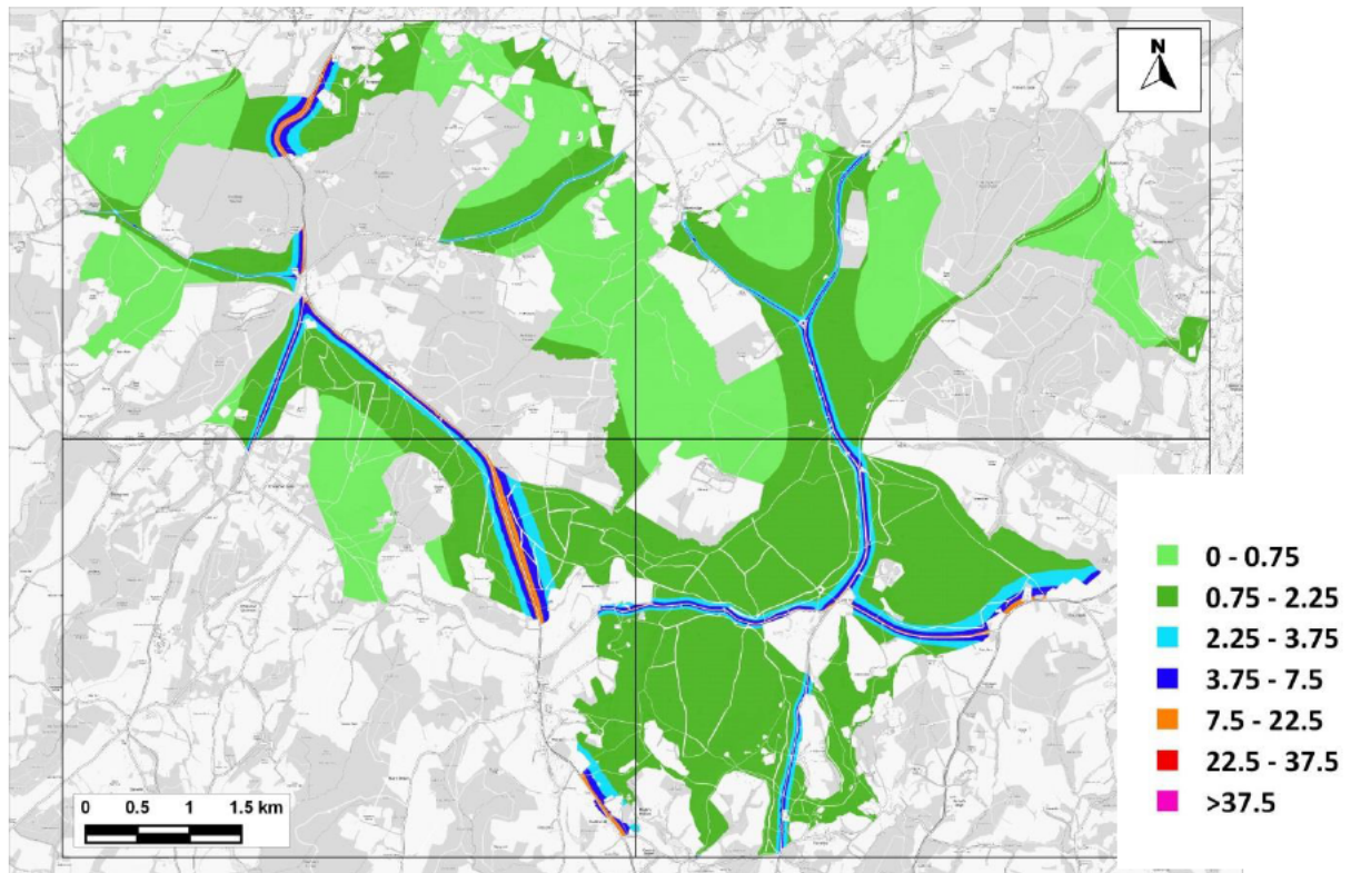
Figure 14.21: Change in Maximum Predicted 24-hour Mean NO x Comparing 'With Plan' to 'No Growth' under Emissions Scenario C ( \mu\text{g}/\text{m}^3 )
