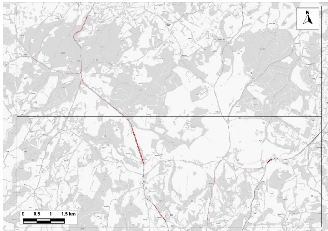
Figure 14.2: Areas in SAC Predicted to Experience an Increase in Annual Mean NO x Concentrations Greater than 1% of the 30 \mu\text{g}/\text{m}^3 Critical Level where the Critical Level would also be Exceeded - Comparing 'With Plan' to 'No Growth' Scenarios under Emissions Scenario A
