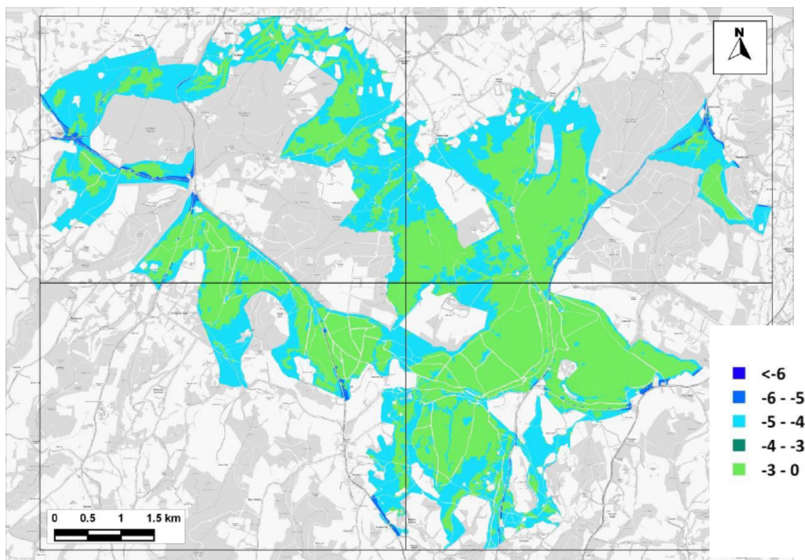
Figure 15.8: Change in Predicted Nitrogen Deposition to SAC Comparing 'With Plan' Emissions Scenario C to 'No Growth' Emissions Scenario A (AQC Method) (kg-N/ha/yr)
