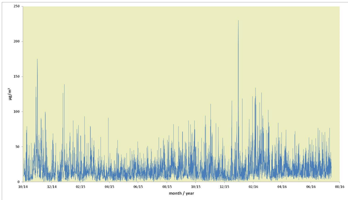
Figure 8.1: 1-hour Mean Nitrogen Oxides Concentrations at Kingstanding between October 2014 and August 2016
