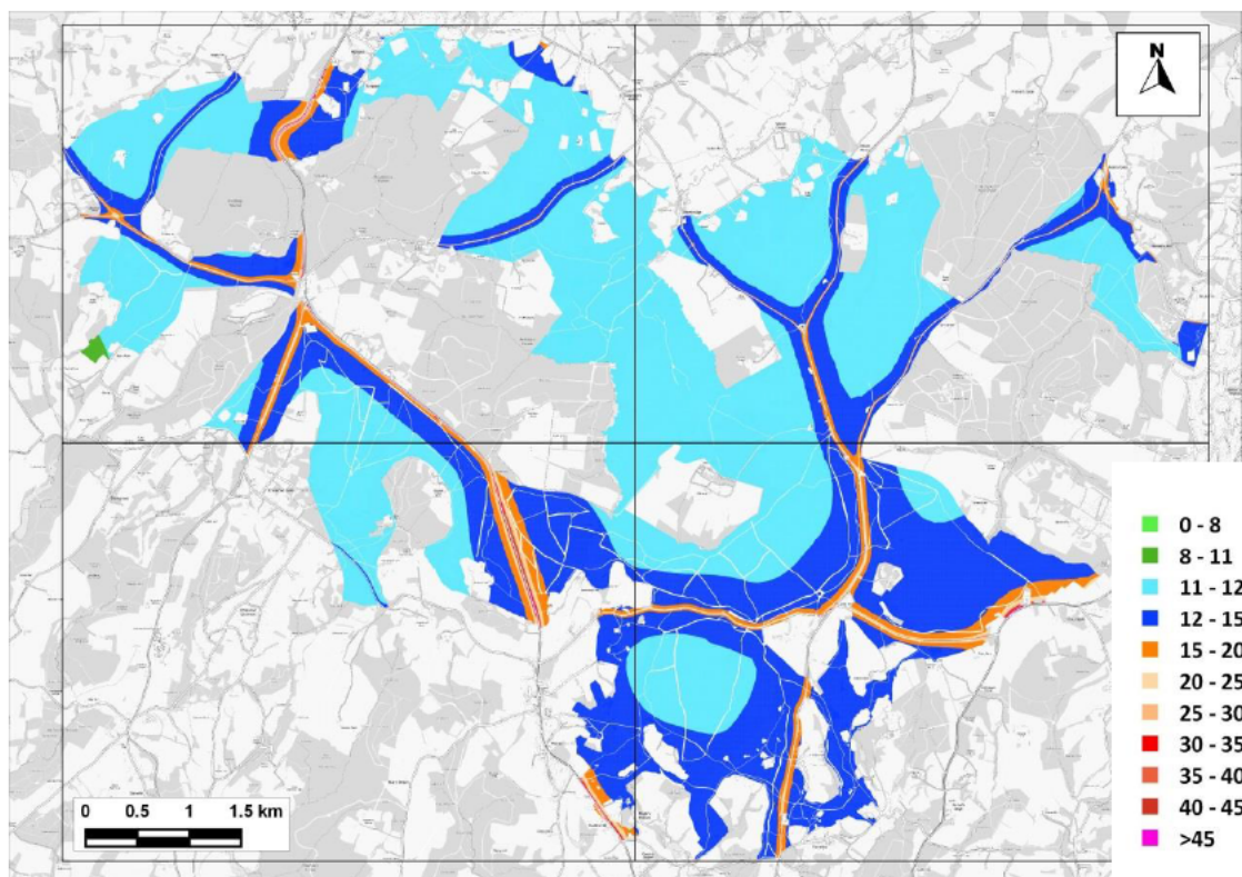
Figure 12.1: Predicted Annual Mean NO x Concentrations across the SAC– 2028 With Plan - A ( \mu\text{g}/\text{m}^3 )
