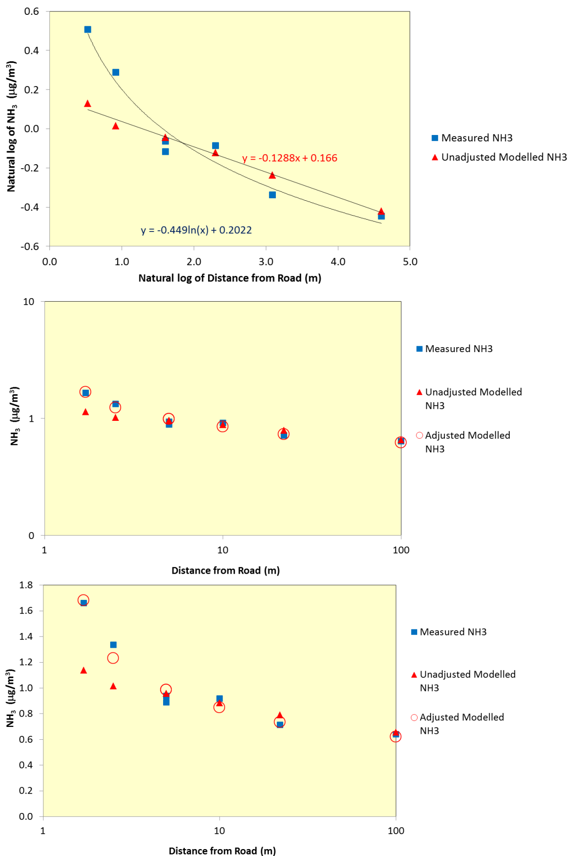
Figure 5.33: Measured vs Predicted 2-Year Average \text{NH}_3 Concentrations along Transect 1: top = unadjusted model on log scales, middle = unadjusted and adjusted models on log 'y' scale; bottom = unadjusted and adjusted models.
