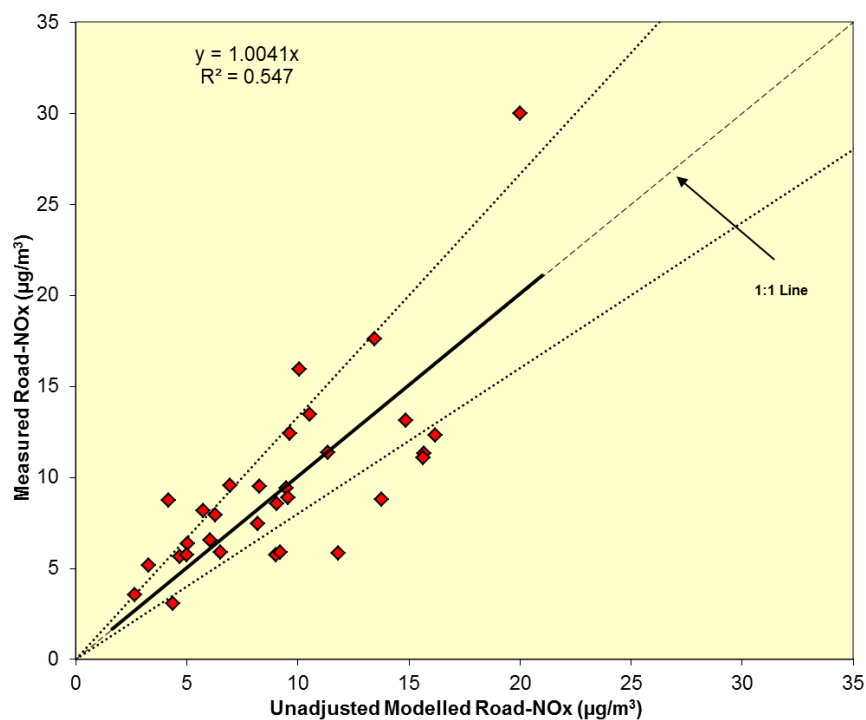
Figure 5.15: Modelled vs Measured Annual Mean Road-NOx, Link Set 2, Iteration 4
