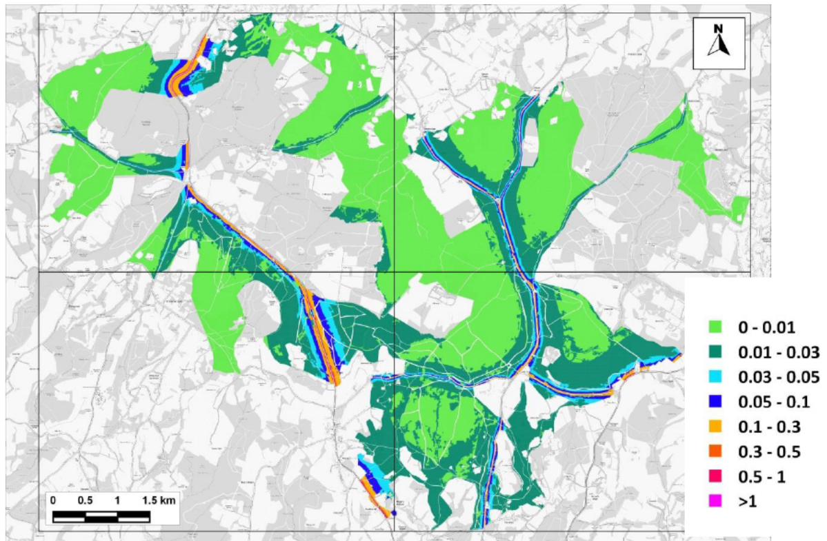
Figure 13.15: Change in Predicted Nitrogen Deposition to SAC Comparing 'With Plan' to 'No WDC-Growth' Under Emission Scenario B (EA Method) (kg-N/ha/yr)
