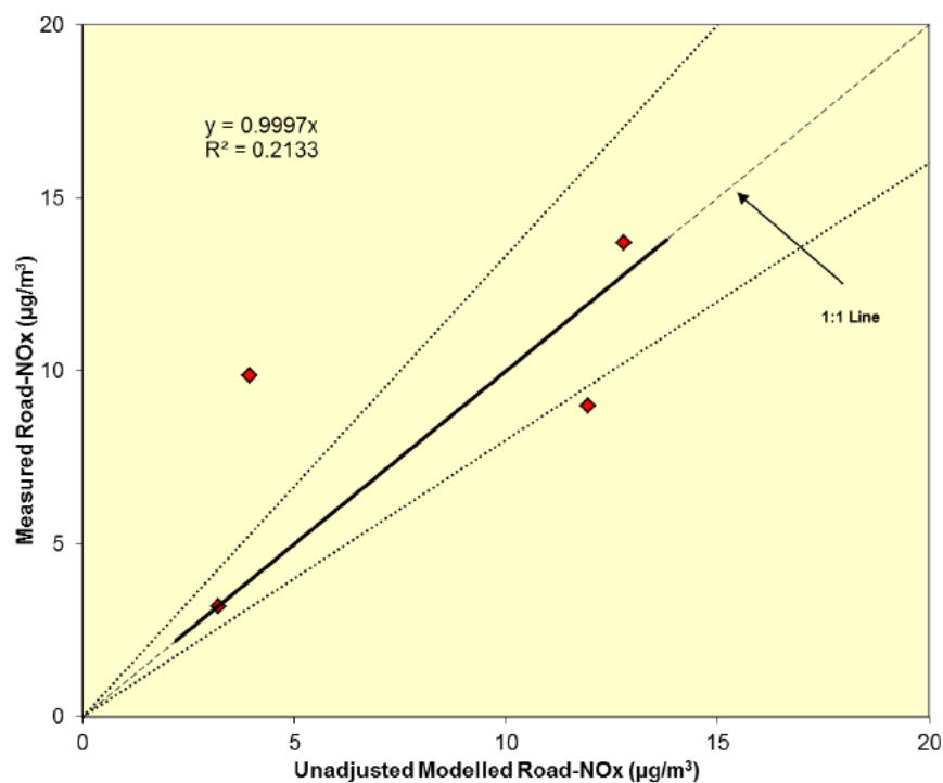
Figure 5.16: Modelled vs Measured Annual Mean Road-NOx, Link Set 3, Iteration 4
