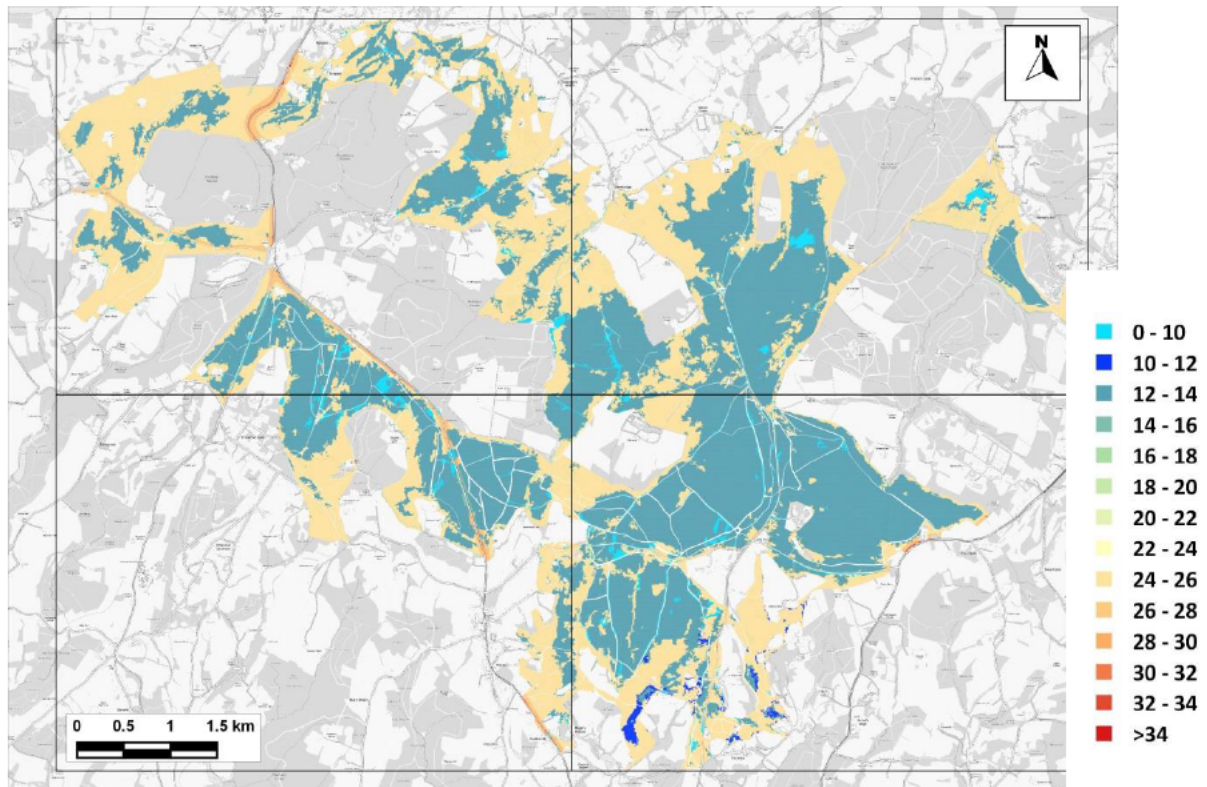
Figure 12.13: Nitrogen Deposition to SAC – 2028 With Plan - C (AQC Method) (kg-N/ha/yr)
