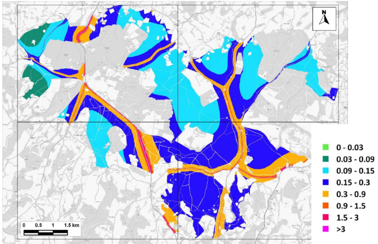
Figure 14.11: Change in Predicted Annual Mean NO x Comparing 'With Plan' to 'No Growth' Under Emissions Scenario B ( \mu\text{g}/\text{m}^3 )
