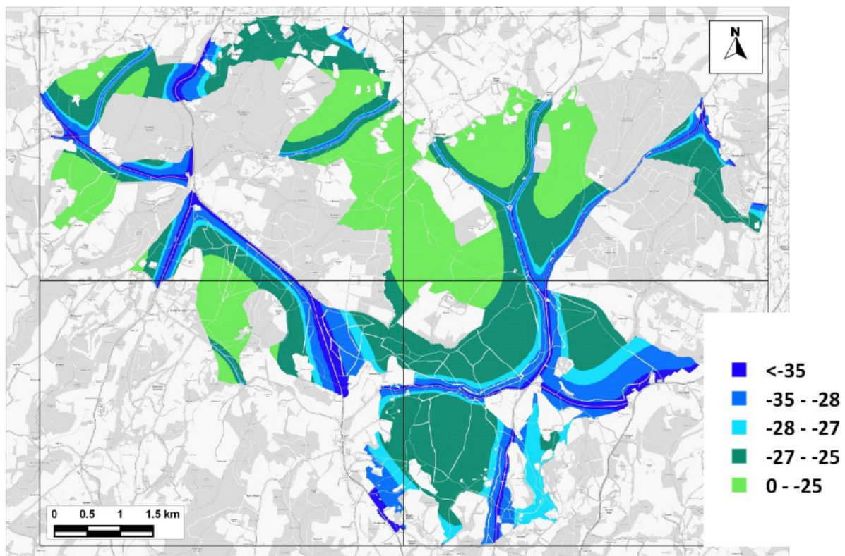
Figure 15.6: Change in Maximum Predicted 24-hour Mean NO x Comparing 'With Plan' Emissions Scenario C to 'No Growth' Emissions Scenario A ( \mu\text{g}/\text{m}^3 )
