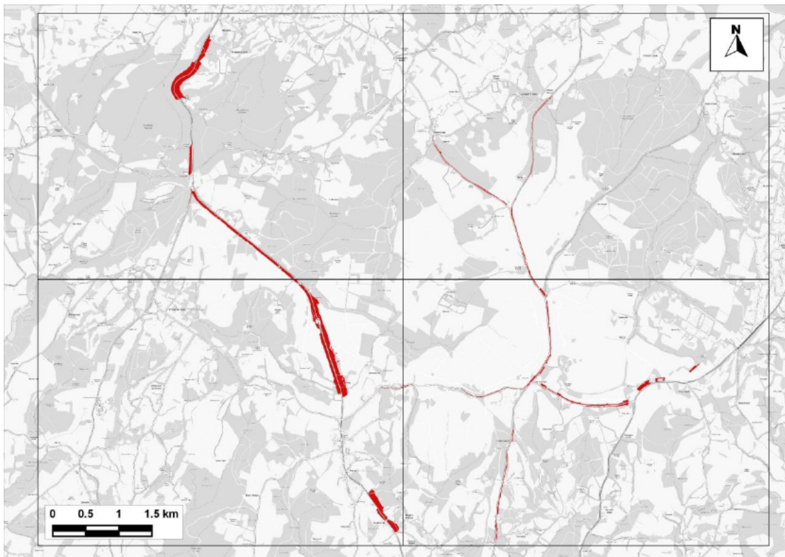
Figure 13.24: Areas in SAC Predicted to Experience an Increase in Nitrogen Deposition Greater than 1% of the 10 kg-N/ha/yr Critical Load where this Critical Load would also be Exceeded - Comparing 'With Plan' to 'No WDC-Growth' Scenarios under Emissions Scenario C (EA Method)
