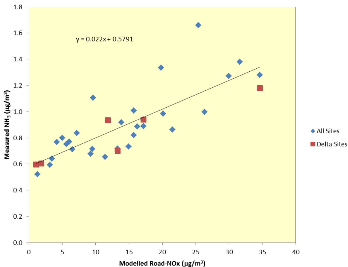
Figure 5.4: Measured \text{NH}_3 vs Predicted Road- \text{NO}_x
