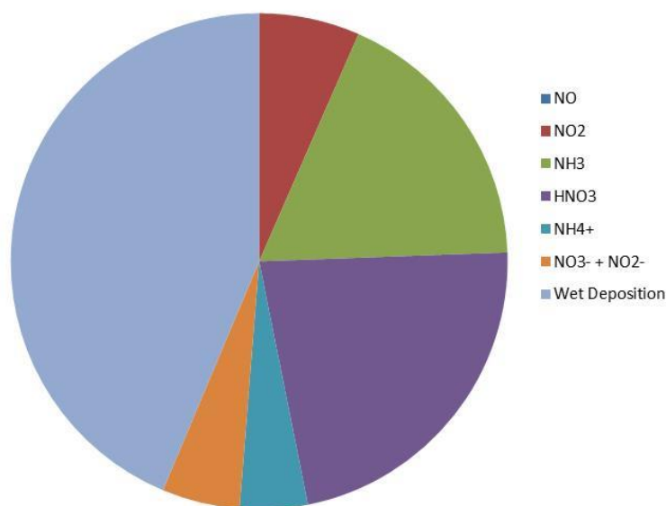
Figure 9.56: Total Nitrogen Deposition to the Ashdown Forest SAC by Pollutant (taking account of relative cover of each land use) (AQC Method)
