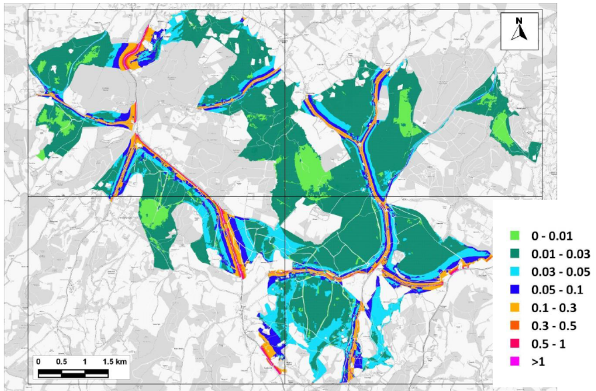
Figure 14.17: Change in Predicted Nitrogen Deposition to SAC Comparing 'With Plan' to 'No Growth' Scenarios under Emissions Scenario B (AQC Method) (kg-N/ha/yr)
