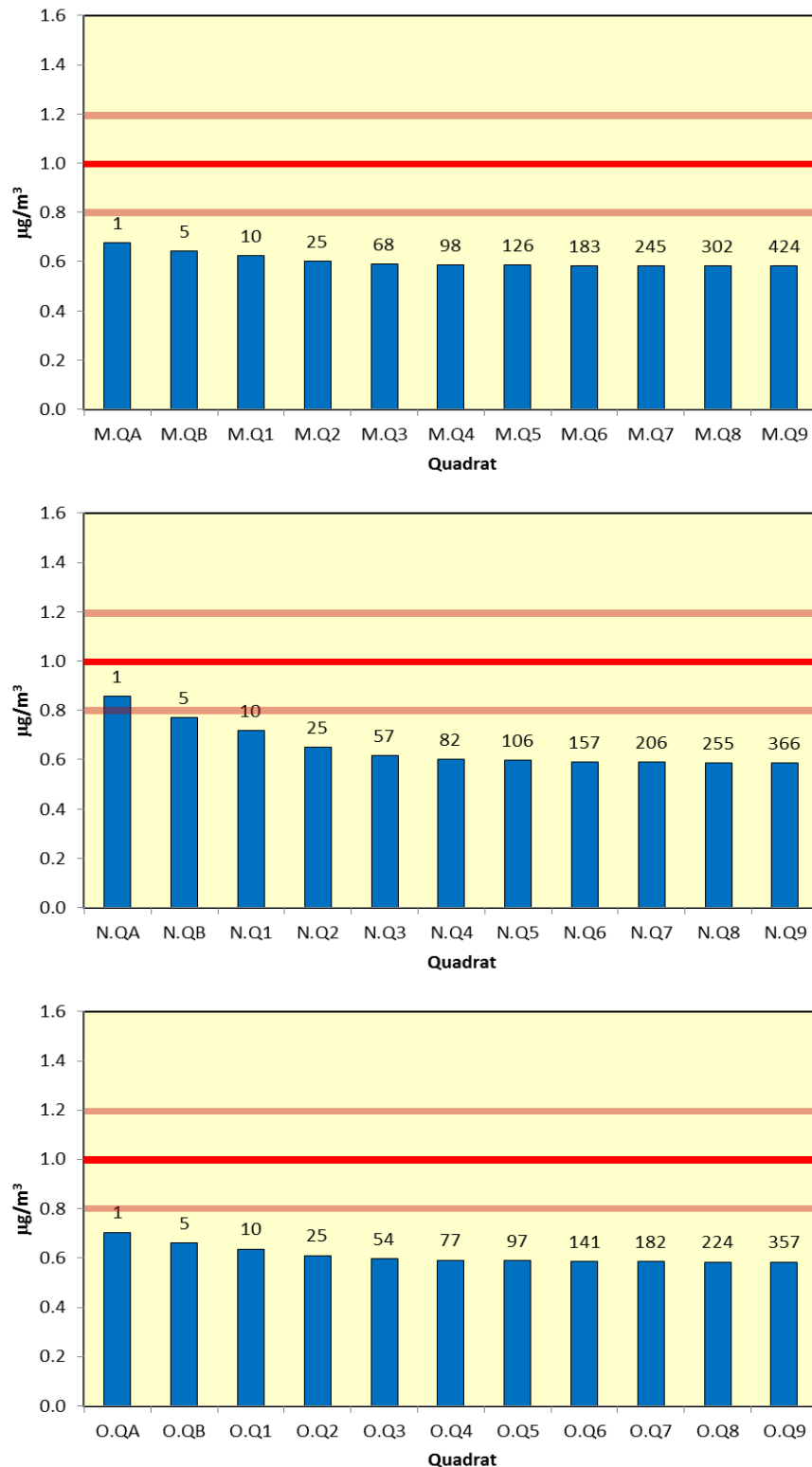
Figure 9.15: Annual Mean \text{NH}_3 Concentrations Along Transects M, N, and O. Approximate distance from the nearest main road to each quadrat to shown numerically above each column. Lines show the 1 \mu\text{g}/\text{m}^3 critical level and the \pm 20\% critical level range suggested by CEH.
