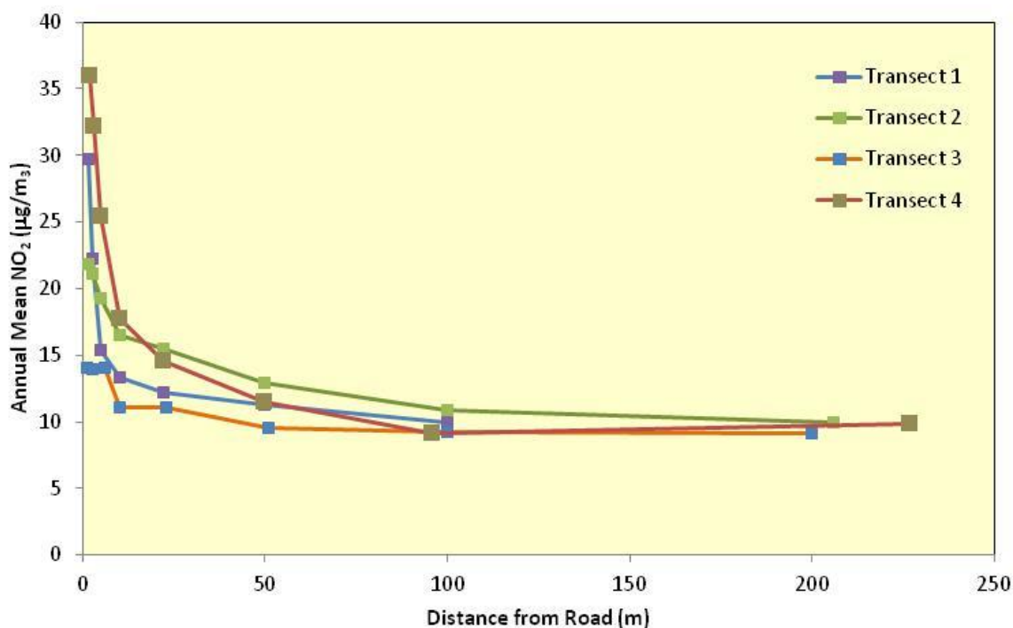
Figure 8.7: Two-year Mean Measured NO 2 Concentration vs Distance from Roads along the Four Transects 32
