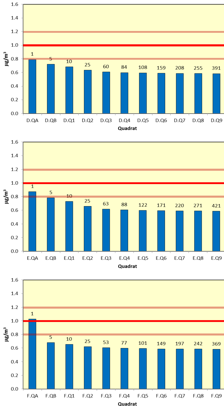
Figure 9.12: Annual Mean \text{NH}_3 Concentrations Along Transects D, E, and F. Approximate distance from the nearest main road to each quadrat to shown numerically above each column. Lines show the 1 \mu\text{g}/\text{m}^3 critical level and the \pm 20\% critical level range suggested by CEH.
