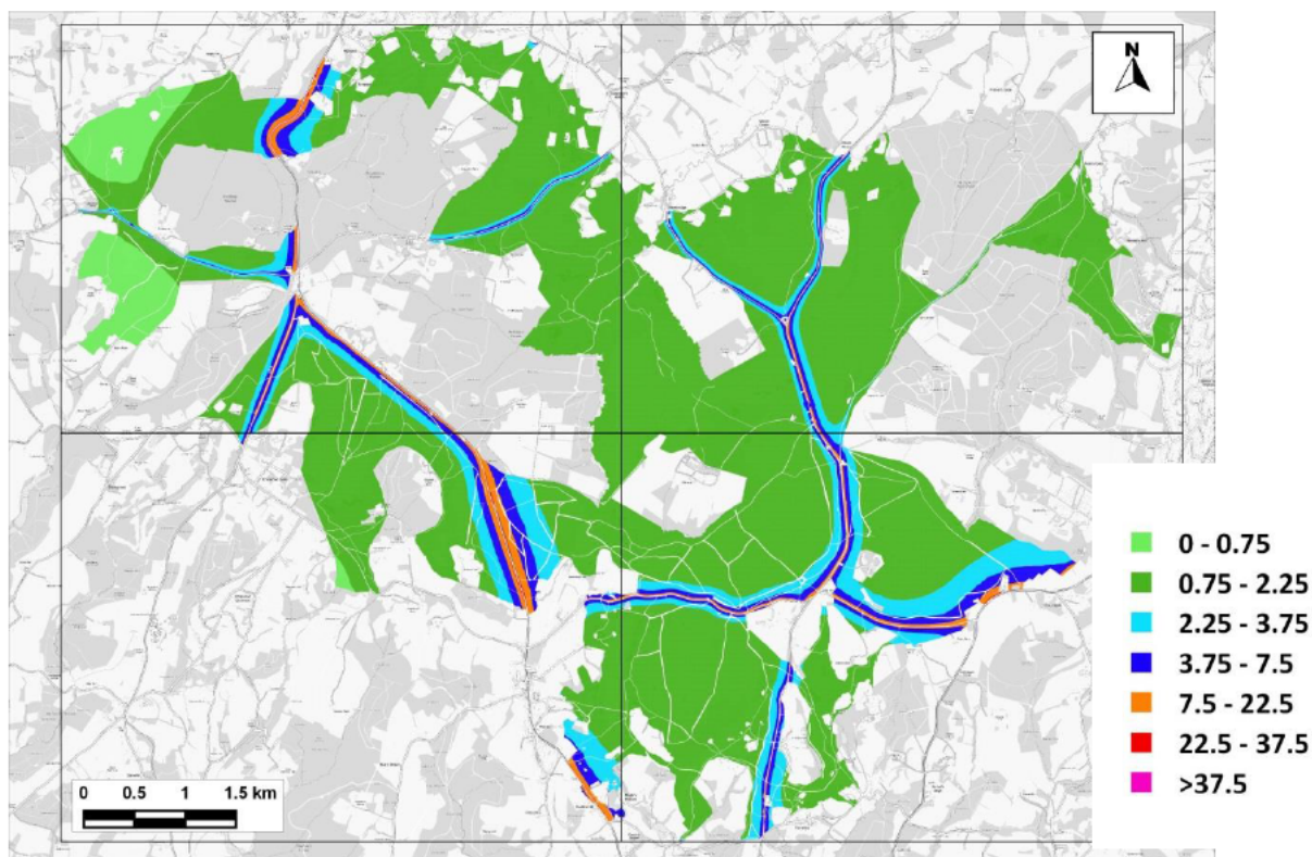
Figure 14.13: Change in Maximum Predicted 24-hour Mean NO x Comparing 'With Plan' to 'No Growth' under Emissions Scenario B ( \mu\text{g}/\text{m}^3 )
