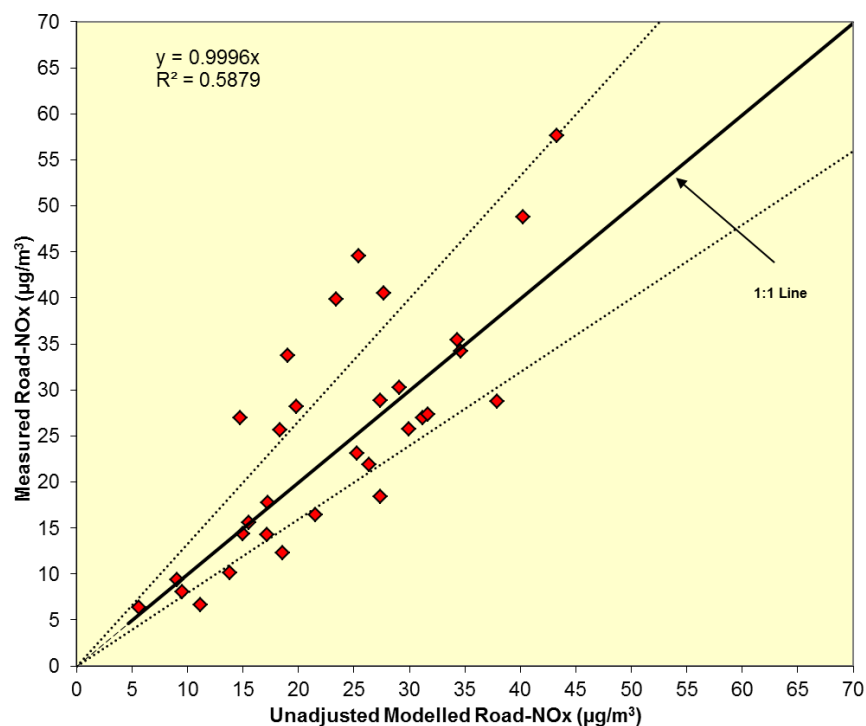
Figure 5.11: Modelled vs Measured Annual Mean Road-NOx, Link Set 1, Iteration 3
