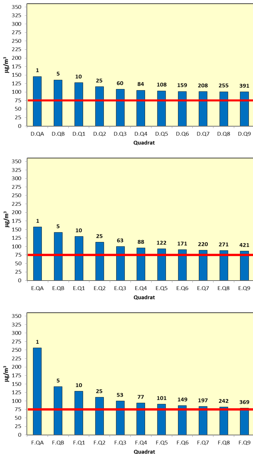
Figure 9.7: Maximum 24-hour Mean NOx Concentrations Along Transects D, E, and F. Approximate distance from the nearest main road to each quadrat to shown numerically above each column. Horizontal line shows the 75 \mu\text{g}/\text{m}^3 critical level.
