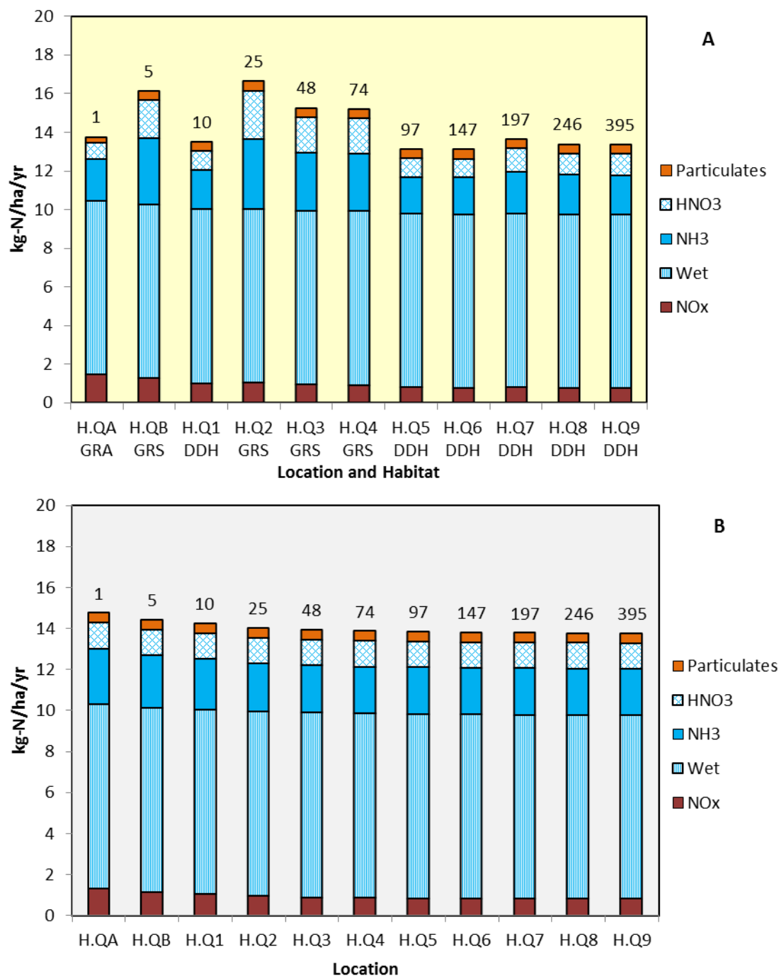
Figure 9.38: Deposition to Ecological Transect H – AQC Method – (A) Using Current Habitat Types and (B) If all Habitat were Heath (approximate distance from the nearest main road to each quadrant to shown numerically above each column) 36
