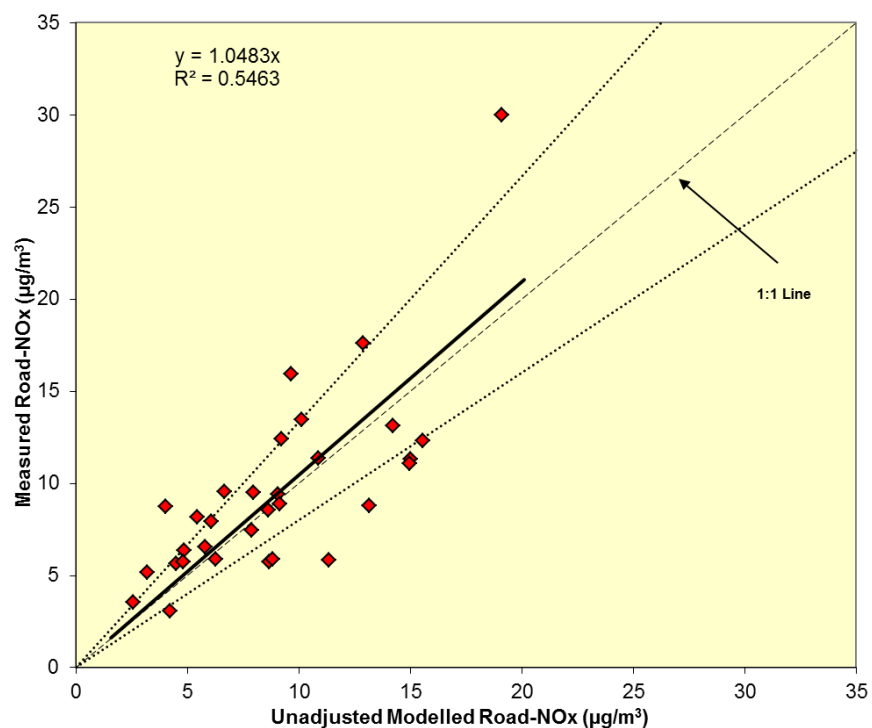
Figure 5.9: Modelled vs Measured Annual Mean Road-NOx, Link Set 2, Iteration 2
