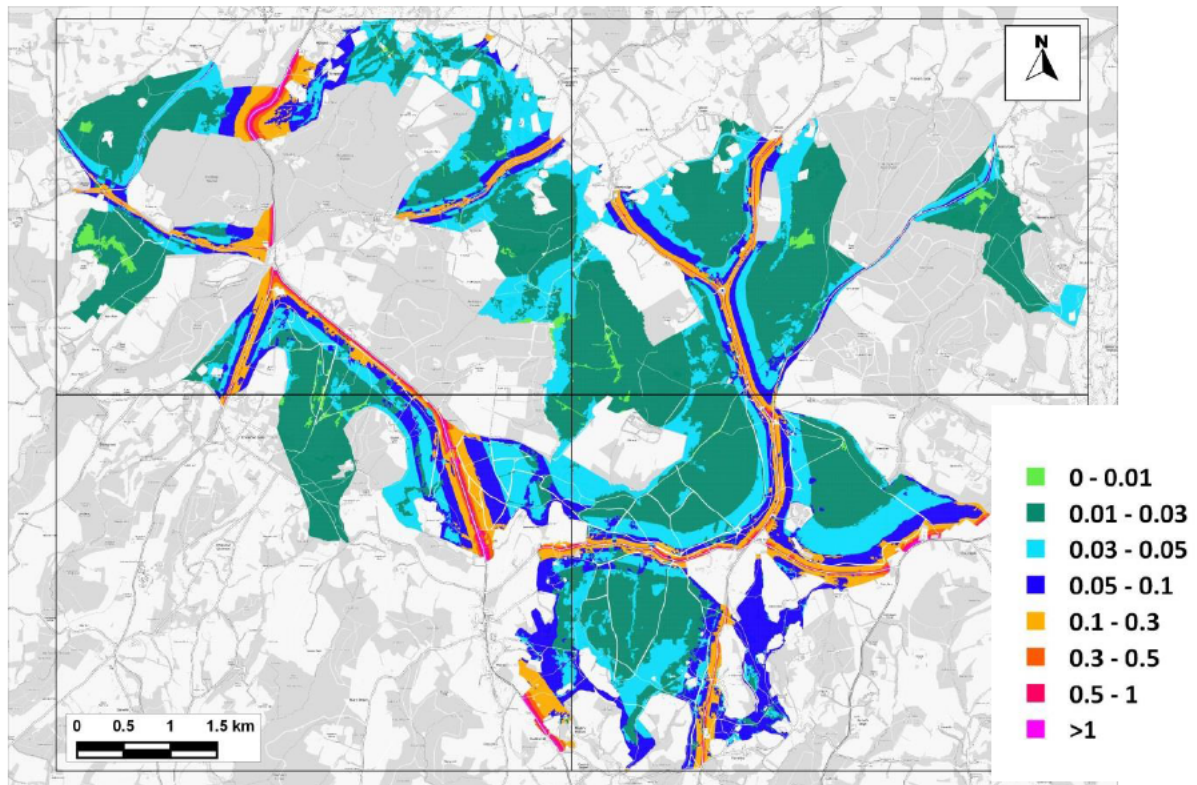
Figure 14.9: Change in Predicted Nitrogen Deposition to SAC Comparing 'With Plan' to 'No Growth' Scenarios under Emissions Scenario A (AQC Method) (kg-N/ha/yr)
