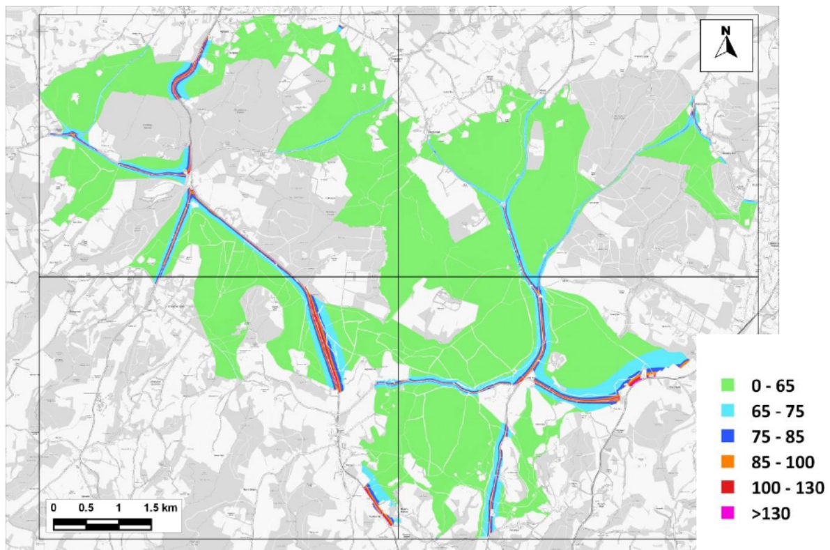
Figure 11.7: Predicted Maximum 24-hour Mean NO x Concentrations across the SAC – 2028 No WDC-Growth - B ( \mu\text{g}/\text{m}^3 )
