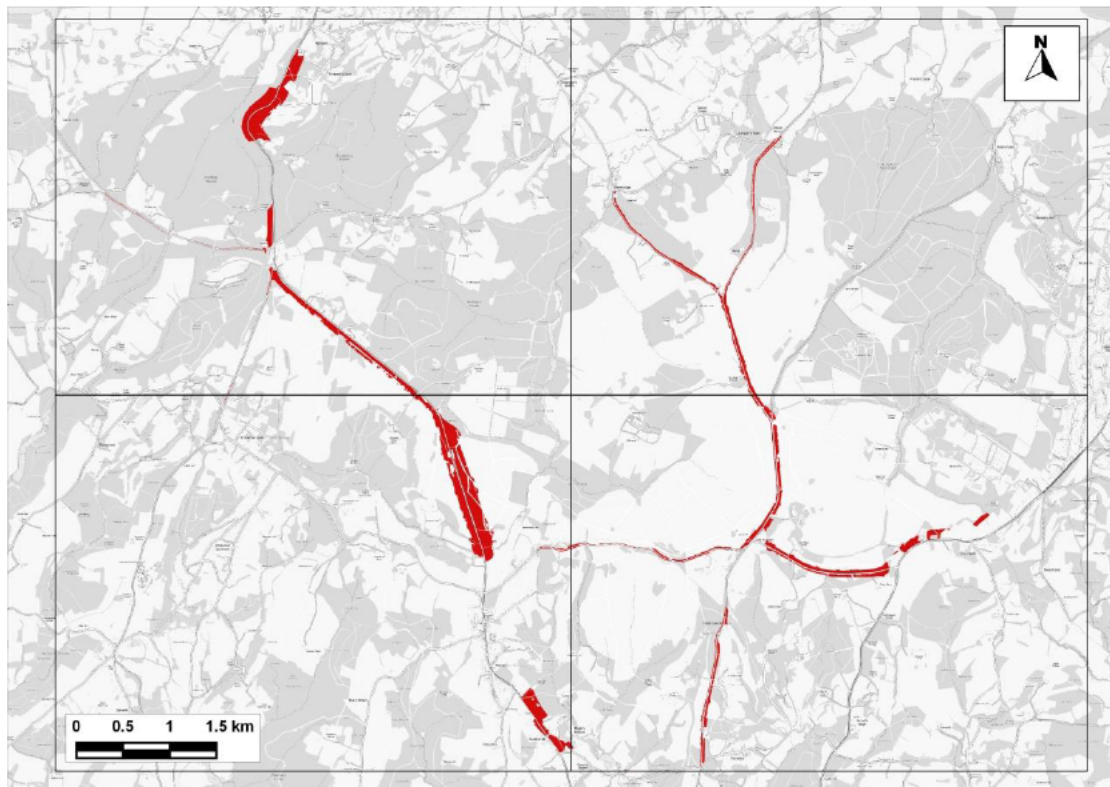
Figure 13.8: Areas in SAC Predicted to Experience an Increase in Nitrogen Deposition Greater than 1% of the 10 kg-N/ha/yr Critical Load where this Critical Load would also be Exceeded - Comparing 'With Plan' to 'No WDC-Growth' Scenarios under Emissions Scenario A (EA Method)
