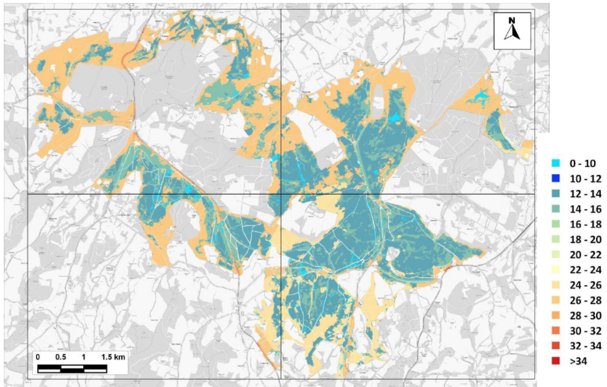
Figure 11.8: Nitrogen Deposition to SAC – 2028 No WDC-Growth - B (EA Method) (kg-N/ha/yr)
