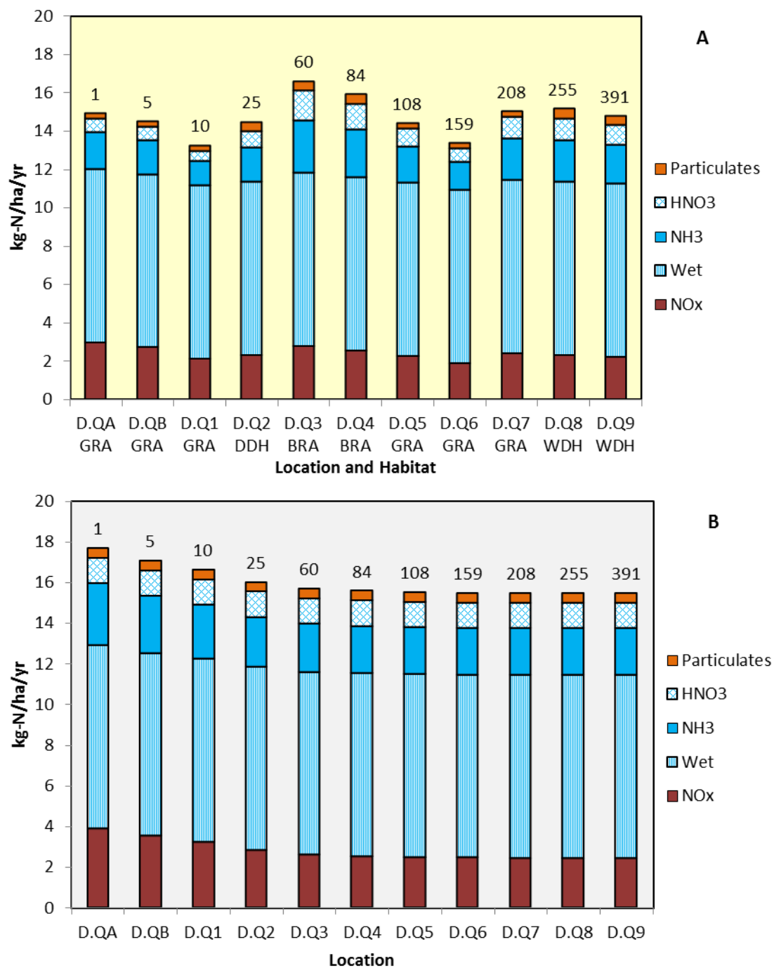
Figure 9.19: Deposition to Ecological Transect D – EA Method – A Using Current Habitat Types and B If all Habitat were Heath (approximate distance from the nearest main road to each quadrant to shown numerically above each column) 36
