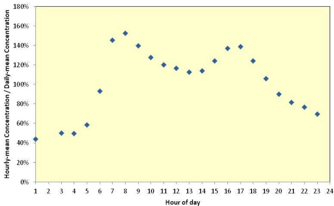
Figure 8.3: 1-hour Mean NHx Concentrations at Kingstanding between October 2014 and August 2016
