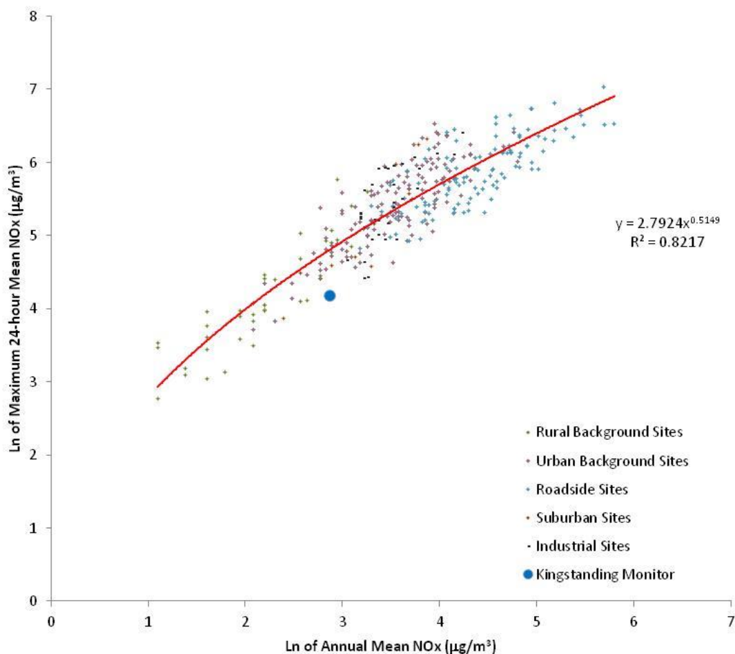
Figure 5.37: Natural Logarithm of Annual Mean NO x vs Maximum 24-hour Mean NO x at all Suitable AURN Sites over 3 Years, by Site Type – Also Showing the Period Mean at the Kingstanding Site
