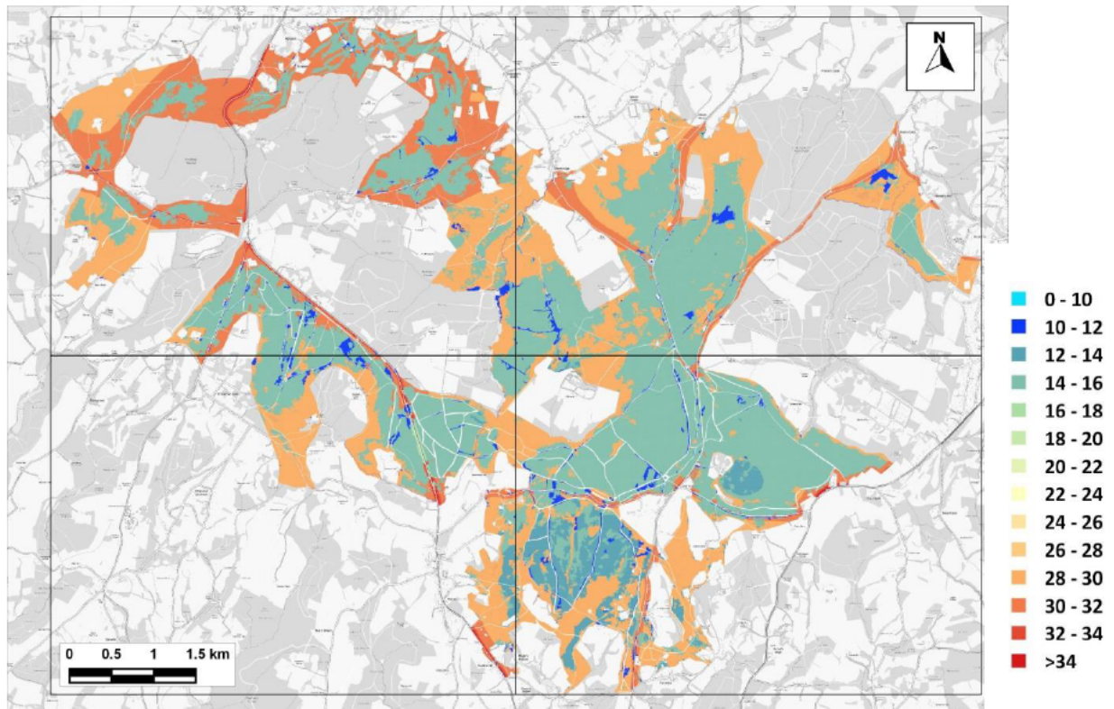
Figure 11.5: Nitrogen Deposition to SAC – 2028 No WDC-Growth - A (AQC Method) (kg-N/ha/yr)
