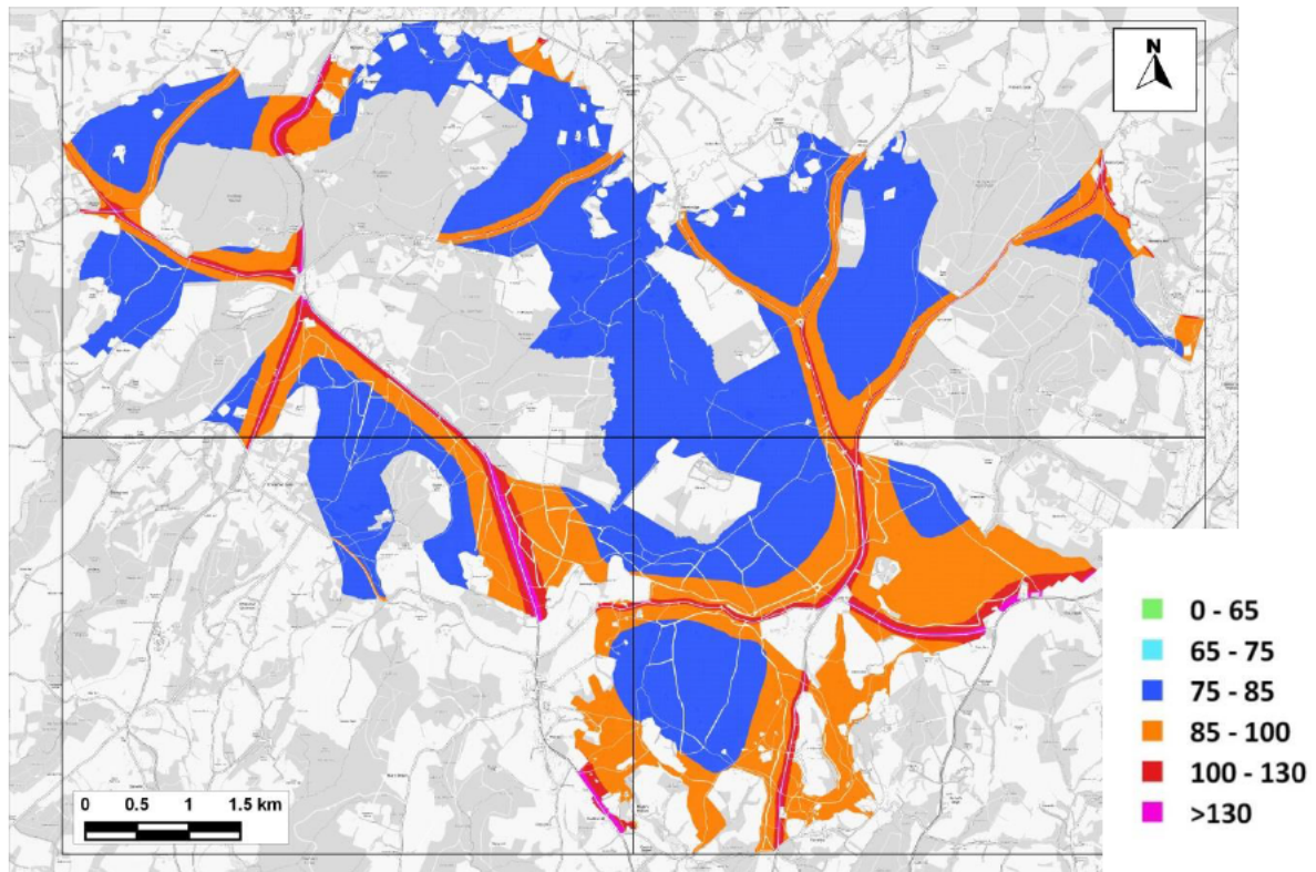
Figure 9.47: Predicted Maximum 24-hour Mean NO x Concentrations across the SAC - Existing Baseline ( \mu\text{g}/\text{m}^3 )
