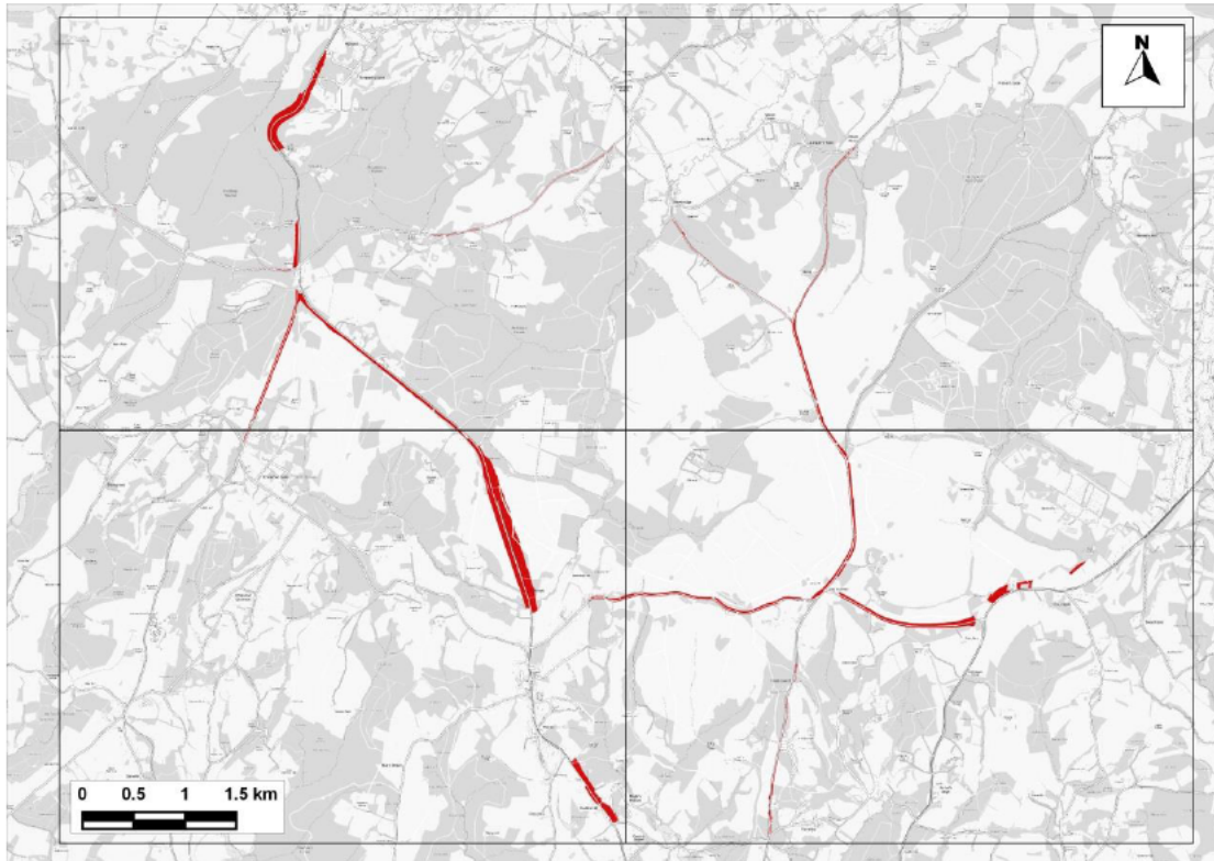
Figure 14.14: Areas in SAC Predicted to Experience an Increase in 24-hour Mean NO x Concentrations Greater than 10% of the 75 µg/m 3 Critical Level where the Critical Level would also be Exceeded - Comparing 'With Plan' to 'No Growth' Scenarios under Emissions Scenario B
