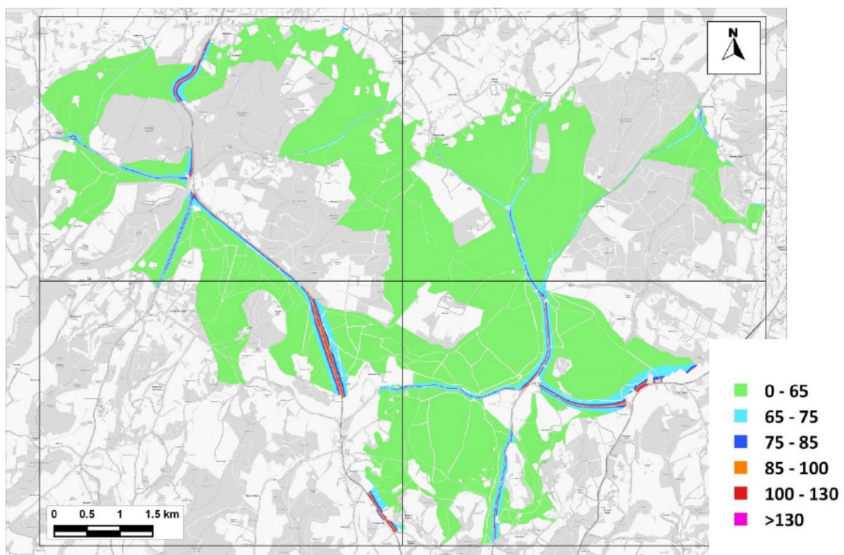
Figure 12.11: Predicted Maximum 24-hour Mean NO x Concentrations across the SAC– 2028 With Plan - C ( \mu\text{g}/\text{m}^3 )
