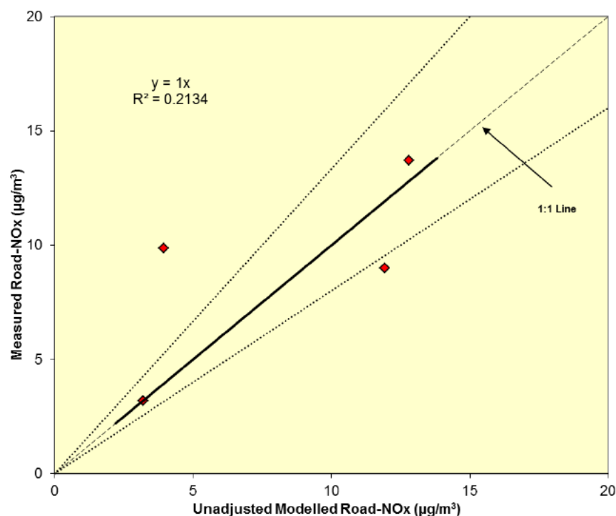
Figure 5.22: Modelled vs Measured Annual Mean Road-NOx, Link Set 3, Iteration 6
