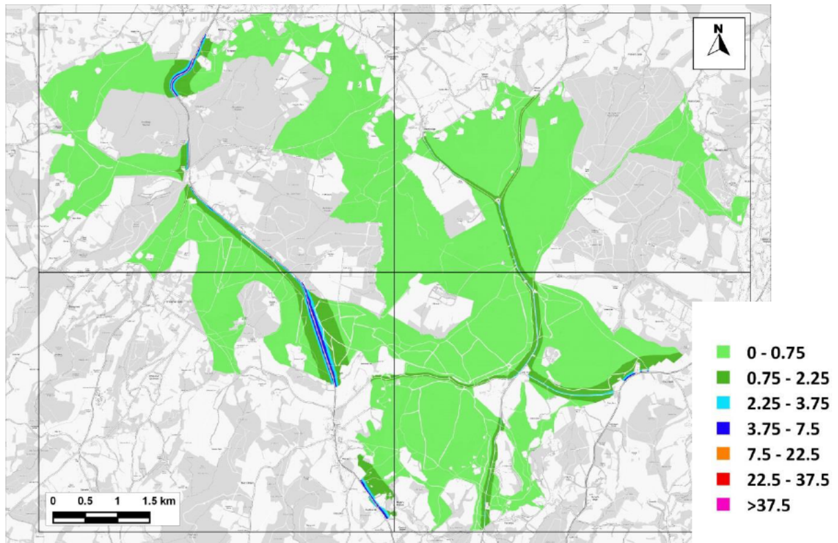
Figure 13.21: Change in Maximum Predicted 24-hour Mean NO x Comparing 'With Plan' to 'No WDC-Growth' under Emissions Scenario C ( \mu\text{g}/\text{m}^3 )
