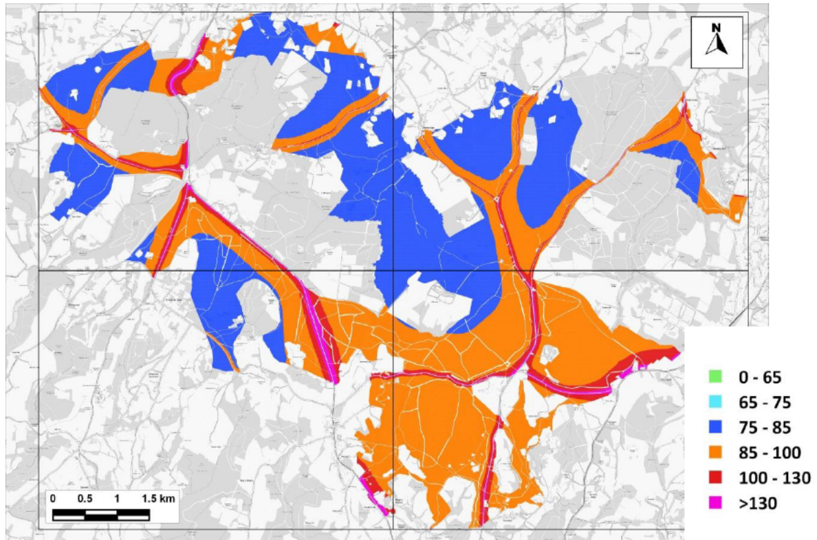
Figure 12.2: Predicted Maximum 24-hour Mean NO x Concentrations across the SAC– 2028 With Plan - A (µg/m 3 )
