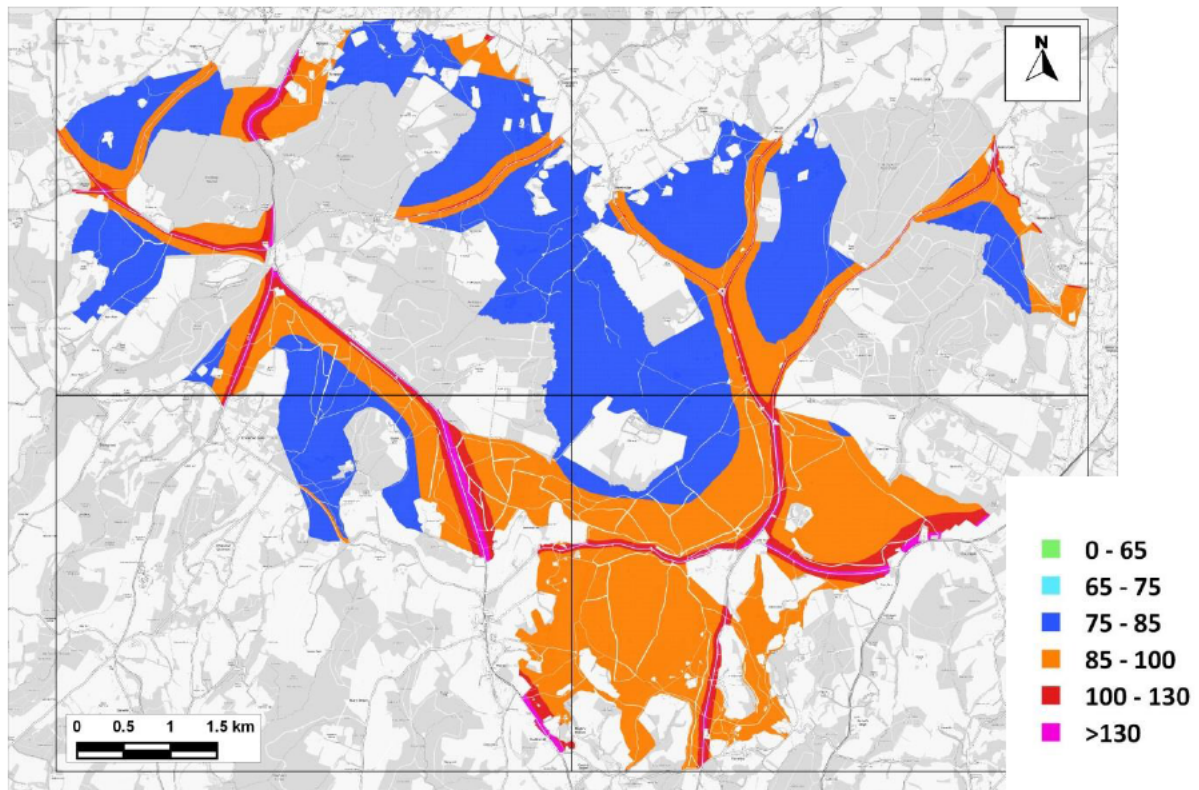
Figure 11.2: Predicted Maximum 24-hour Mean NO x Concentrations across the SAC – 2028 No WDC-Growth - A ( \mu\text{g}/\text{m}^3 )
