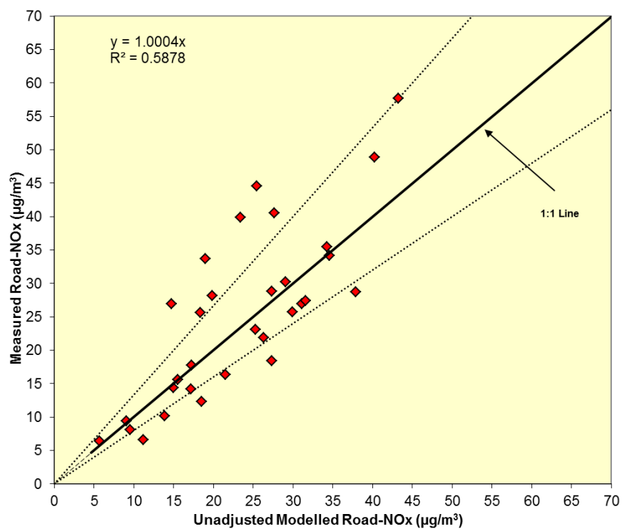
Figure 5.8: Modelled vs Measured Annual Mean Road-NOx, Link Set 1, Iteration 2
