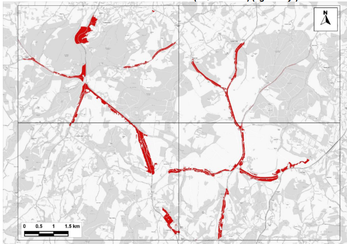
Figure 14.18: Areas in SAC Predicted to Experience an Increase in Nitrogen Deposition Greater than 1% of the 10 kg-N/ha/yr Critical Load where this Critical Load would also be Exceeded - Comparing 'With Plan' to 'No Growth' Scenarios under Emissions Scenario B (AQC Method)
