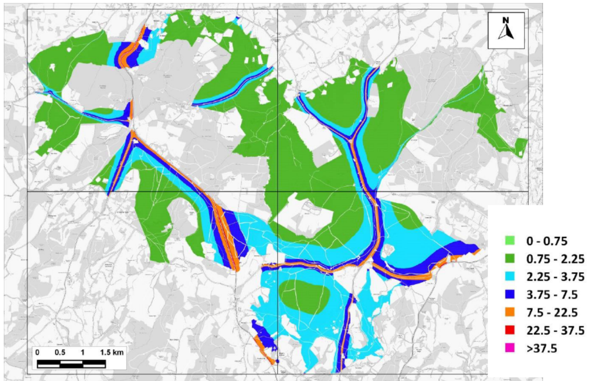
Figure 14.3: Change in Maximum Predicted 24-hour Mean NO x Comparing 'With Plan' to 'No Growth' under Emissions Scenario A ( \mu\text{g}/\text{m}^3 )
