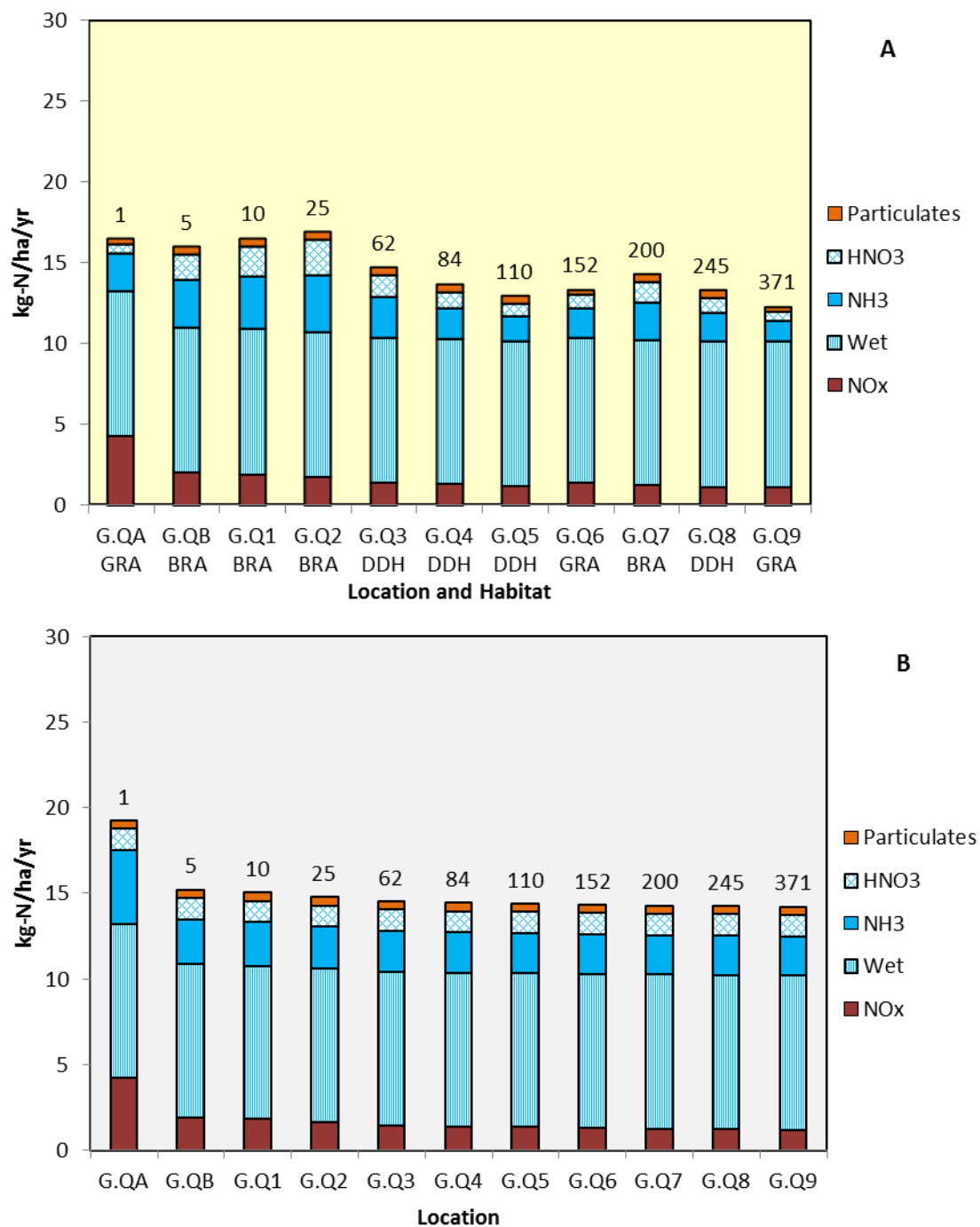
Figure 9.37: Deposition to Ecological Transect G – AQC Method – (A) Using Current Habitat Types and (B) If all Habitat were Heath (approximate distance from the nearest main road to each quadrant to shown numerically above each column) 36
